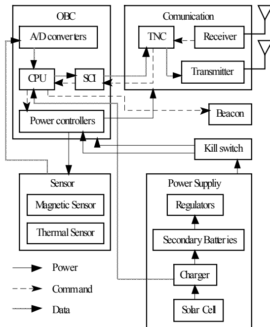
Figure 4. System Block
