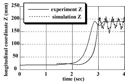
Figure 9. Tip coordinate (longitudinal direction)
