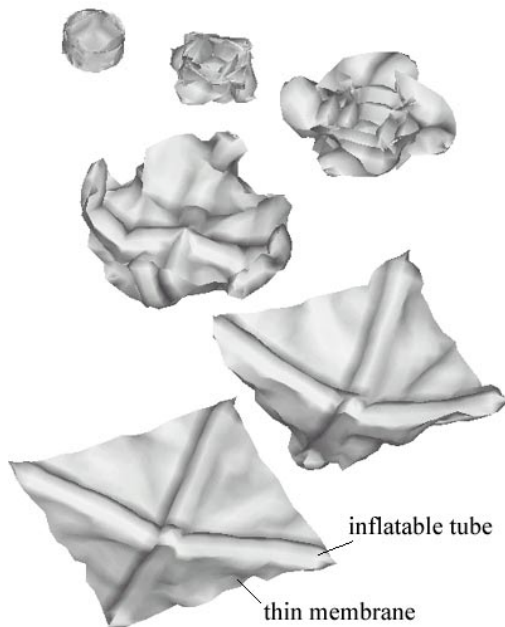
Figure 6. Membrane supported by four tubes
