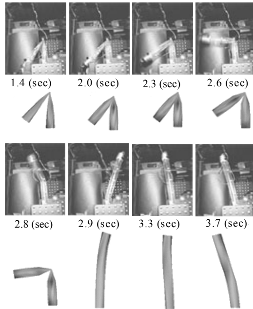
Figure 7. Deployment of a tube under micro-gravity
