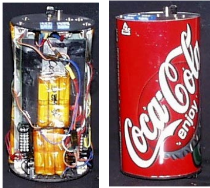
Figure 1. Cansat inside and outside view
