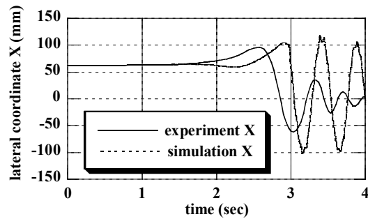
Figure 8. Tip coordinate (lateral direction)
