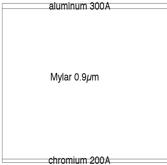
Figure 3-12 Sail Substrate and Metallization
