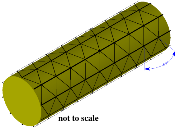
Figure 3-9 Sub-Tg Composite Isogrid Boom
