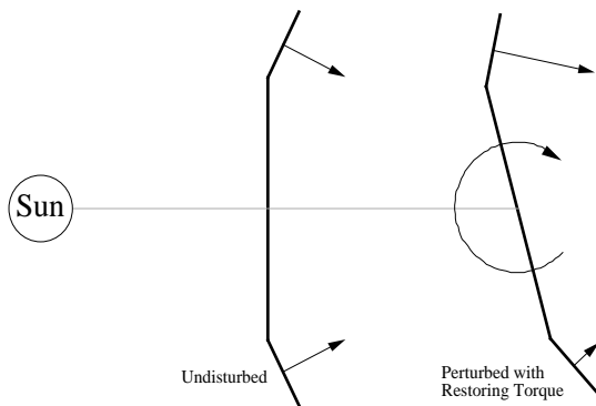
Figure 3-16 Sailcraft Pitch and Roll Passive Stabilization Technique
