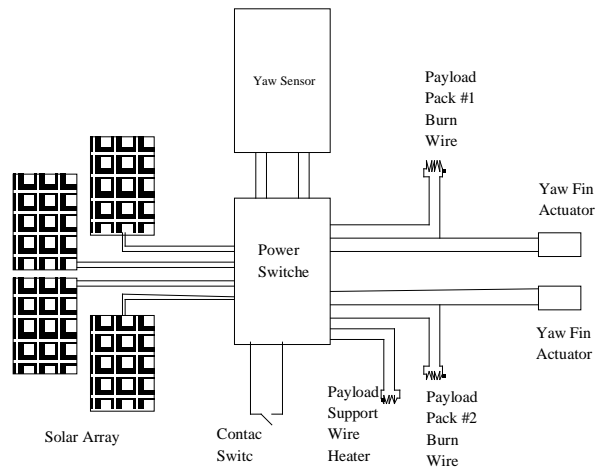
Figure 3-17 Yaw Control System Schematic
