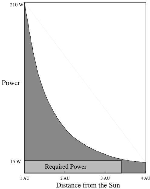
Figure 3-18 Sailcraft Power Profile
