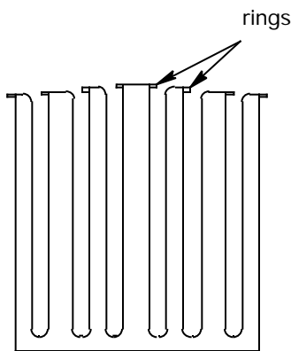
Figure 3-10 Boom Telescopic Packaging
