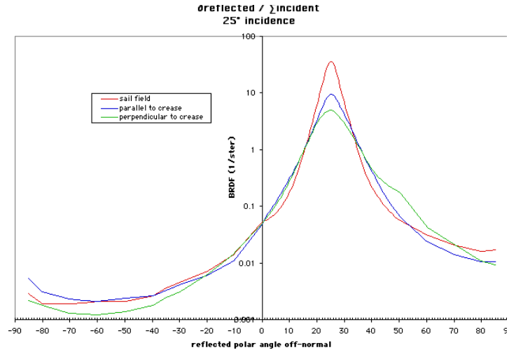
Figure 3-14 Scattering Data and Symmetry Model
