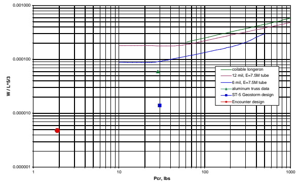
Figure 3-11 Boom Structural Efficiency
