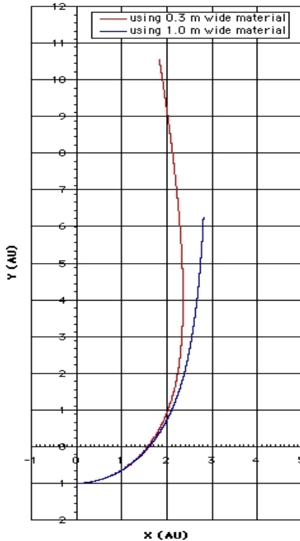
Figure 3-6 Sailcraft Trajectories
