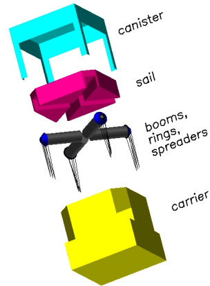
Figure 3-5 Packaged Sailcraft
