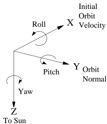
Figure 3-15 Sailcraft Reference Coordinates
