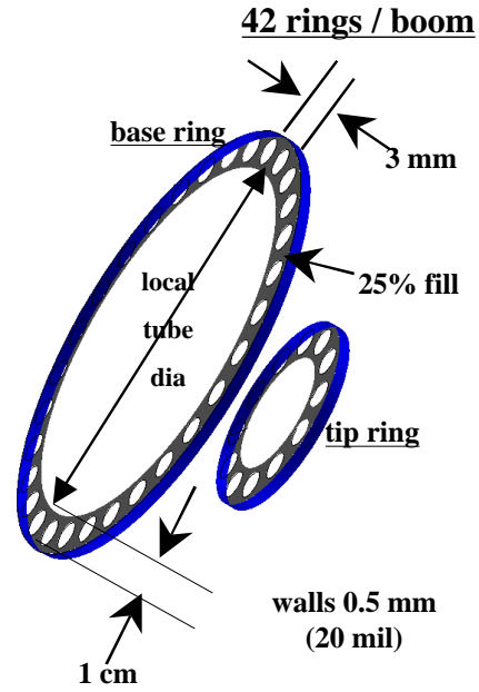
Figure 3-8B Spreaders and Rings
