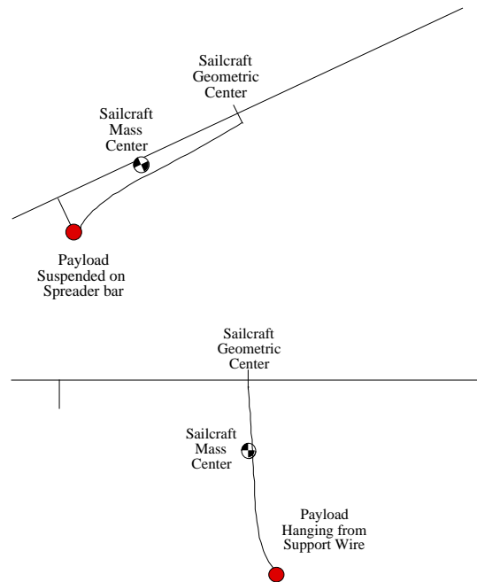
Figure 3-19 Sailcraft Pitch Control Technique
