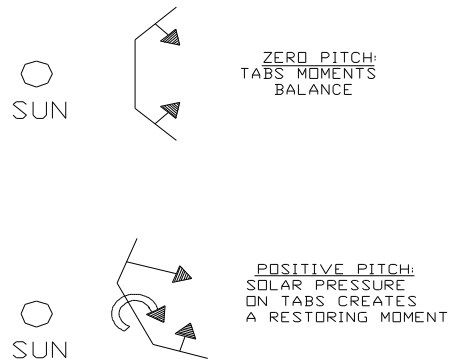
Figure 3-7 Passive Stabilization
