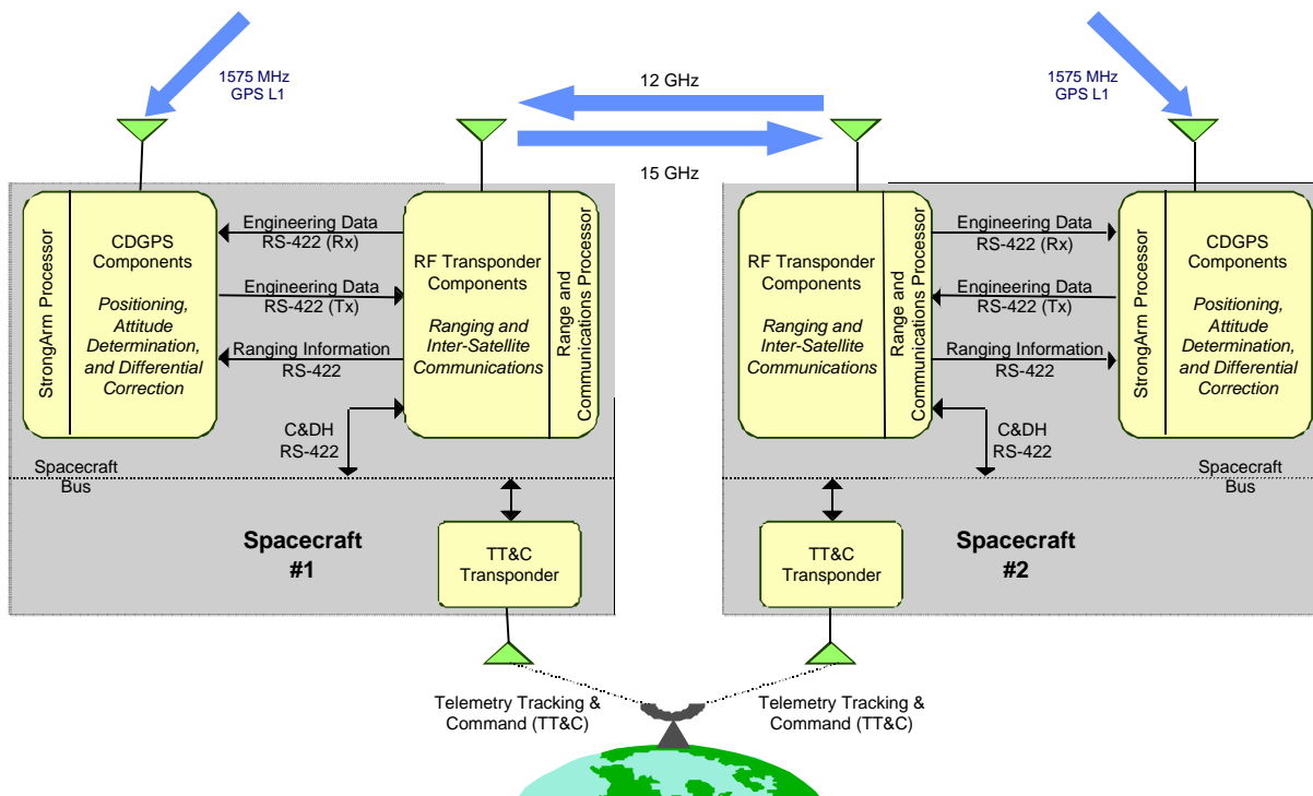
Figure 1. Star Ranger Conceptual Diagram
