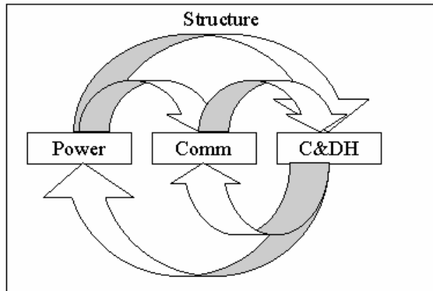
Figure 3. Architecture diagram
