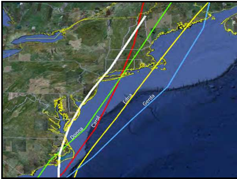
Fig. 7. Reconstructed track of the 1821 New England Hurricane (thick white line) and similar track hurricanes used for the synoptic environment composite analysis (Hurricanes Carol (1954); Edna (1954); Donna (1960); and Gerda (1969)).
