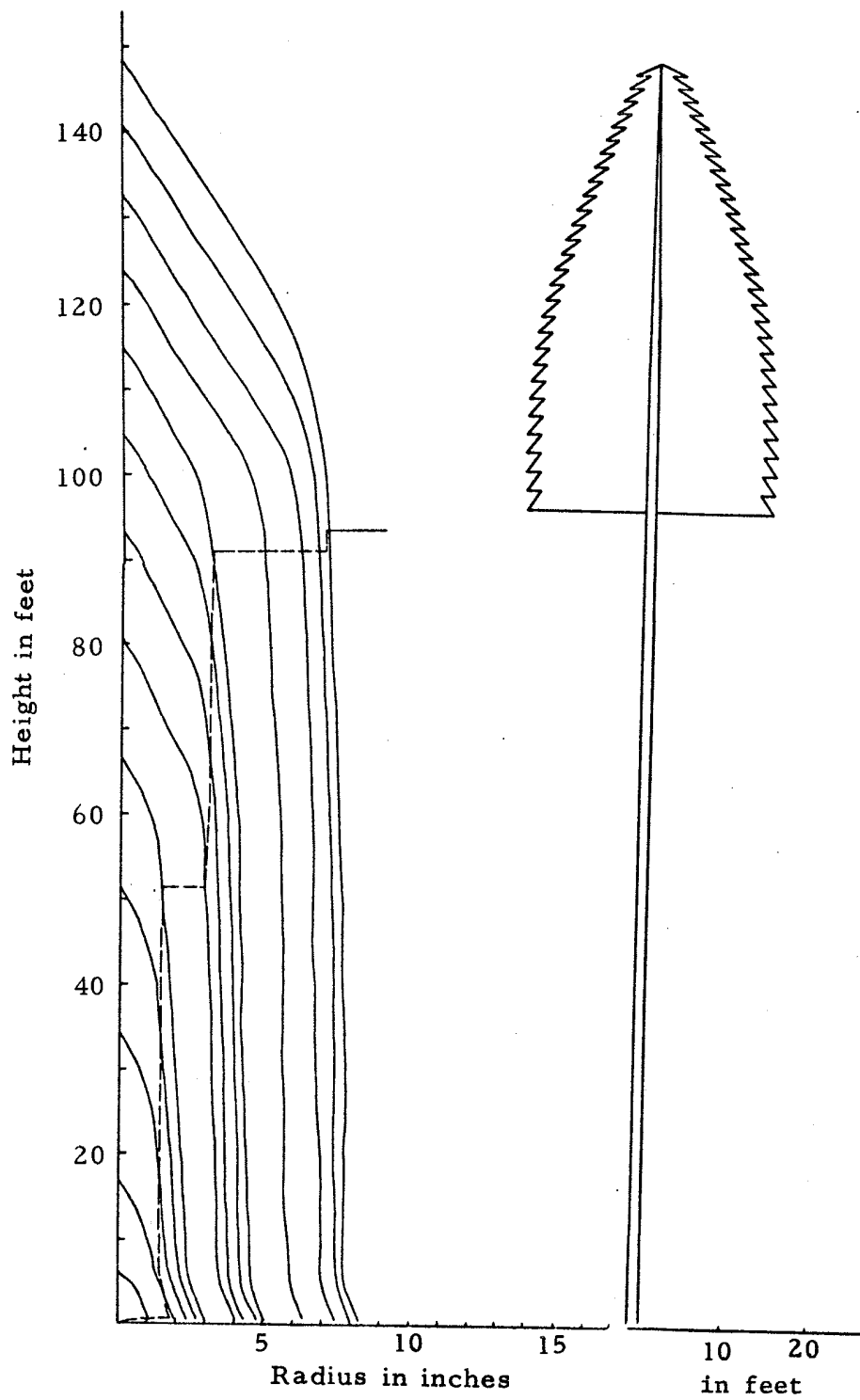
Figure 14. Simulated stem profile at 60 years showing 5 year increments. Initially 681 trees per acre, thinned at 20 and 40 years.
