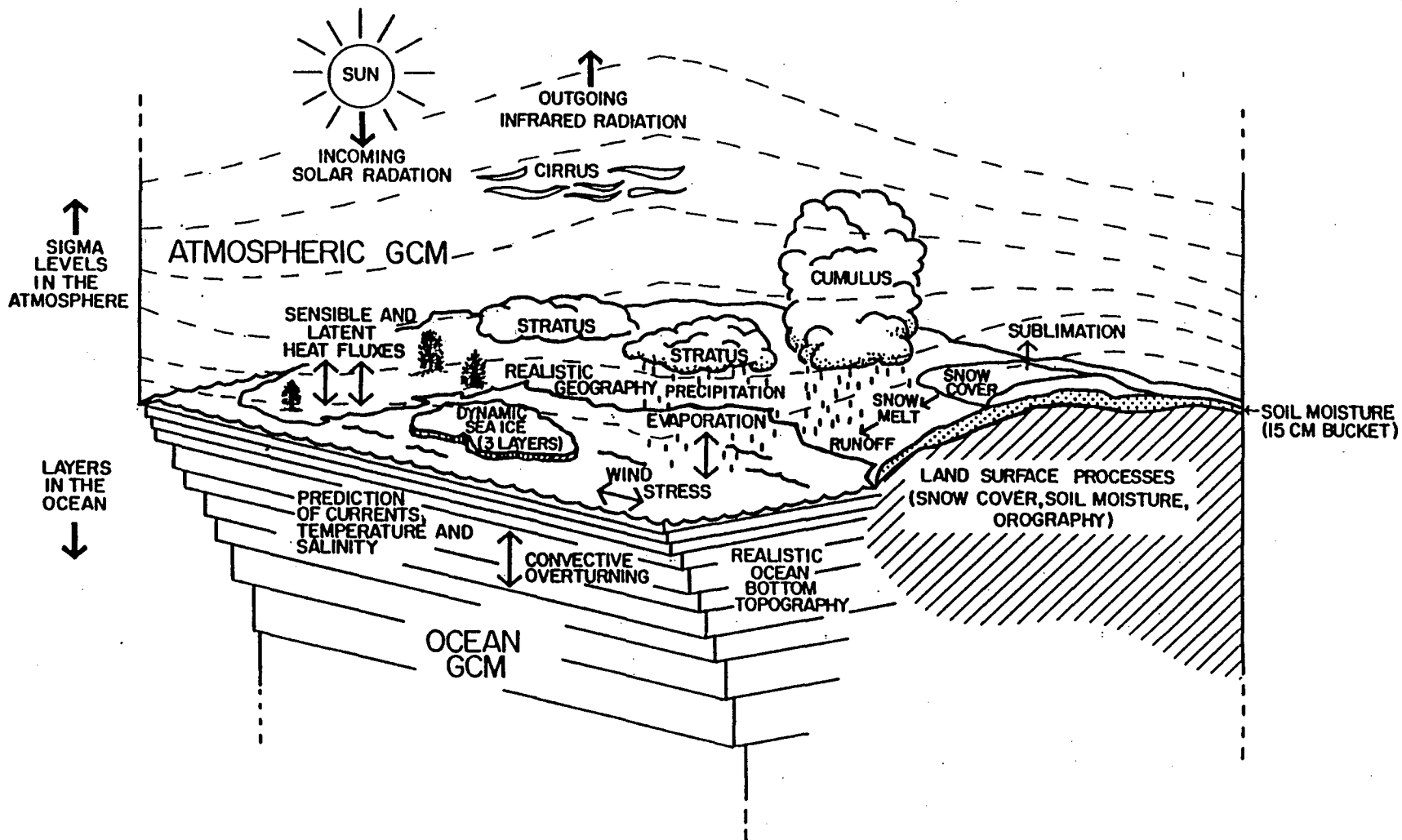
Figure 14.—Schematic of climate model.
