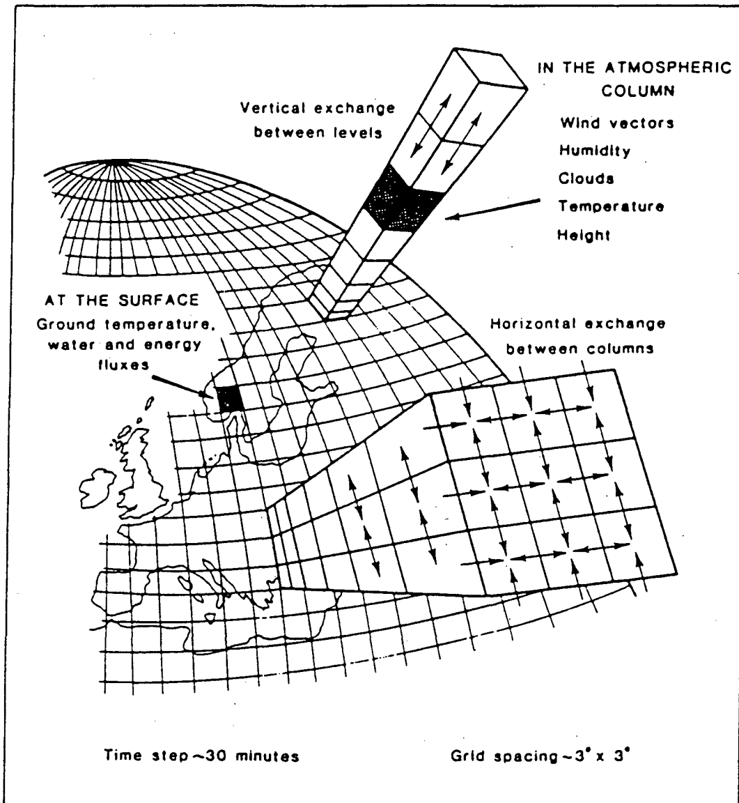
Figure 13.—The structure of an atmospheric GCM.
