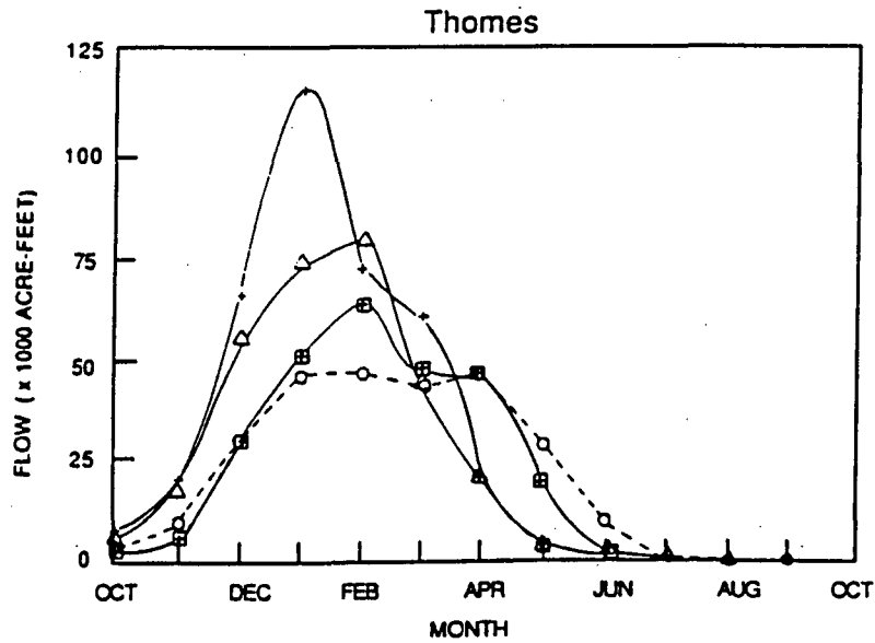
Figure 20.—Study catchment monthly mean streamflow for base case and CO 2 doubling scenarios A1-A3.
