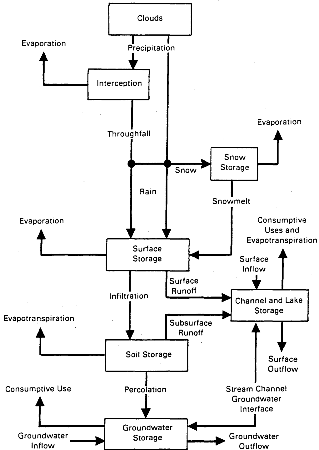
Figure 15.—Schematic diagram of the hydrologic system of a drainage basin.
