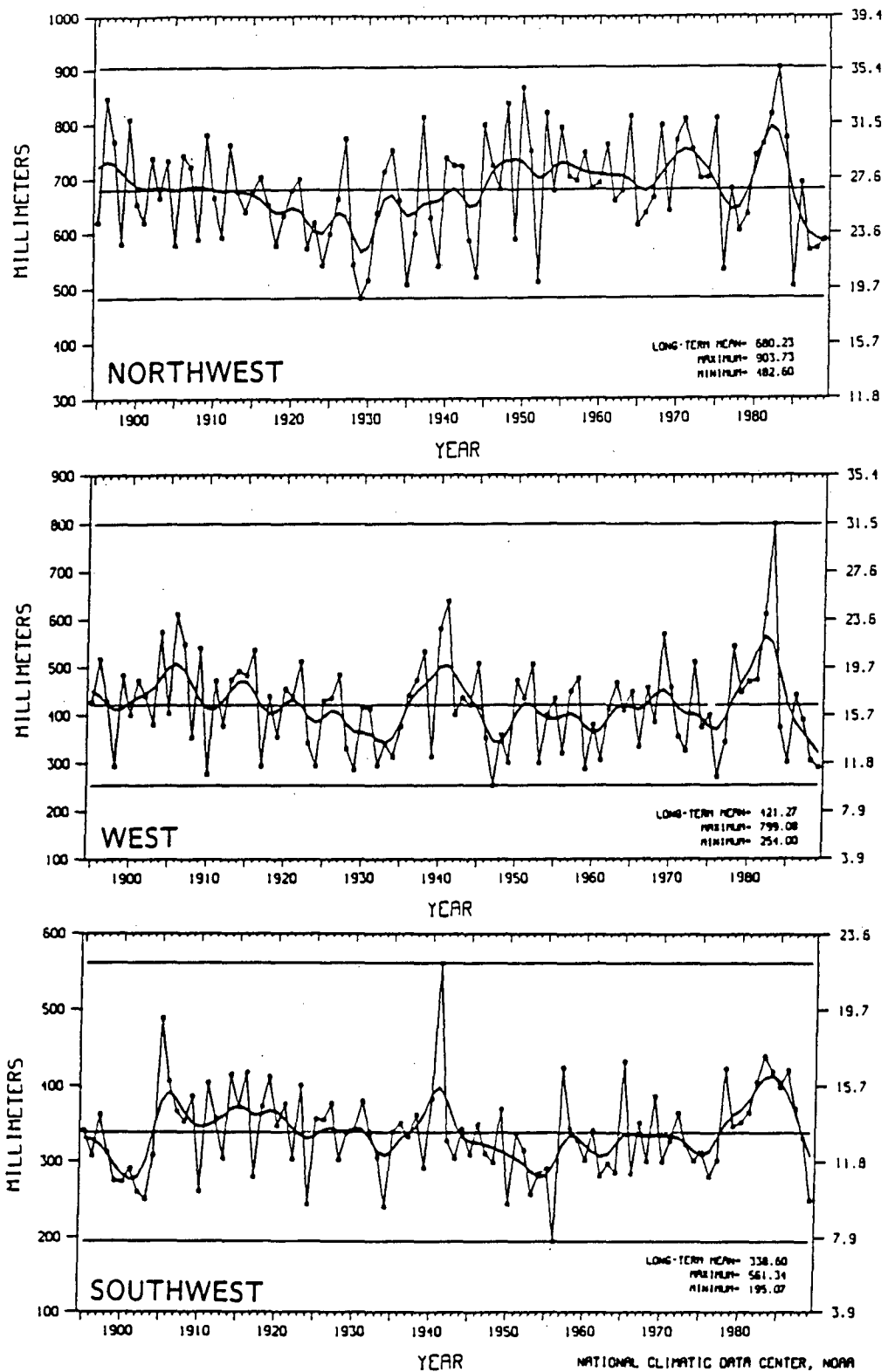
Figure 5.—Time series of annual mean precipitation amounts in the Northwest, West, and Southwest regions in millimeters (left) and inches (right). The long-term mean and extremes are given at the lower right, and lines are plotted for each. A low pass smoother shows interdecadal fluctuations.
