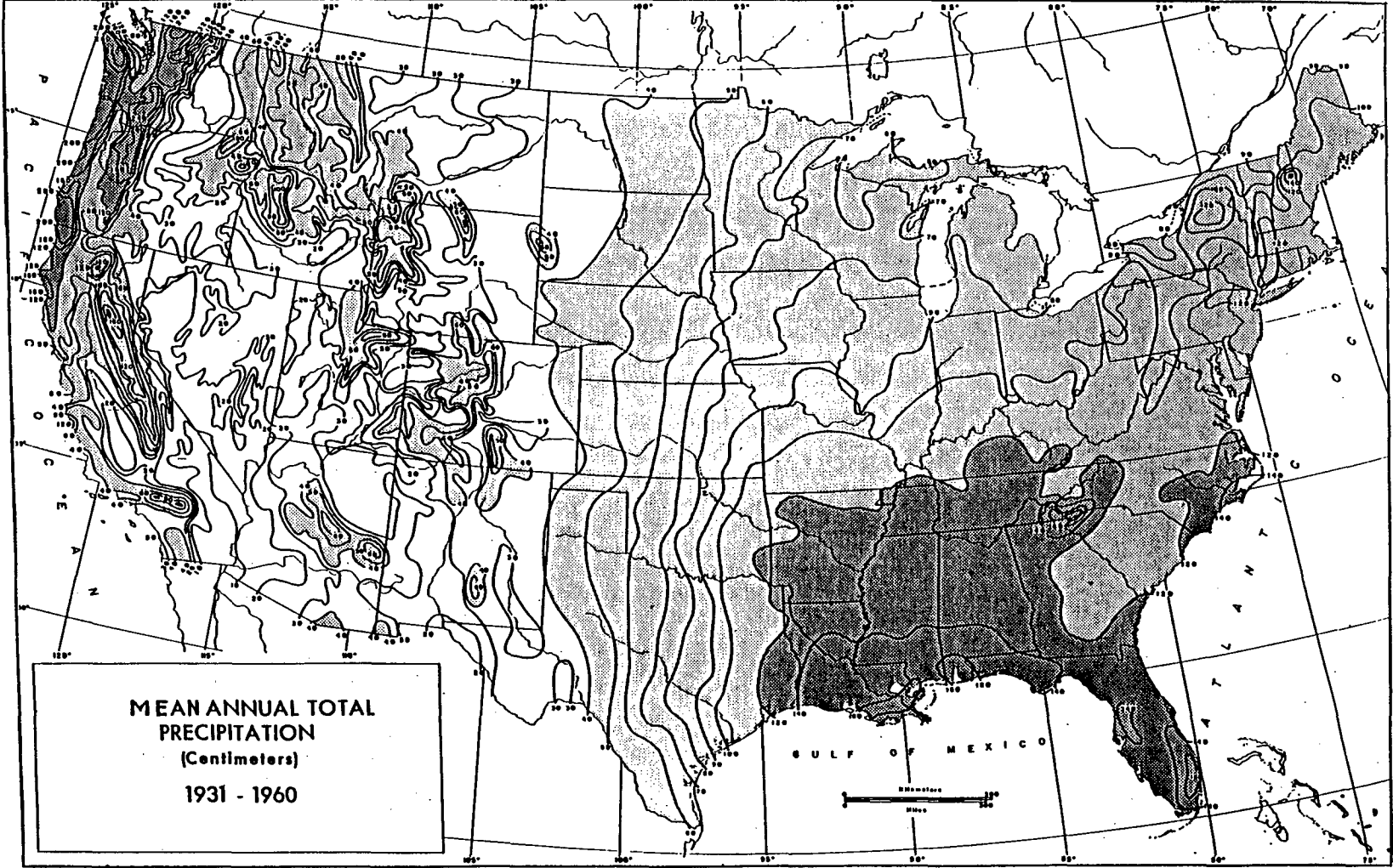
Figure 3.—Mean annual total precipitation, based on all available stations adjusted to standard period 1931-1960 (after U.S. Weather Bureau).
