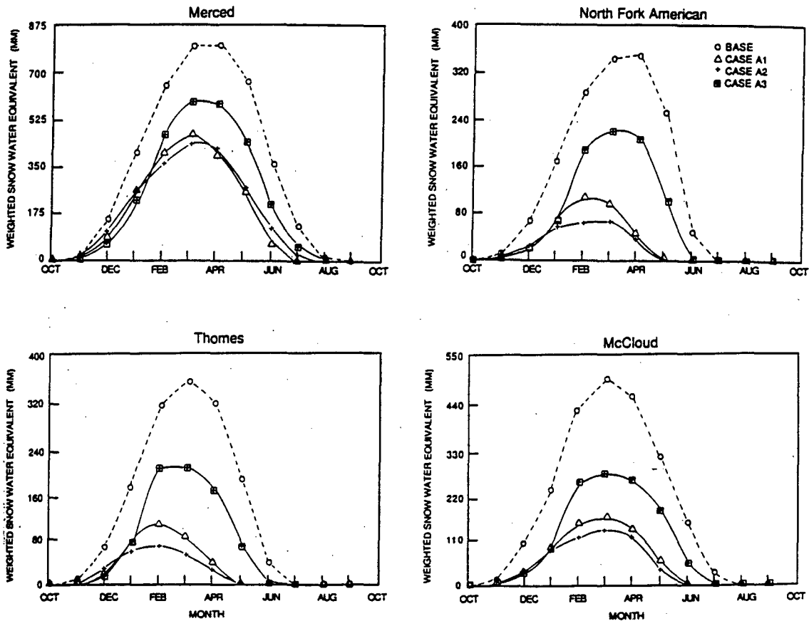
Figure 19.—Study catchment mean weighted snow water equivalent for base case and CO 2 doubling scenarios A1-A3.
