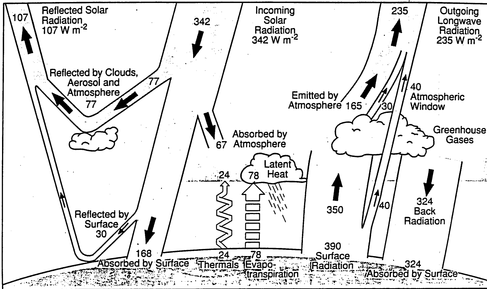
Figure 11.—The Earth's radiation and energy balance. The net incoming solar radiation of 342 Wm -2 is partially reflected by clouds at the atmosphere, or at the surface, but 49 percent is absorbed by the surface. Some of that heat is returned to the atmosphere as sensible heating and most as evapotranspiration that is realized as latent heat in precipitation. The rest is radiated as thermal infrared radiation, and most of that is absorbed by the atmosphere which, in turn, emits radiation both up and down, producing a greenhouse effect, as the radiation lost to space comes from cloud tops and parts of the atmosphere much colder than the surface. The partitioning of the annual global mean energy budget and the accuracy of the values are given in Kiehl and Trenberth (1997).
