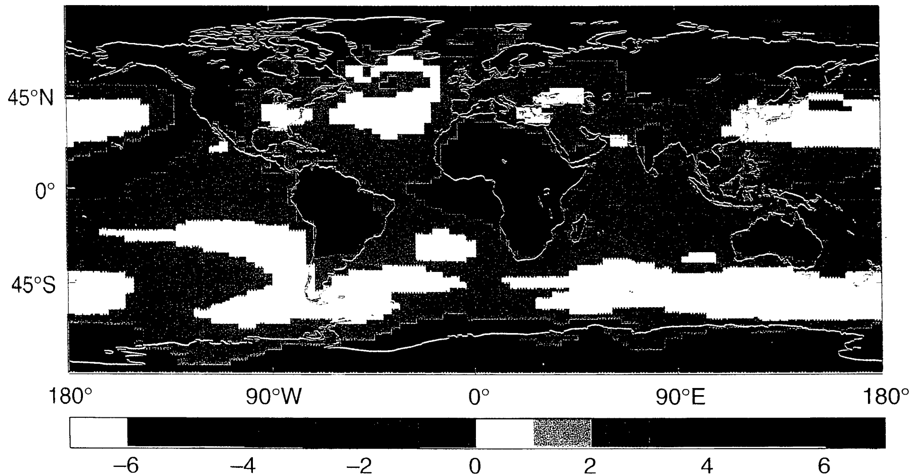
Figure 9.—The pattern of surface temperature change projected by a transient coupled model at the time of CO 2 doubling when both CO 2 and aerosol concentration increases are taken into account.
