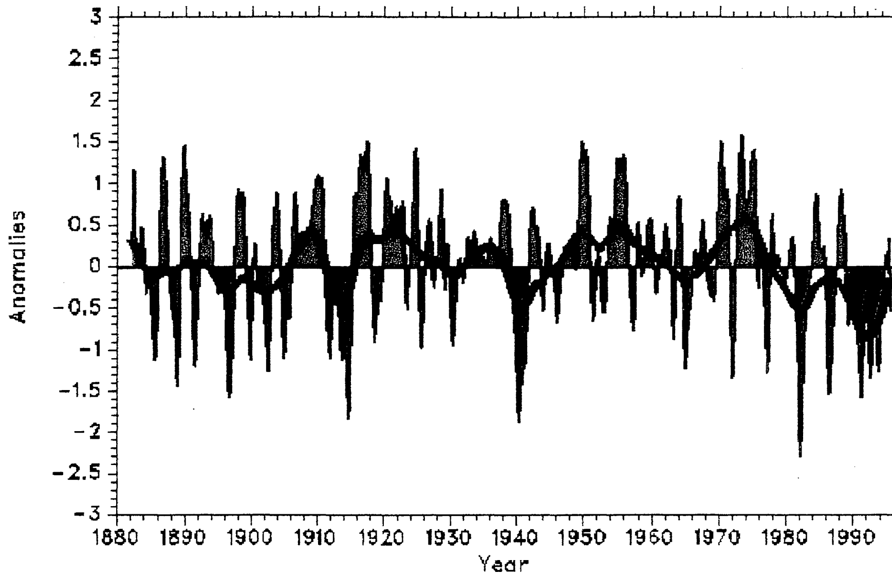
Figure 7.—Darwin Southern Oscillation Index.
