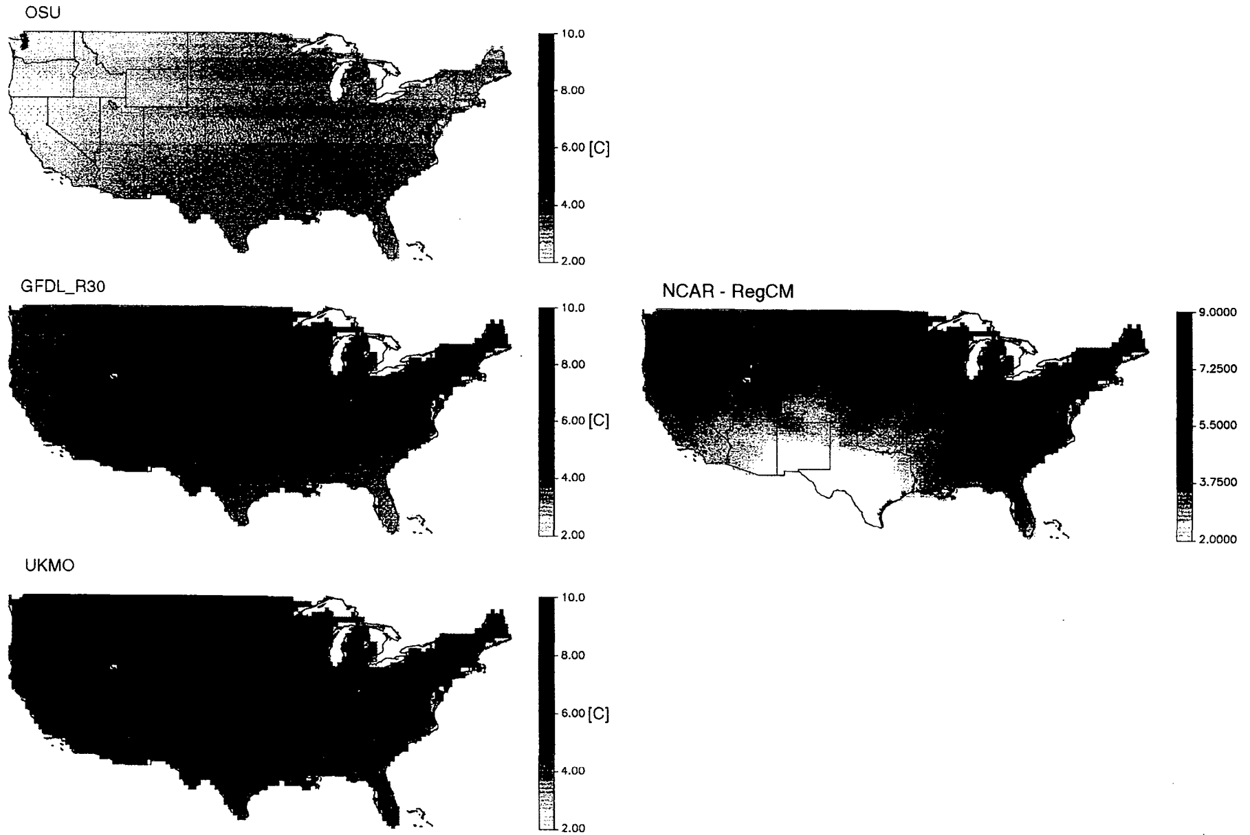
Figure 17.—Climate scenario—annual temperature change difference.
