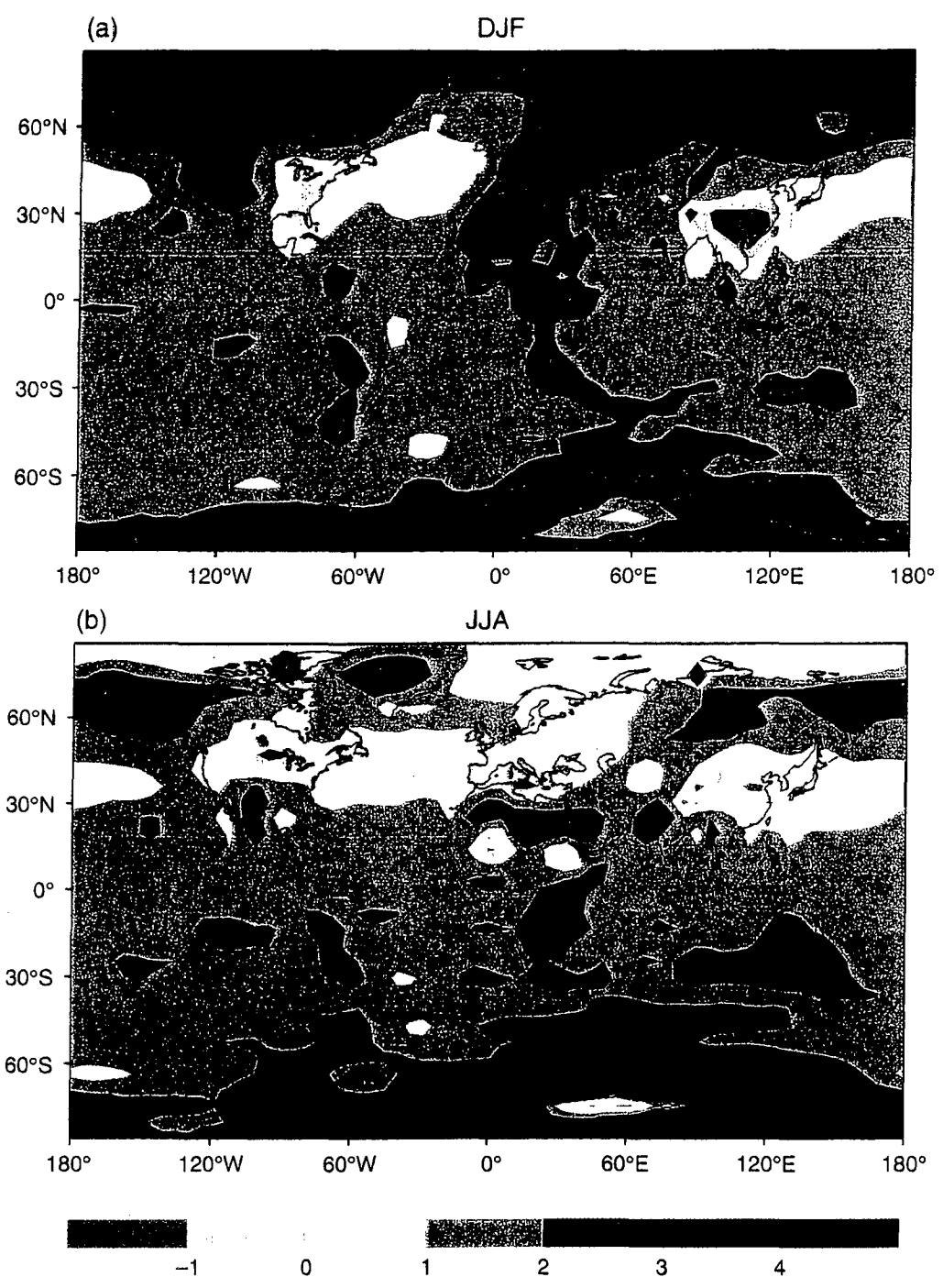
Figure 12.—Seasonal change in surface temperature from 1880-1889 to 2040-2049 in simulations with aerosol effects included from IPCC. Contours every 1 °C. (a) December to February; (b) June to August.
