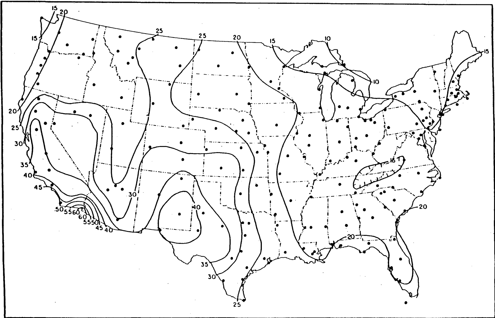
Figure 4.—Coefficient of variation (%) of annual precipitation, 1931-1960, at 220 first-order stations. Station locations indicated by dots.
