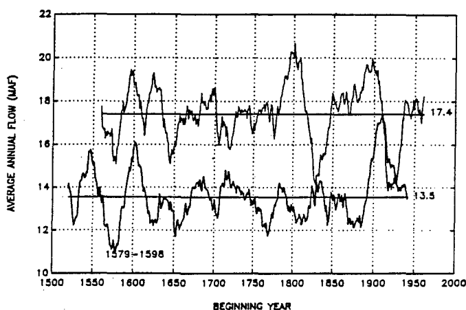
Figure 6.—Time series plots of 20-year running means of reconstructed flows for the Colorado River at Lee's Ferry (lower line) and for the Four Rivers Index, northern California (upper line).
