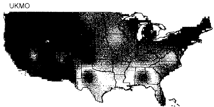
Figure 18.—VEMAP climate scenarios—annual precipitation change ratio.
