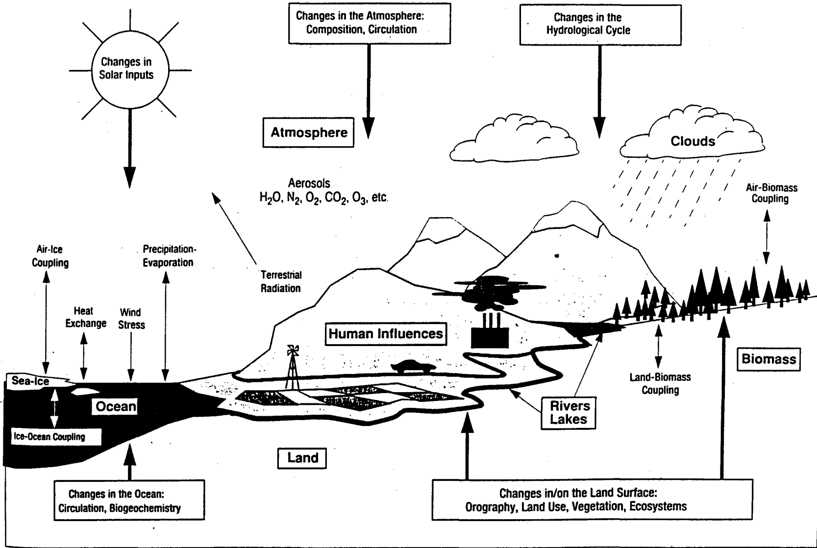
Figure 10.—Schematic view of the components of the global climate system (bold), their processes and interactions (thin arrows), and some aspects that may change (bold arrows).
