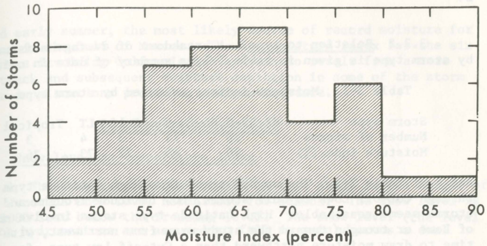
Figure 3-3. Frequency distribution of moisture indices in 42 qualifying storms.
