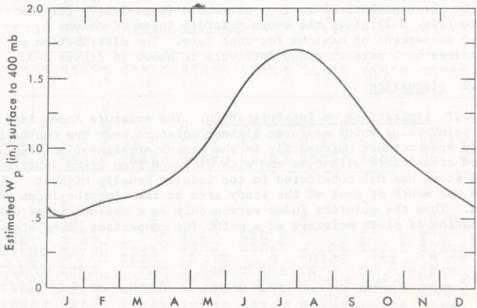
Figure 3-2. Seasonal variation of precipitable water (in.) at Grand Junction, surface to 400-mb, based on maximum persisting 12-hour 1000-mb dew points from reference 10.
