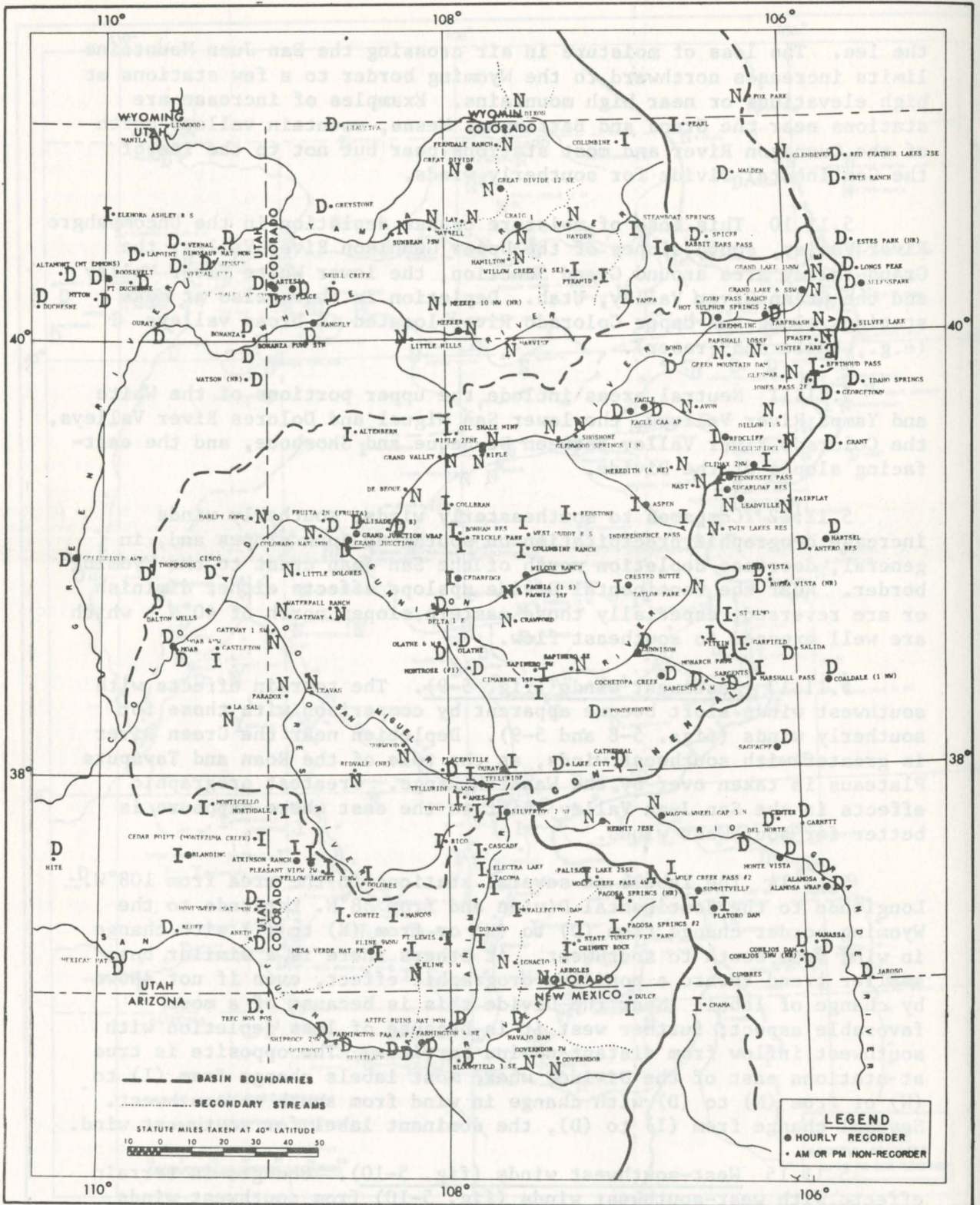
Figure 5-9. Local terrain effects on precipitation for southwesterly 500-mb winds. Letters indicate effects, observed in storms or estimated, to be deletion (D), no effect (N), or increase (I).
