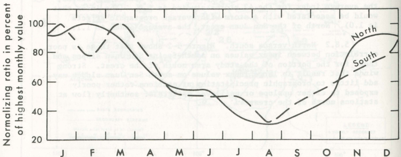
Figure 5-4. Monthly normalizing ratio (Rn) north (—) and south (---) of the San Juan crest, as percent of highest monthly value.
