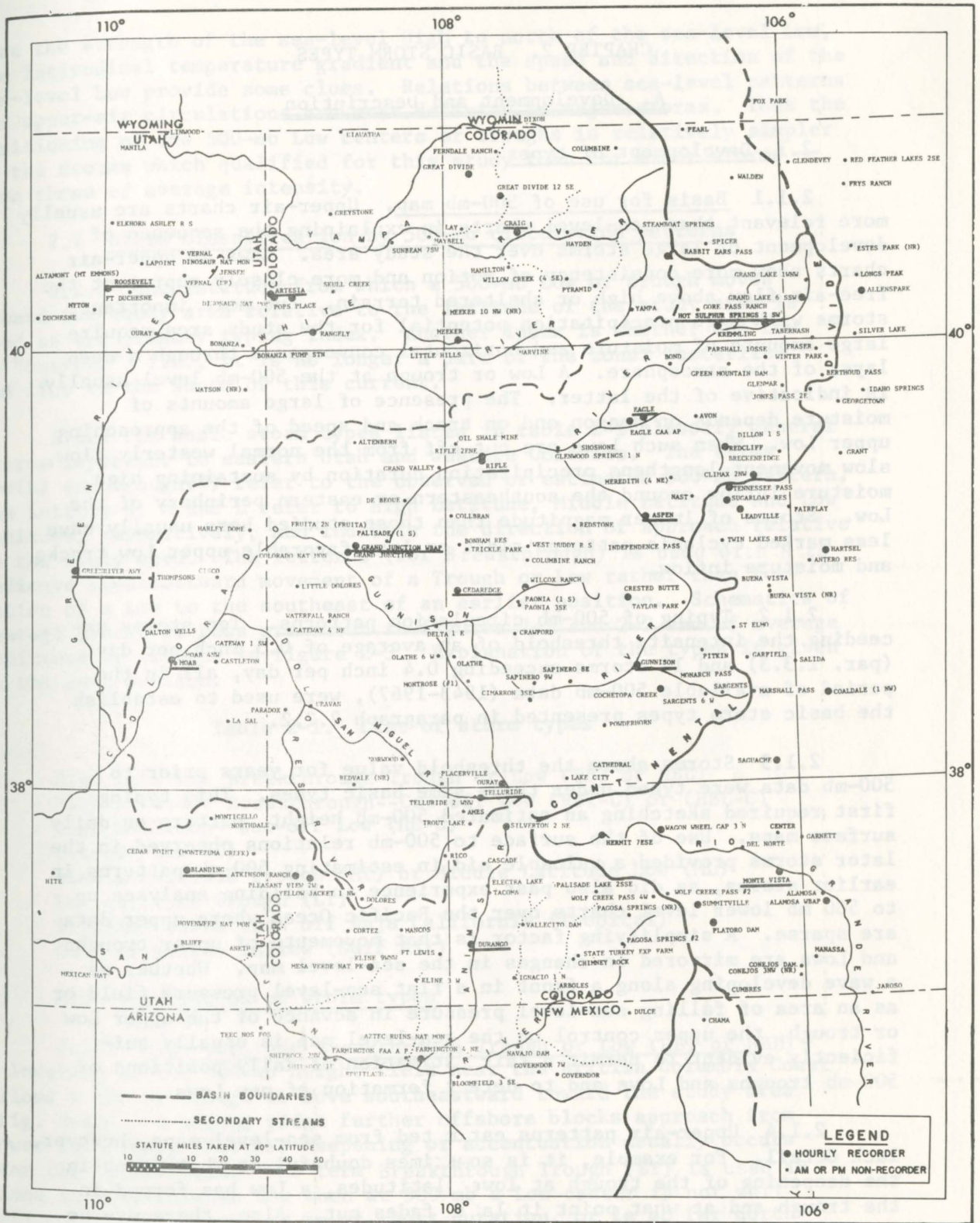
Figure 1-3. Map of precipitation stations in the study area for the period 1933 to 1966. (Key stations for selection of qualifying storms are underlined.)
