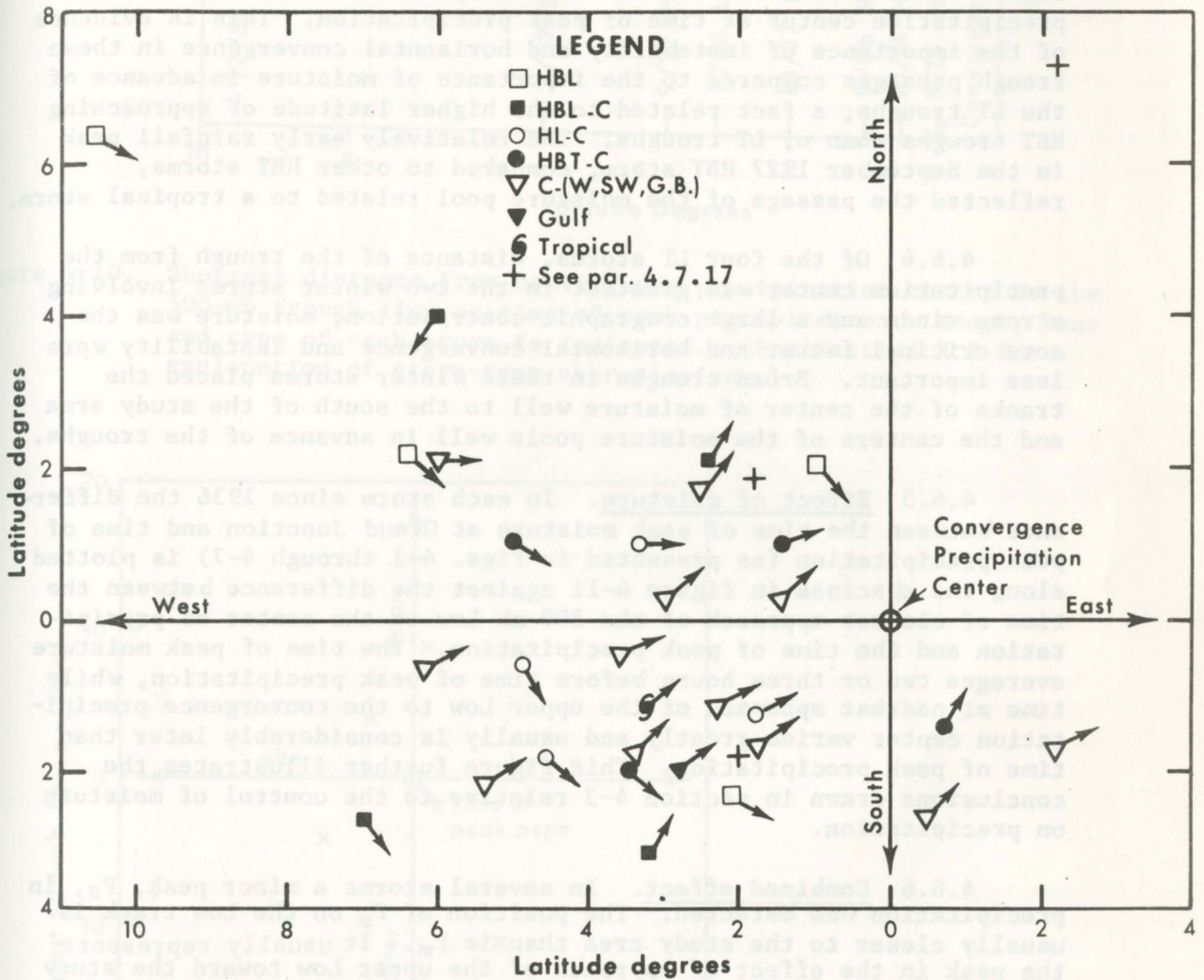
Figure 4-9. Positions of 500-mb Lows relative to convergence precipitation centers at time of peak precipitation. Arrows are parallel to tracks of Lows. (See Section 2.3 for explanation of storm-type abbreviations.)
