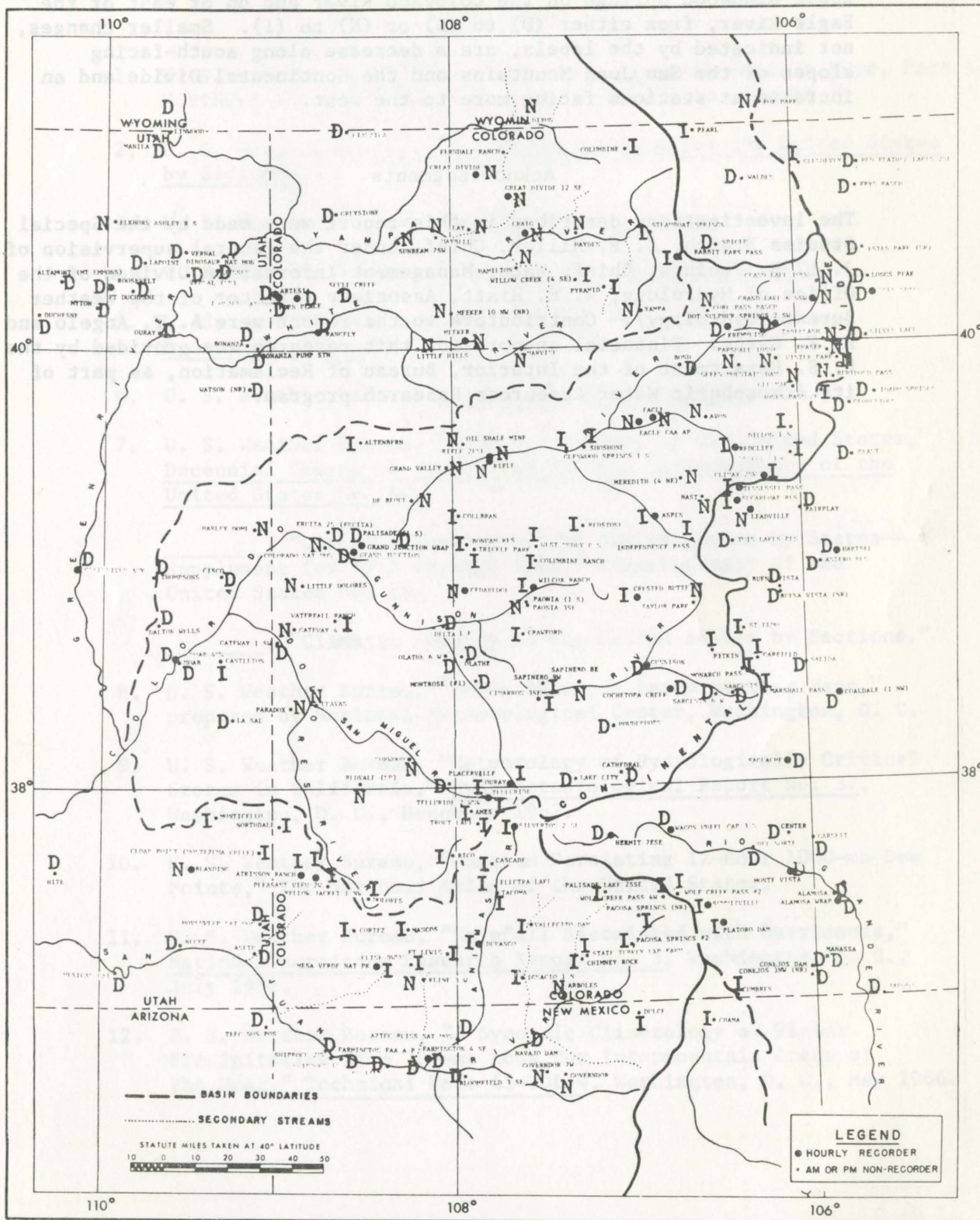
Figure 5-10. Local terrain effects on precipitation for west-southwesterly 500-mb winds. Letters indicate effects, observed in storms or estimated, to be depletion (D), no effect (N), or increase (I).
