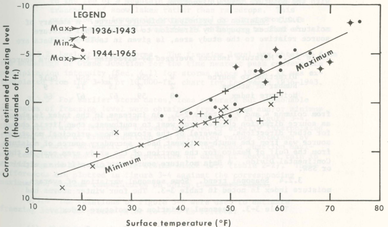
Figure 3-4. Correction to apply to storm freezing level estimated from Grand Junction maximum or minimum temperatures, assuming a moist adiabatic lapse rate. (Based on the freezing level at Grand Junction interpolated from 700-mb analysis in storms 1936-1943 and observed in storms 1944-1965. Storms used are listed in table 2-2.)
