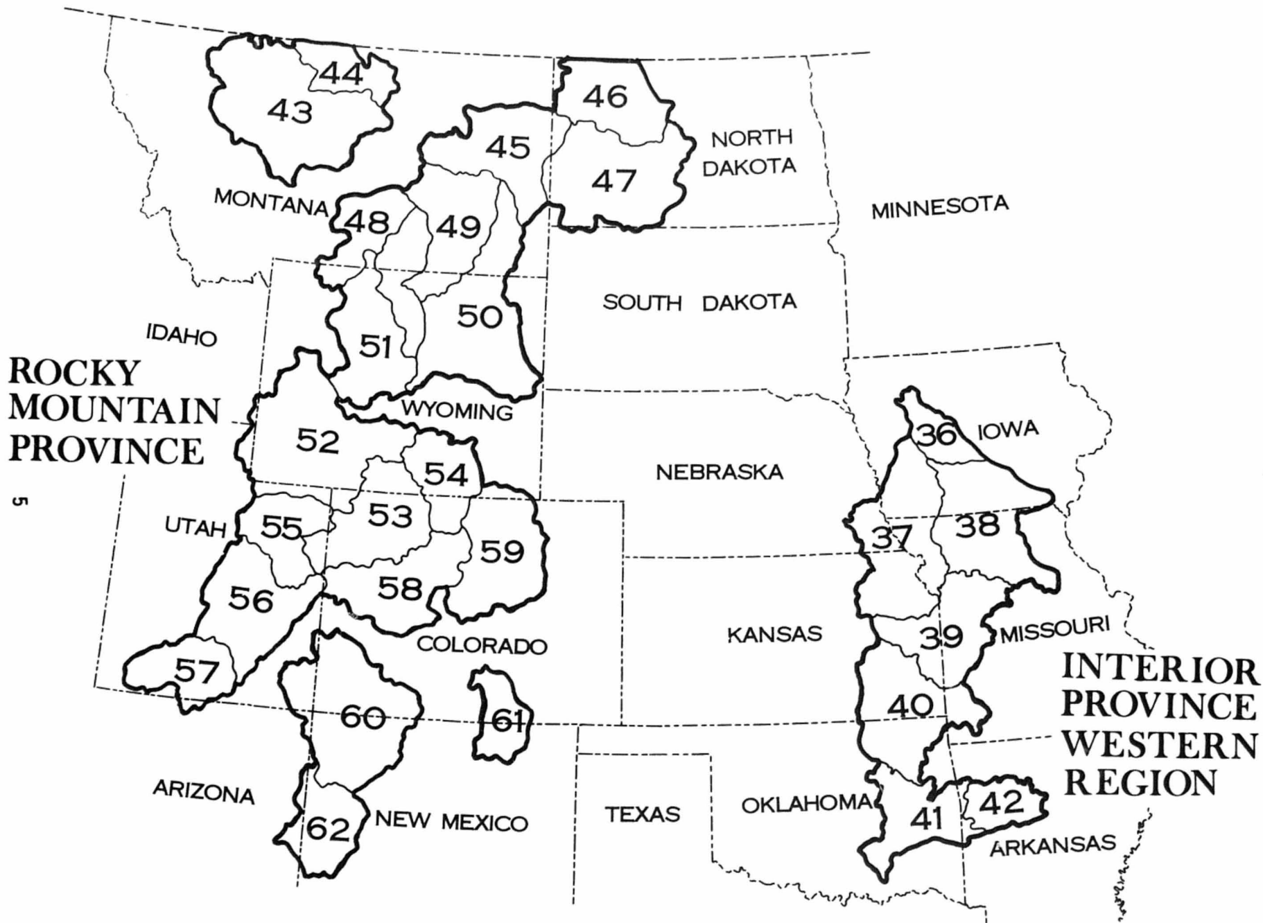
Figure 2b.--U. S. Geological Survey coal areas in the Rocky Mountain and Western Interior Coal Provinces.
