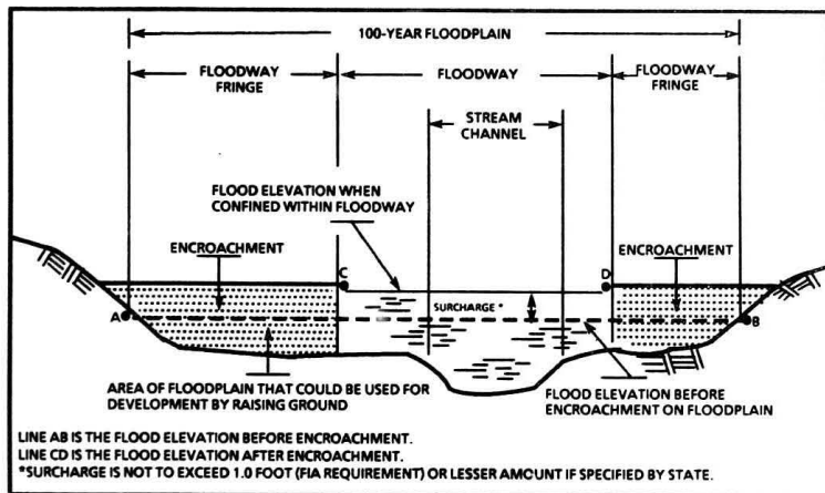
Figure 1. Floodway Schematic
