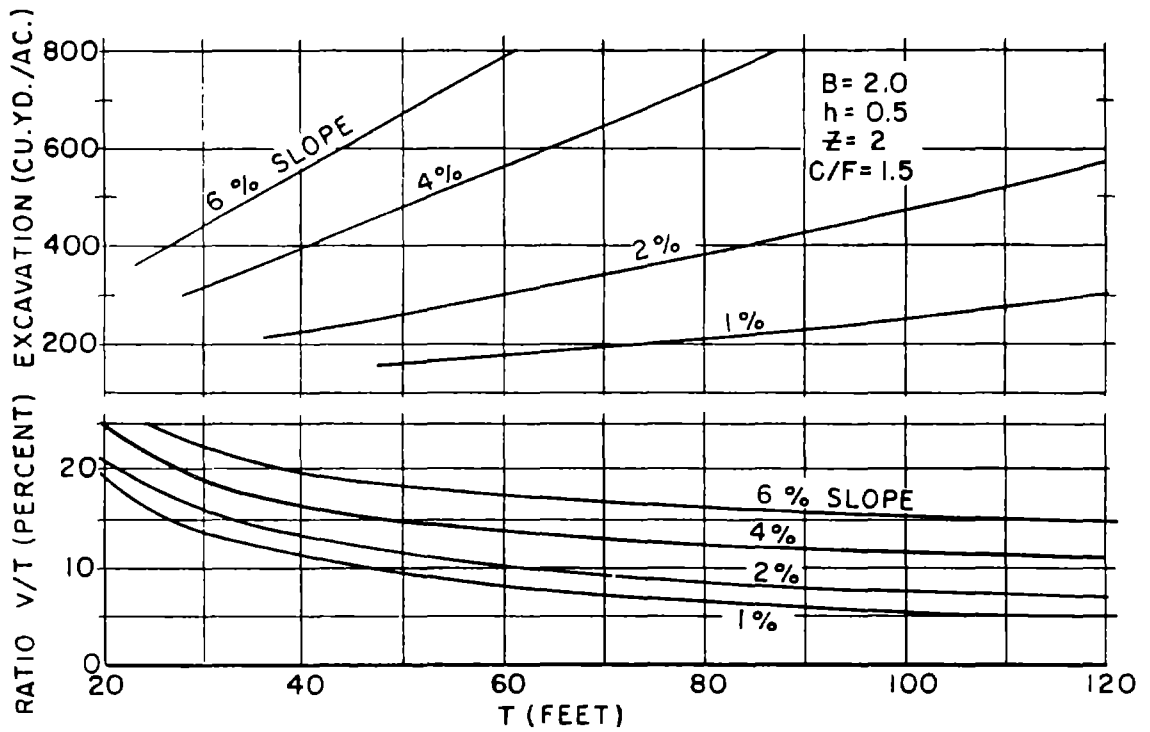
Figure 12-12.--Contour-bench relationships.
