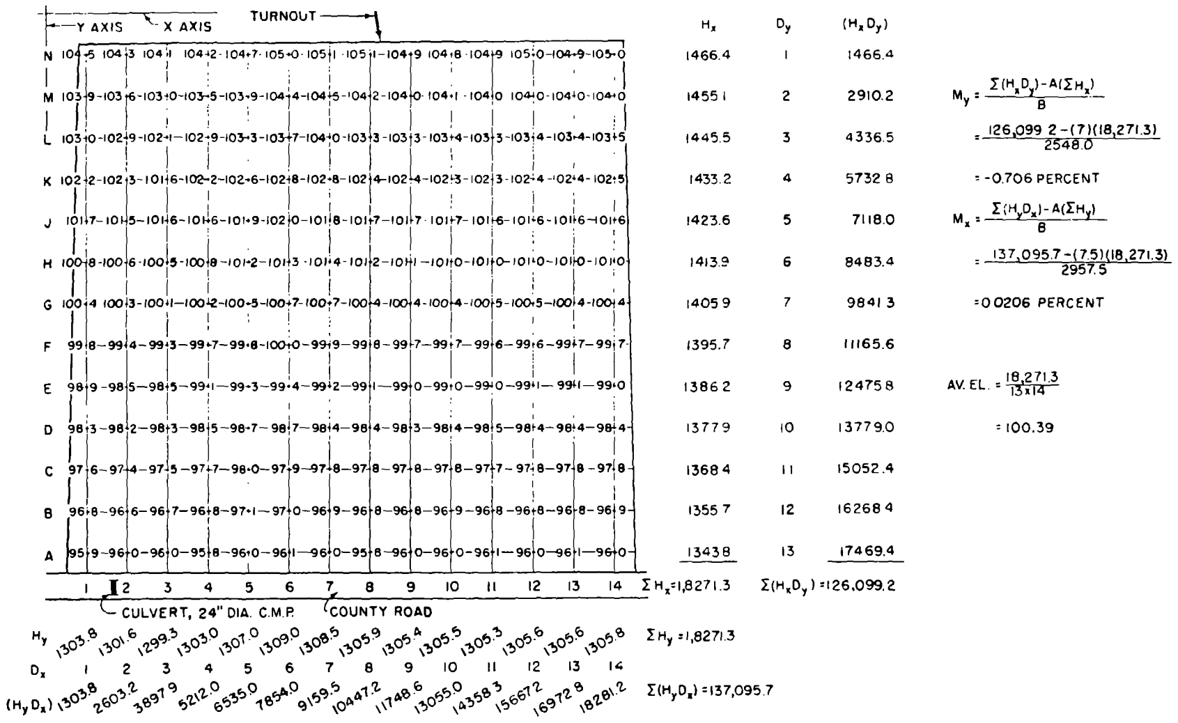
Figure 12-4.--Determination of plane of best fit.
