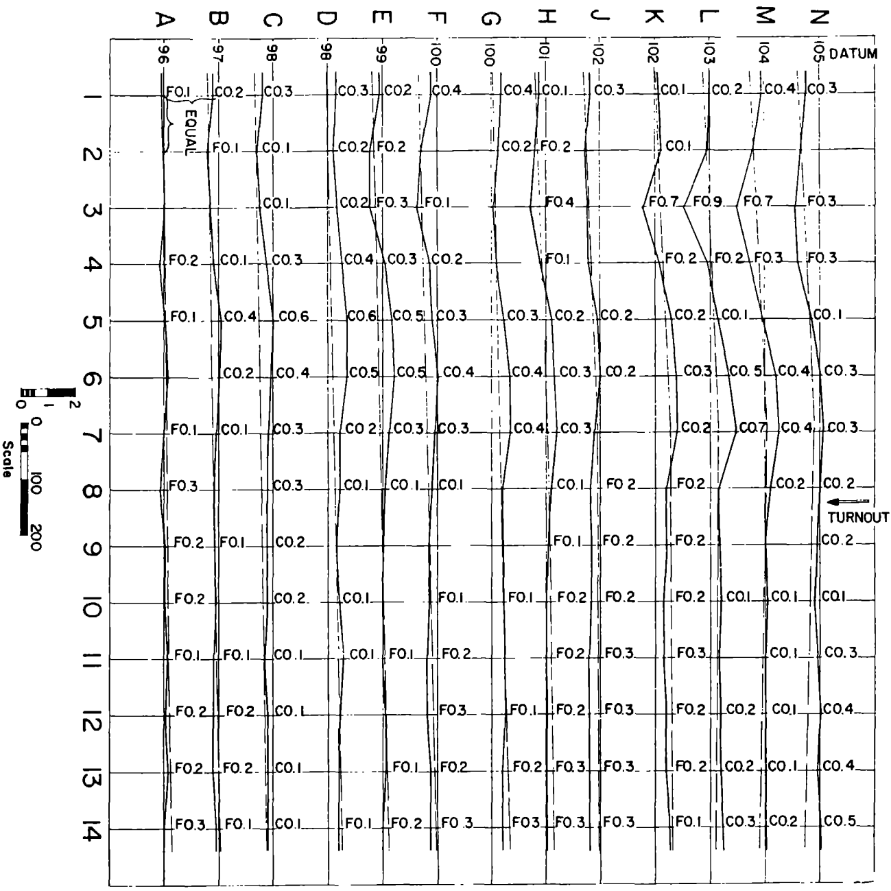
Figure 12-6.—The profile method of land leveling.
