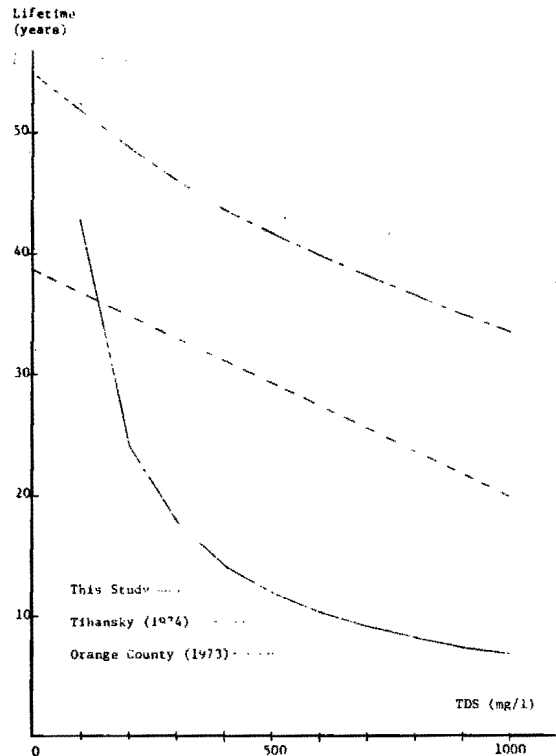
Figure E-4. Graphical comparison of estimated lifetime relationships for galvanized wastewater pipes.
