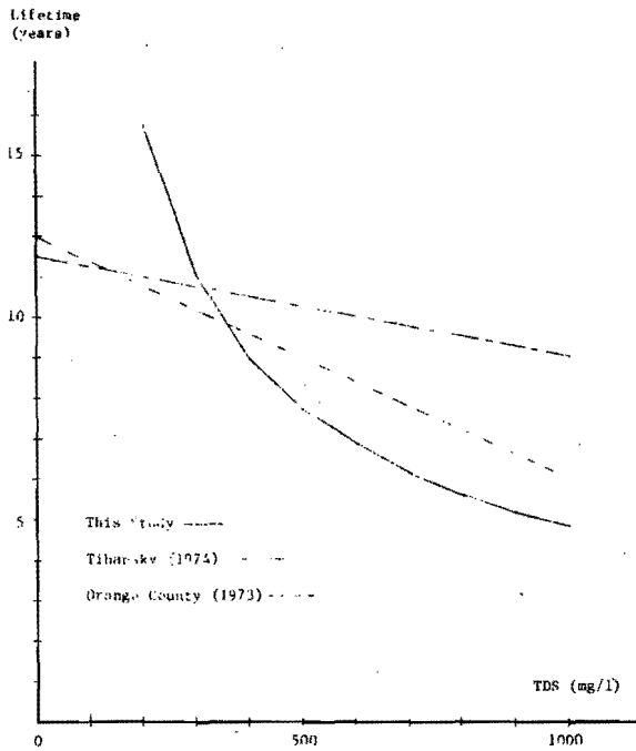
Figure E-5. Graphical comparison of estimated lifetime relationships for brass faucets.
