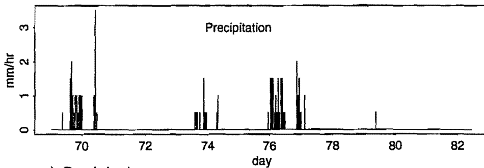
c) Precipitation.
