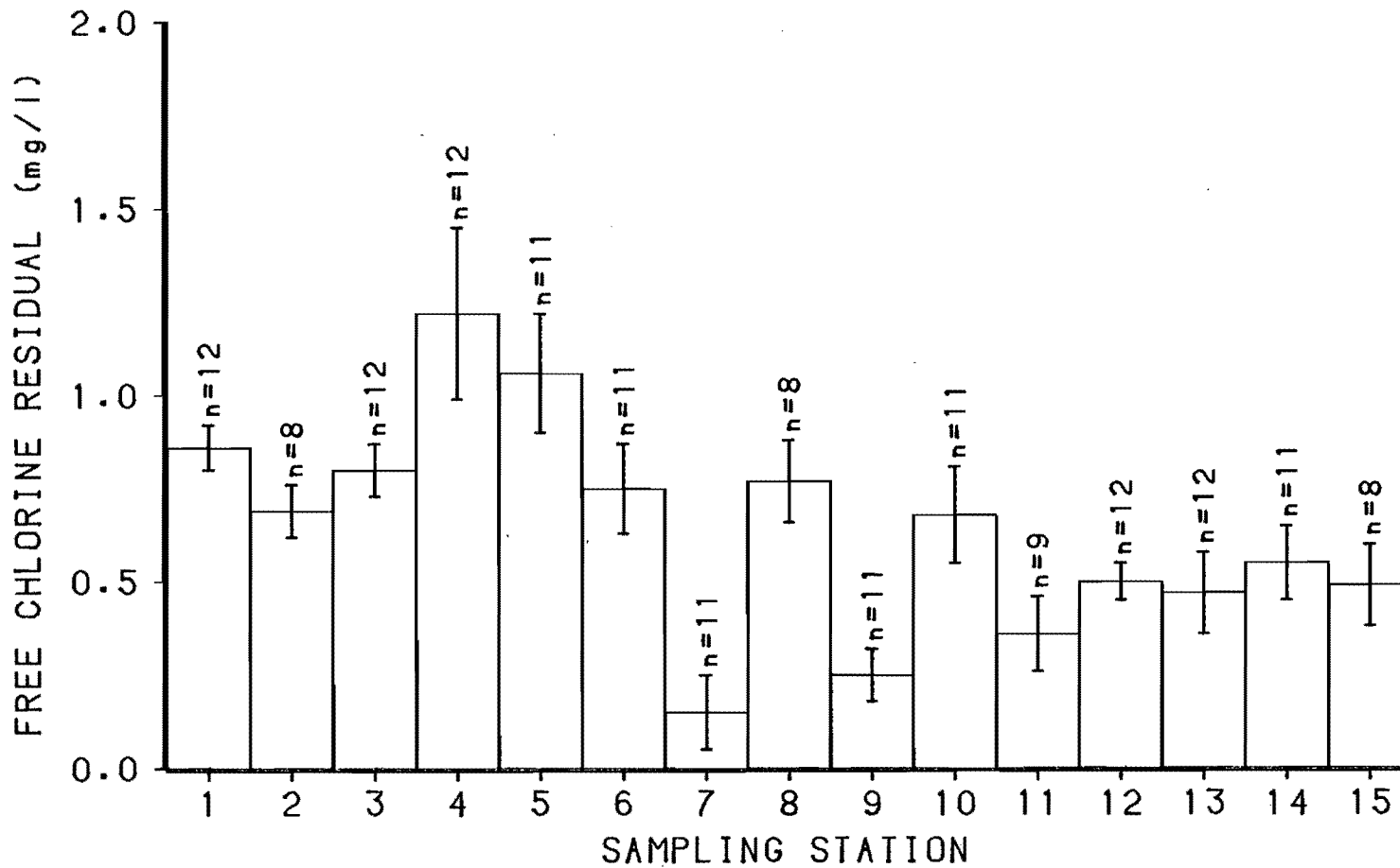
Figure 31. Finished water mean monthly free chlorine residuals with standard deviations for water treatment plants and distribution stations during 1981.
