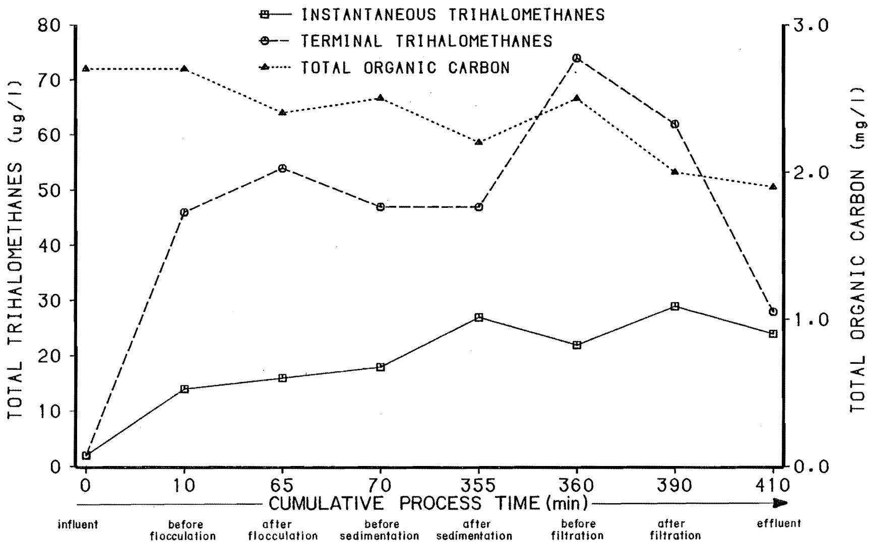
Figure 34. Trihalomethane formation and total organic carbon reduction at the Parleys water treatment plant on July 1, 1981.
