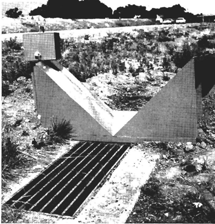
Figure 5. Bobbed tailed cutthroat flume used to measure the runoff at the Layton site.
