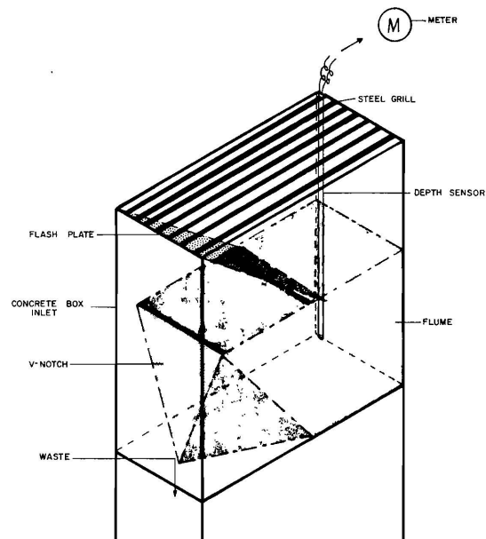
Figure 15. Drawings of grate inlet box with measuring flume in place.
