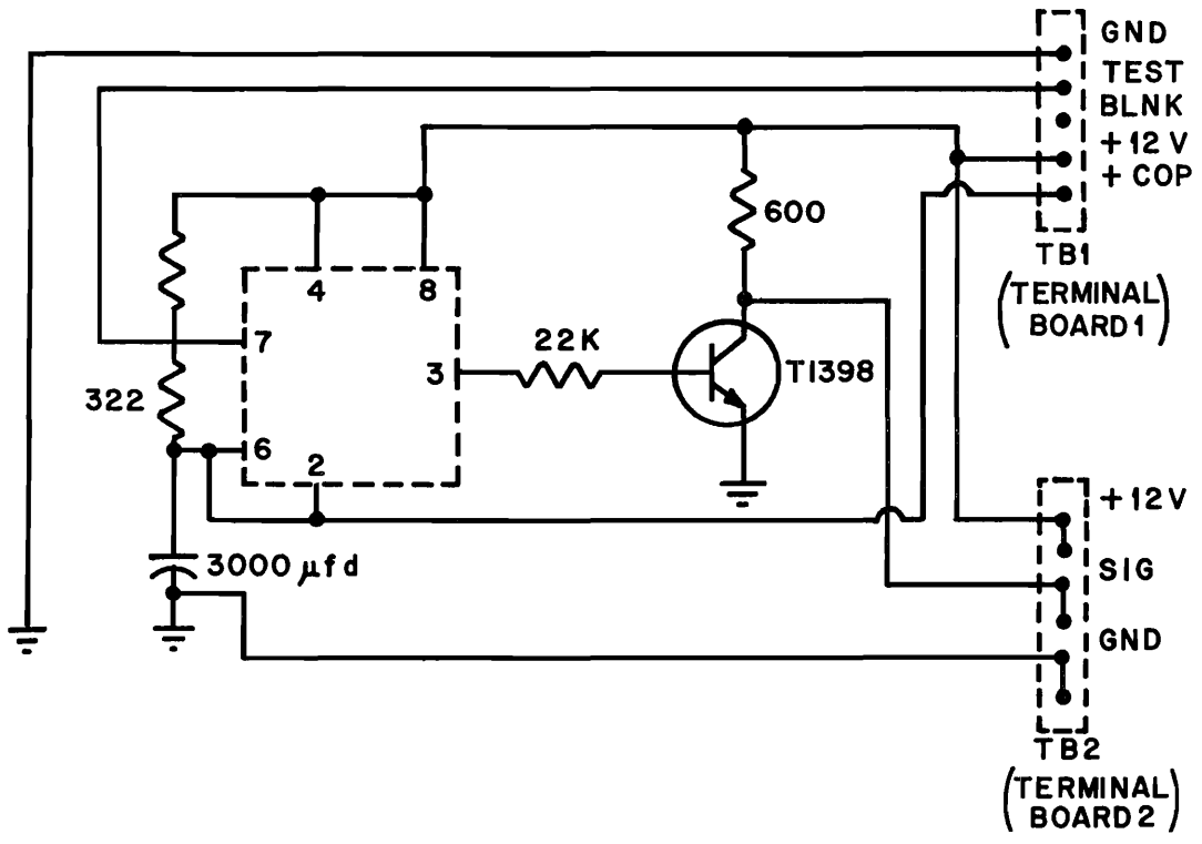
Figure 18. Schematic drawing of time synchronizer at both sites.
