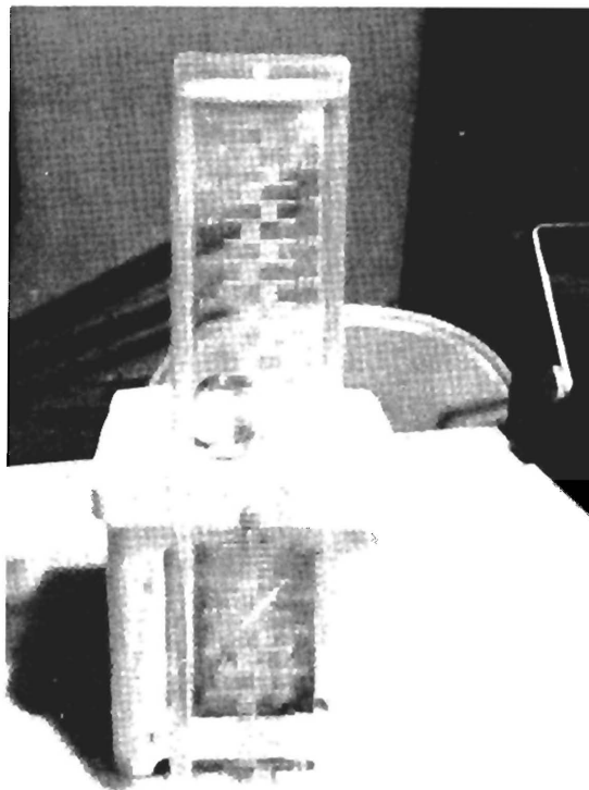
Figure 6. Typical weighing recording rain gage for measuring precipitation at the Layton site. The instruments at its base are the recorders for wind and soil moisture.
