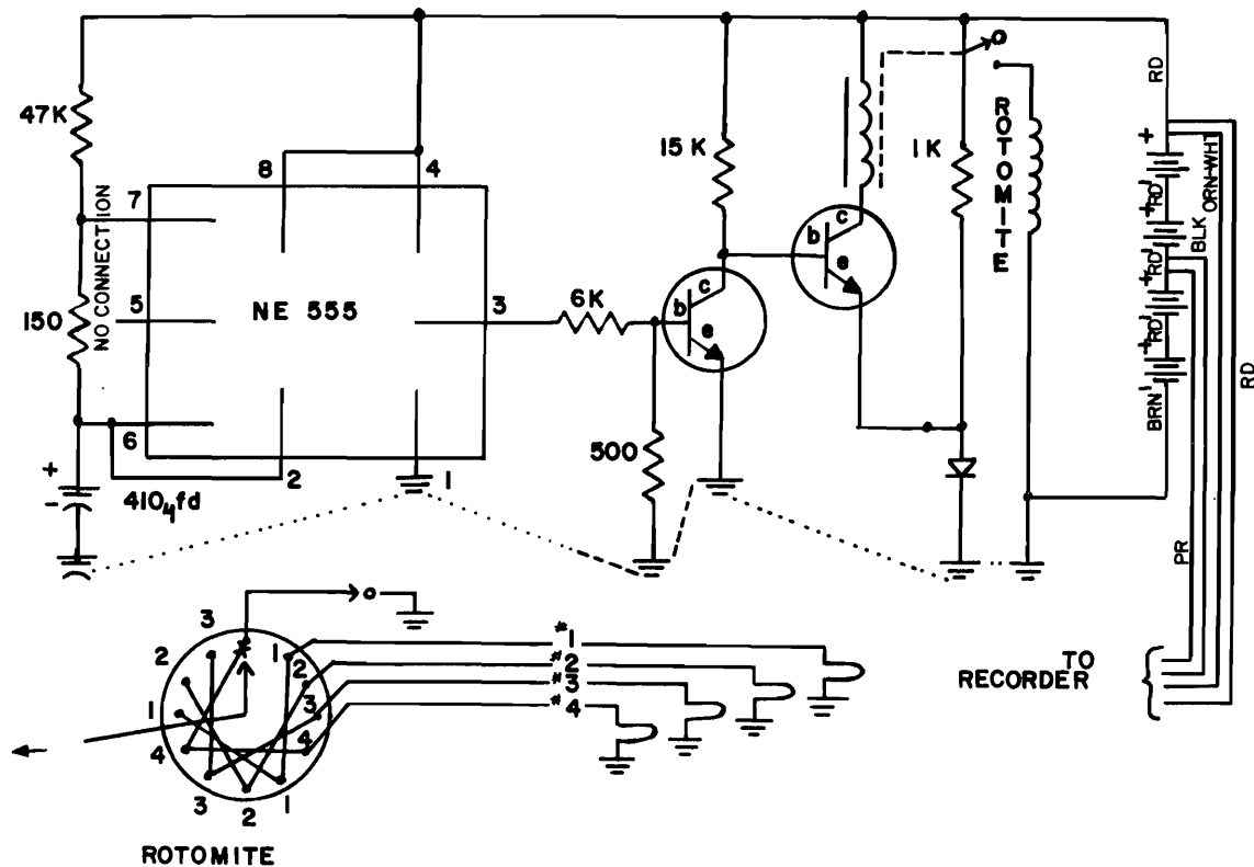
Figure 11. Switching system used to sense three soil moisture depths in sequence.
