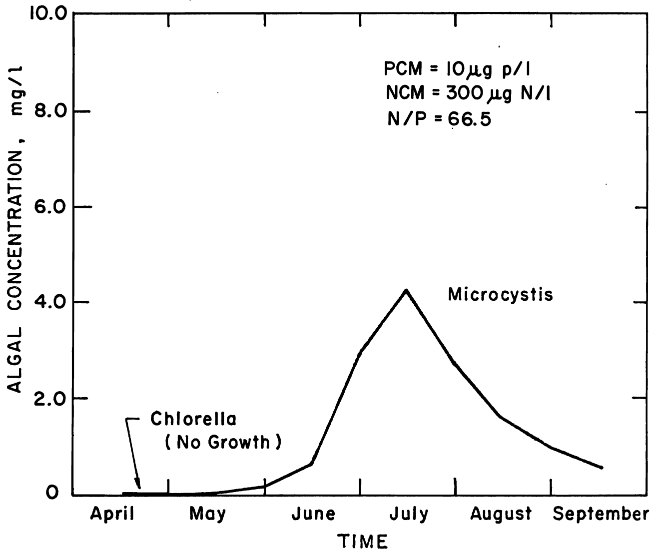
Figure 8. Microcystis uses virtually all of the available phosphorus when the initial nutrient concentrations are 10 \mu\text{g}\cdot\text{P}/\text{l} and 300 \mu\text{g}\cdot\text{N}/\text{l} , corresponding to an N/P ratio of 66.
