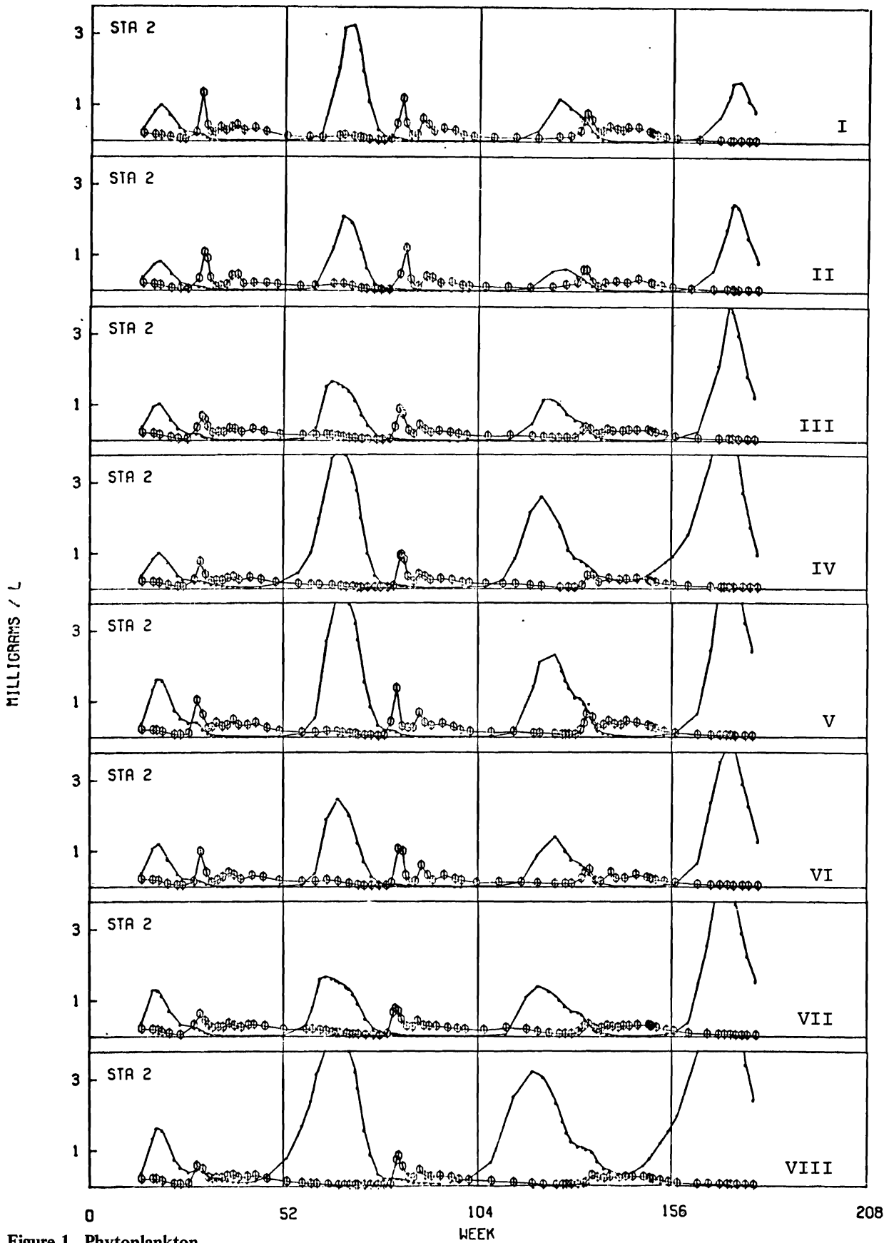
Figure 1. Phytoplankton.
