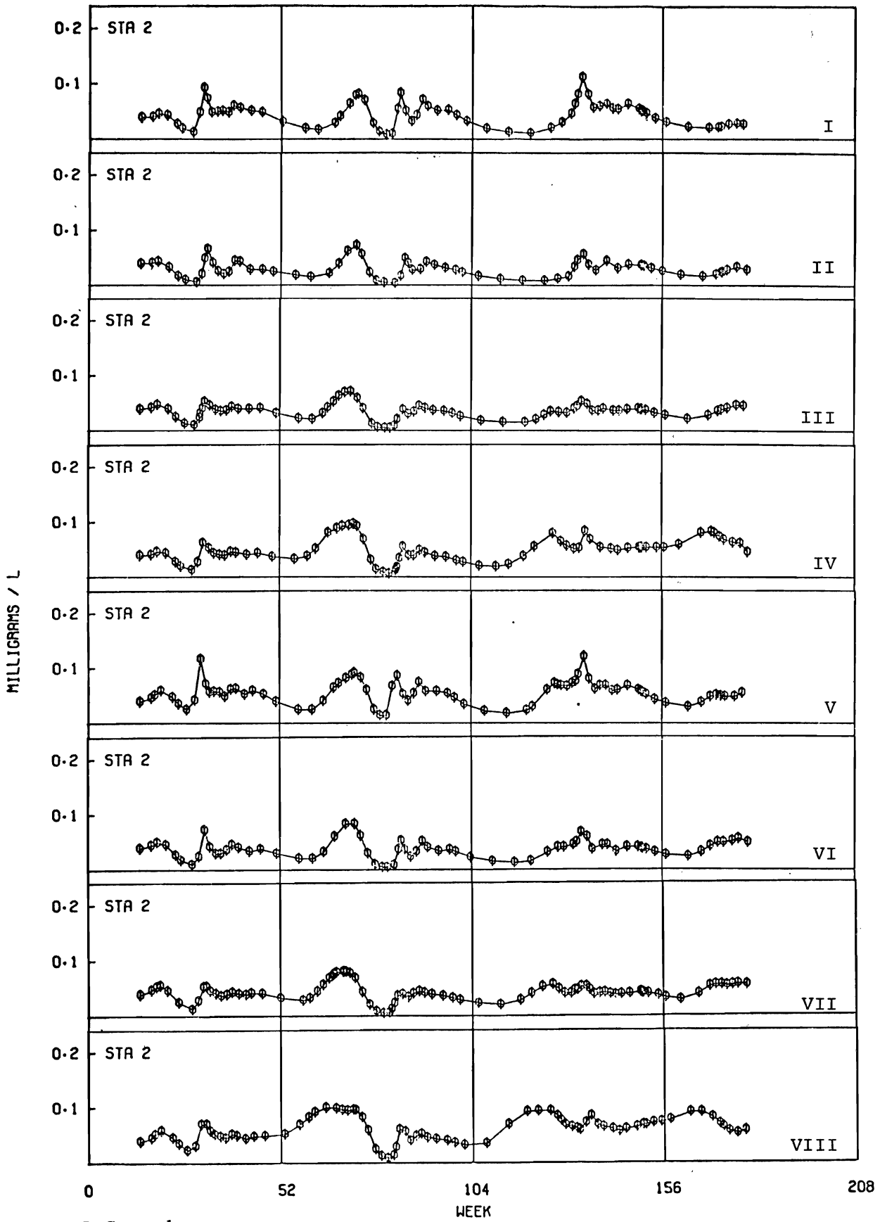
Figure 5. Copepods.
