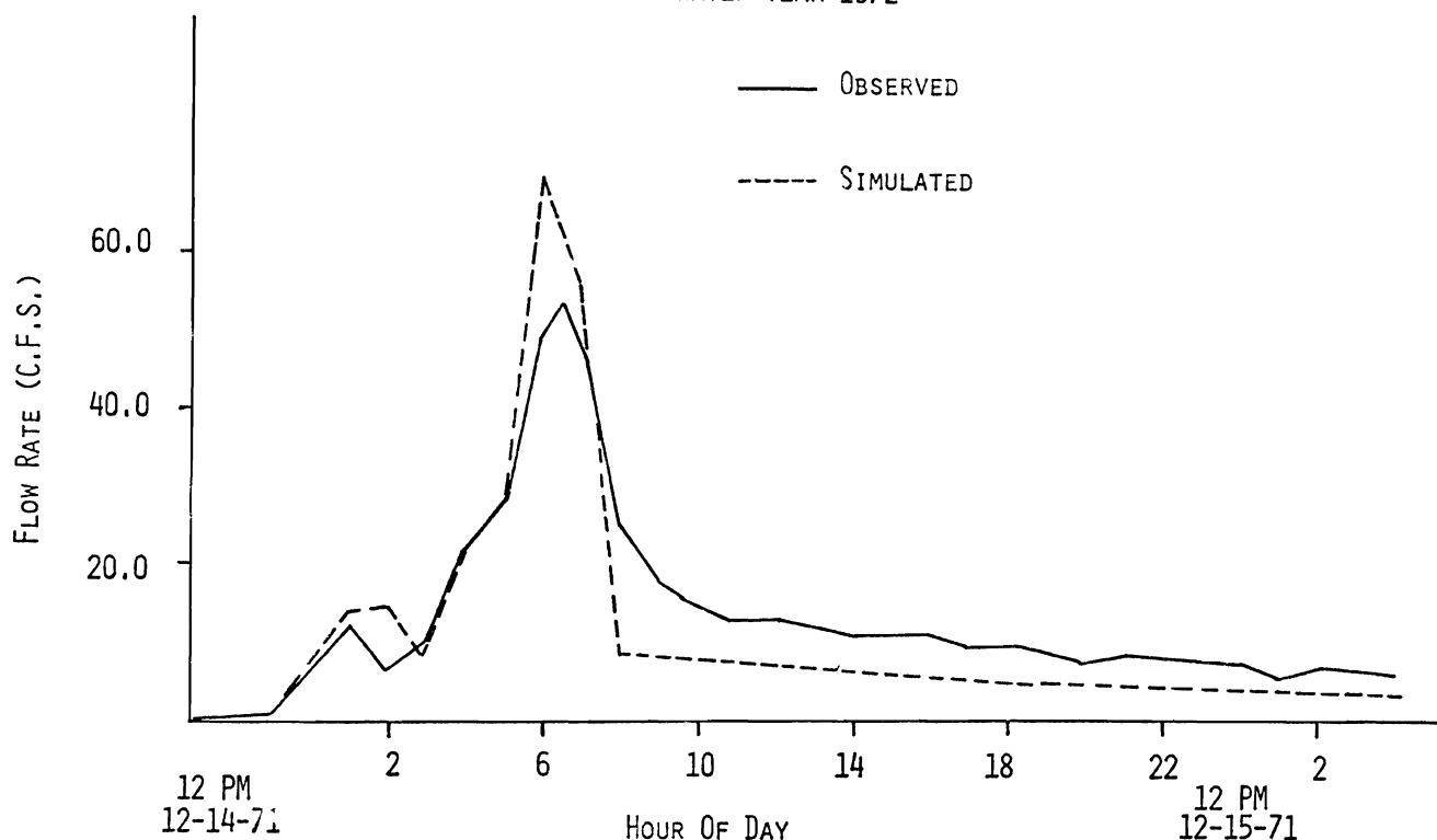
Figure 9. Storm hydrograph- Nakoma (December 15, 1971).
