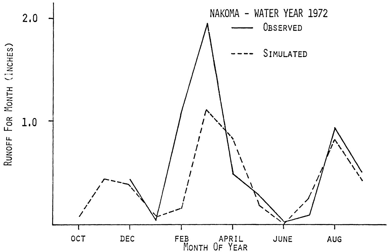
Figure 4. Observed vs. simulated runoff—Nakoma (1972).
