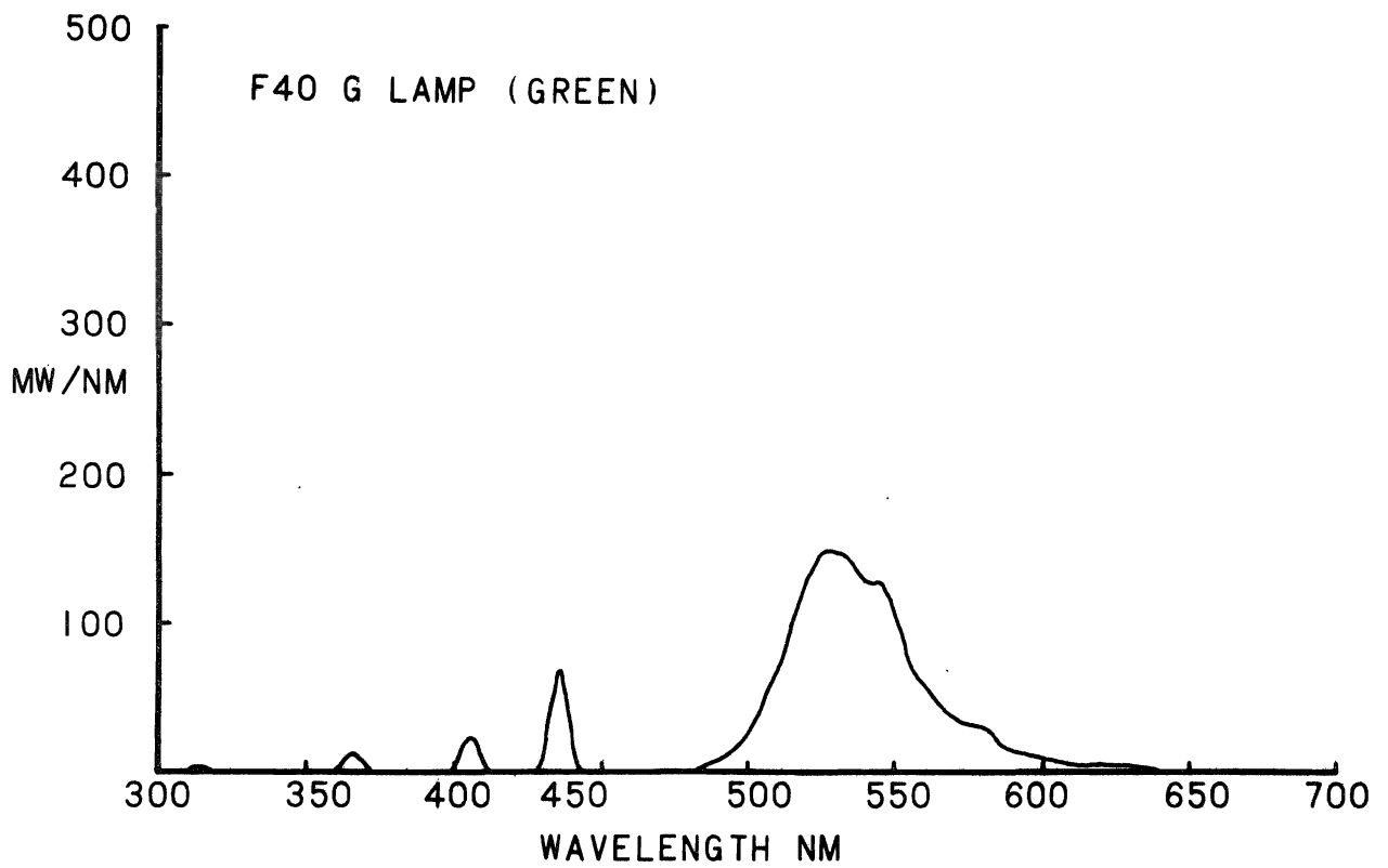
Figure 10. Fluorescent lamp spectral energy distribution curve.
