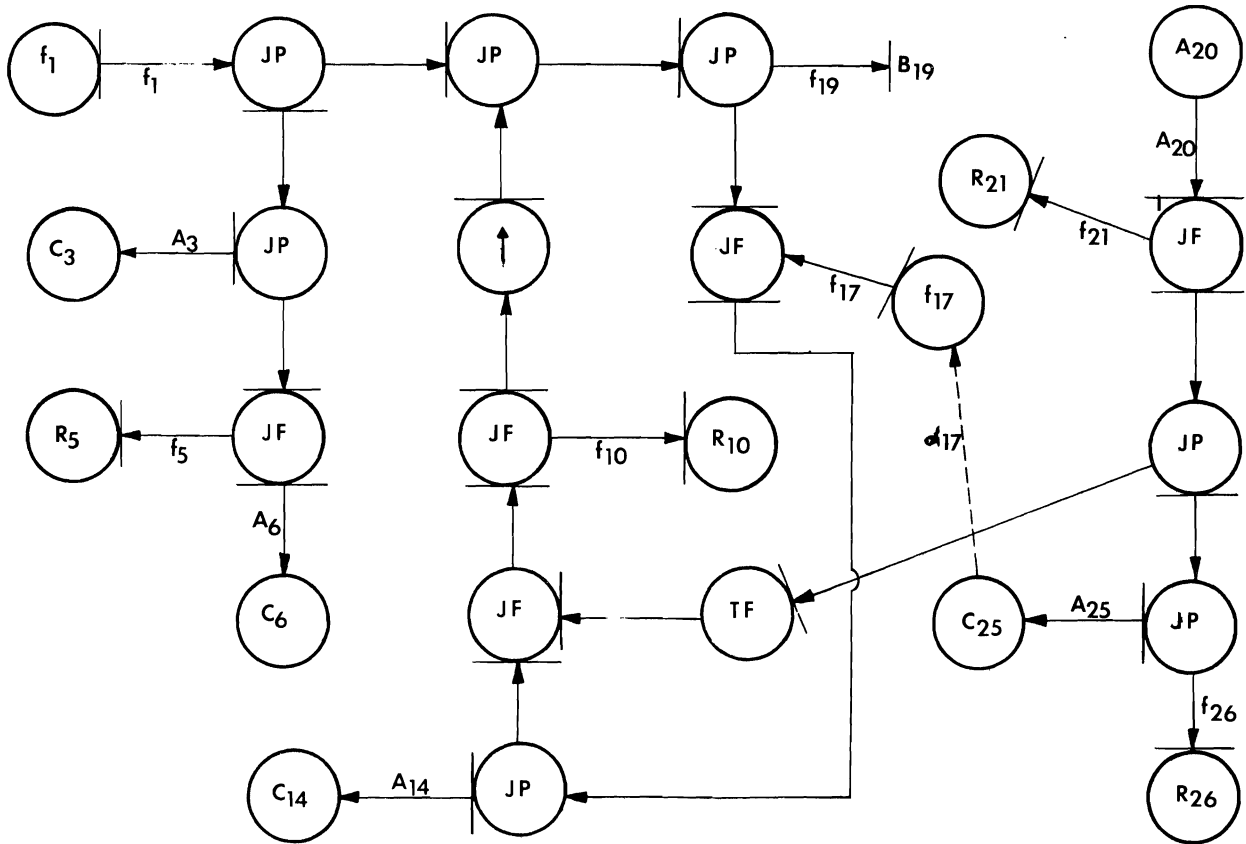
Figure 4. Bond graph of the oxygen subsystem of the microcosm with the independent variables indicated.
