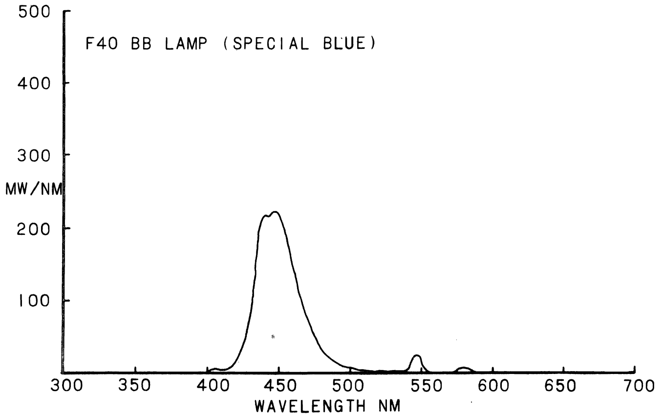
Figure 11. Fluorescent lamp spectral distribution curve.
