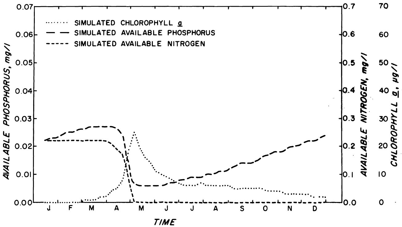
Figure 7. Simulation 3. C_L = 0.025 \text{ day}^{-1} .
