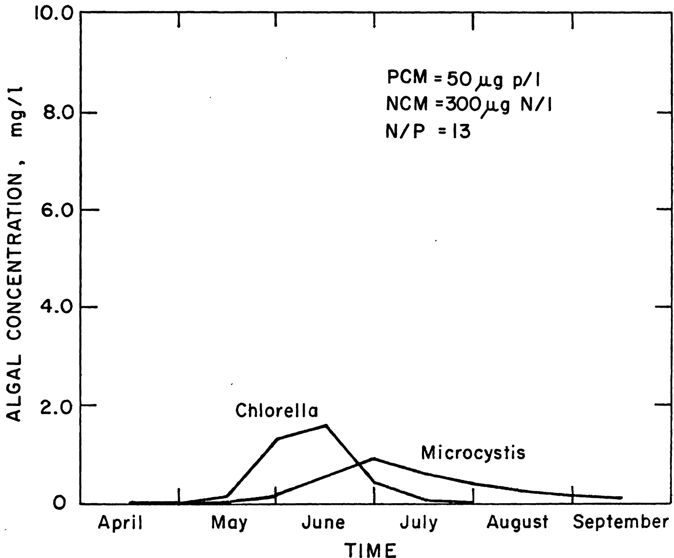
Figure 9. Chlorella dominates Microcystis because the initial phosphorus concentration of 50 \mu\text{g}\cdot\text{P}/\text{l} is sufficiently high that it can exploit its growth rate advantage and utilize most of the limited supply of nitrogen, 300 \mu\text{g}\cdot\text{N}/\text{l} , before the Microcystis .
