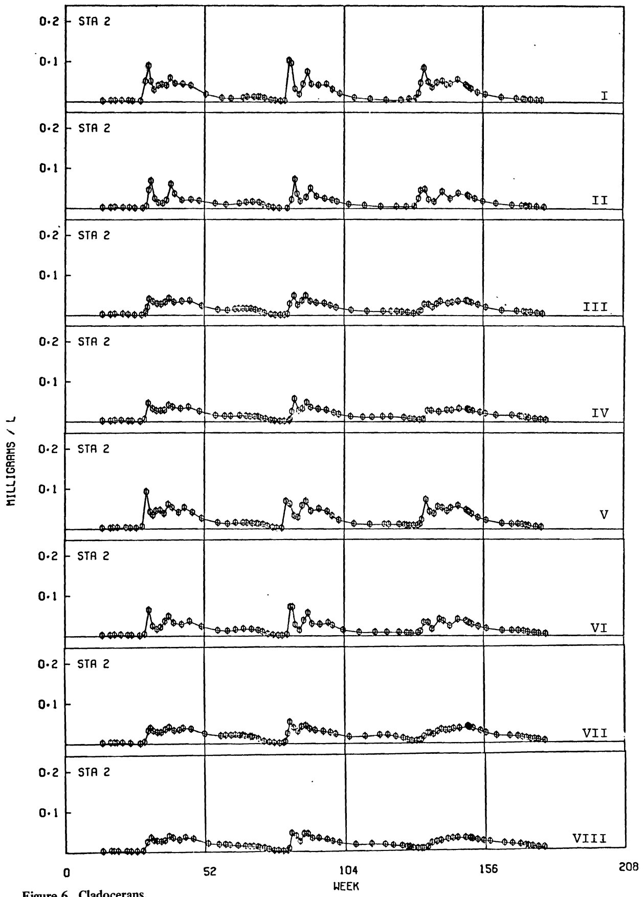
Figure 6. Cladocerans.
