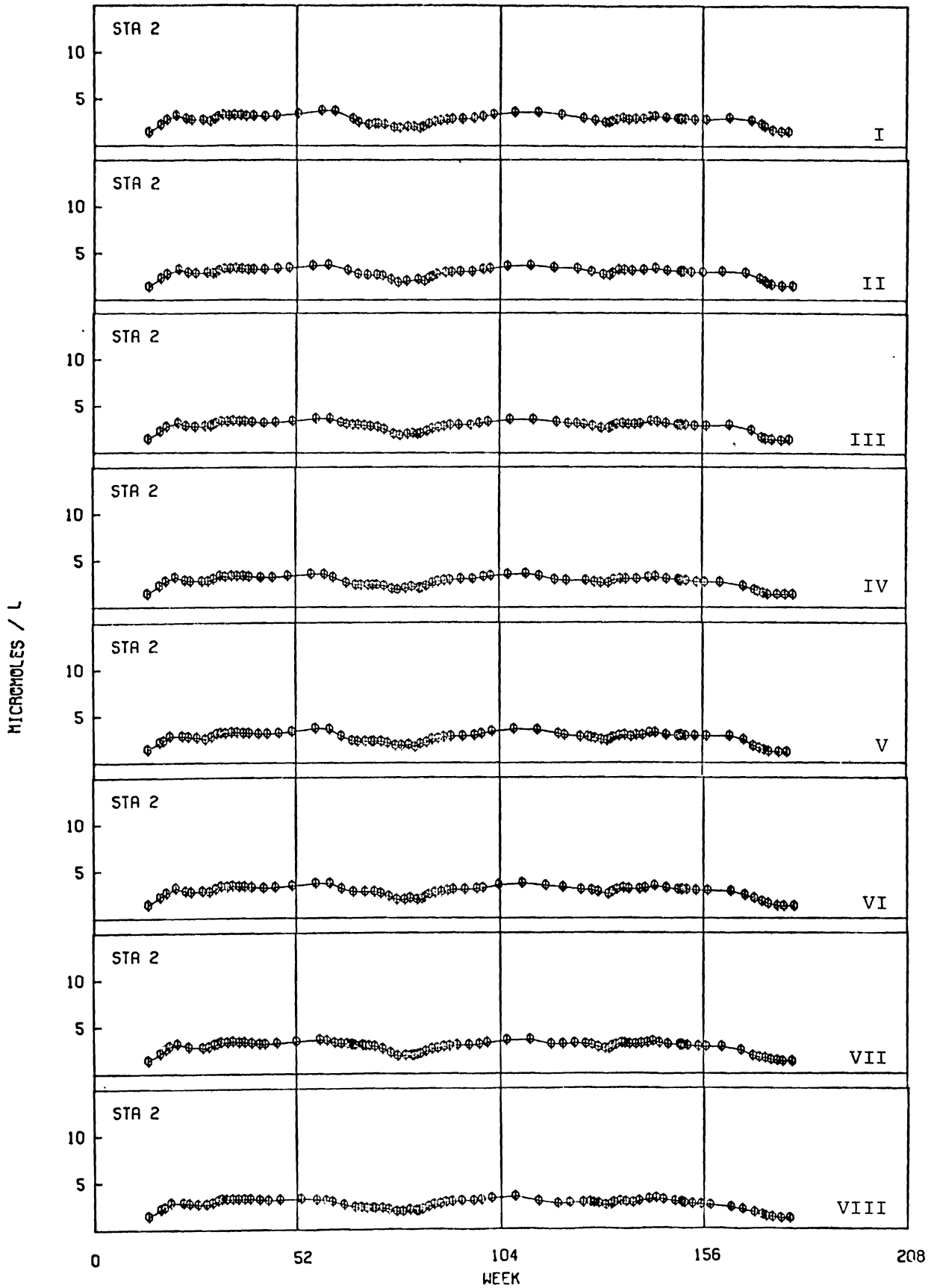
Figure 2. Phosphate.
