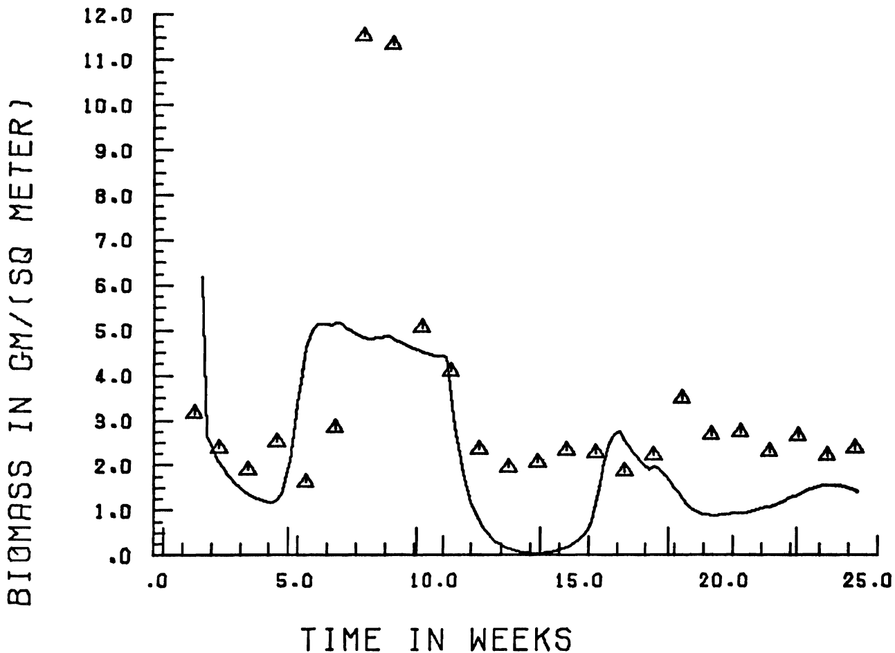
Figure 24. Output of open water model driven by hydrologic data. Nutrient input reduced by 95 percent.
