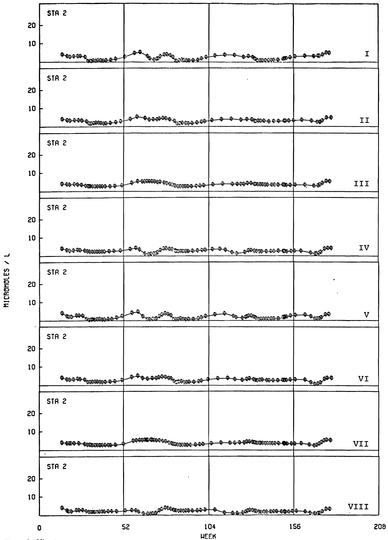
Figure 3. Nitrate.
