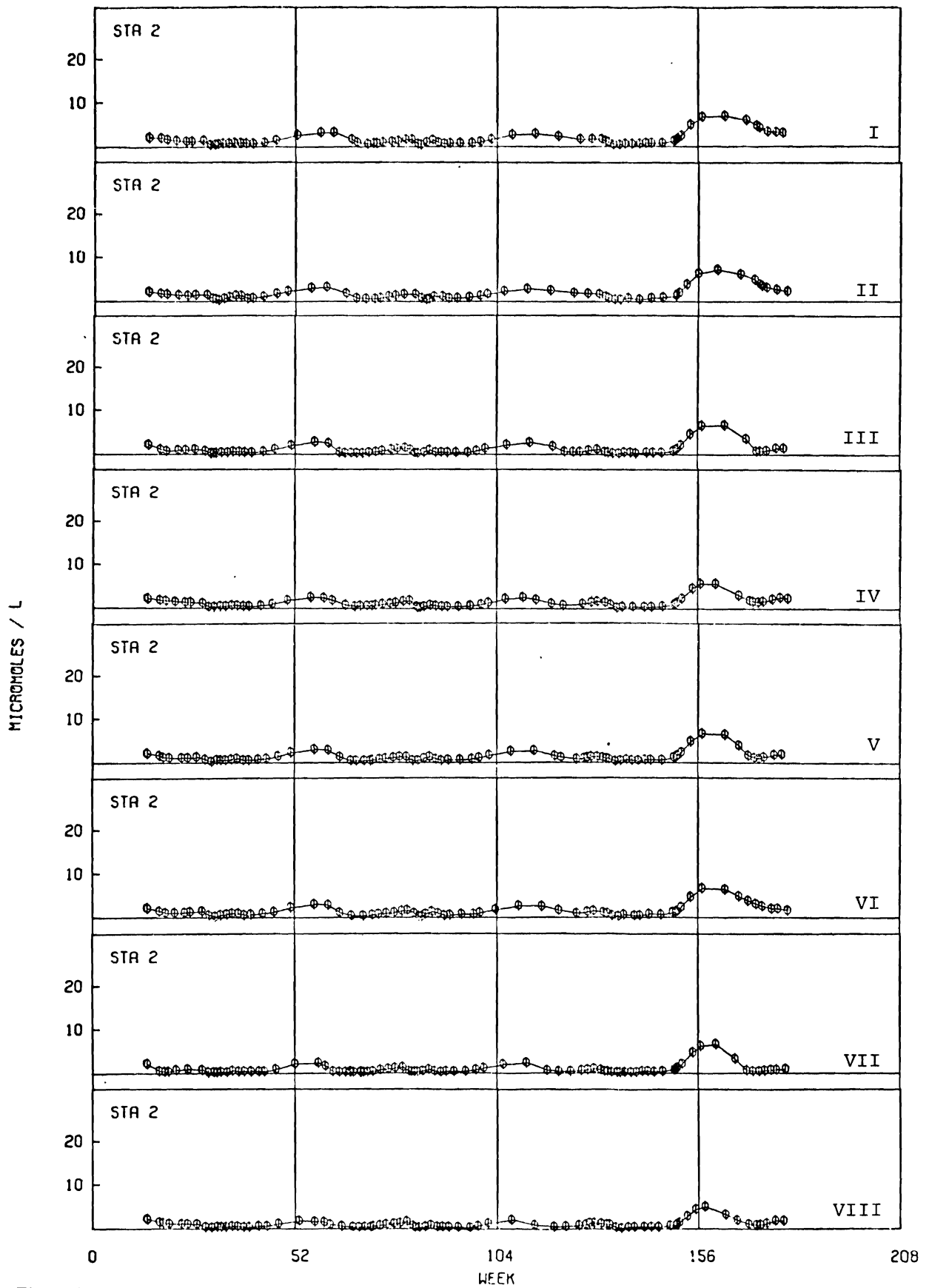
Figure 4. Ammonium.
