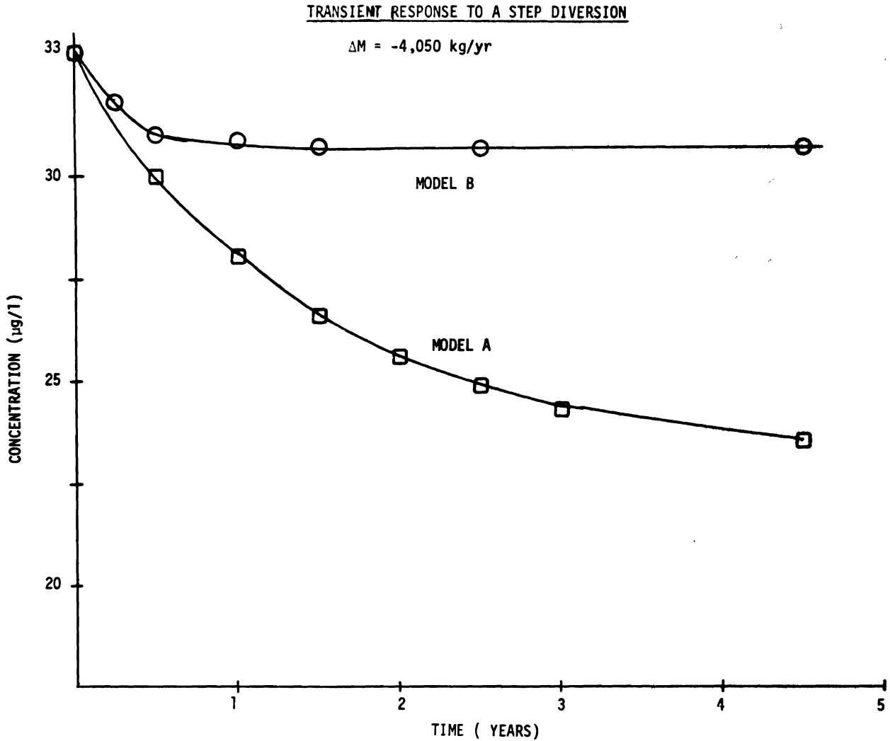
Figure 6. Transient change in total phosphorus concentration in Lake Sammamish predicted by two models in response to a 30 percent (4,050 kg/yr) decrease in phosphorus income.
