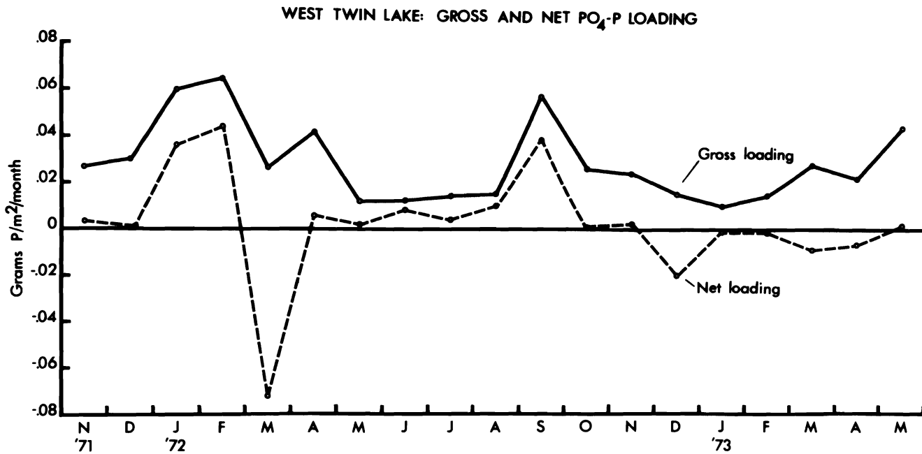
Figure 5. Gross and net PO 4 -P loading of West Twin Lake.
