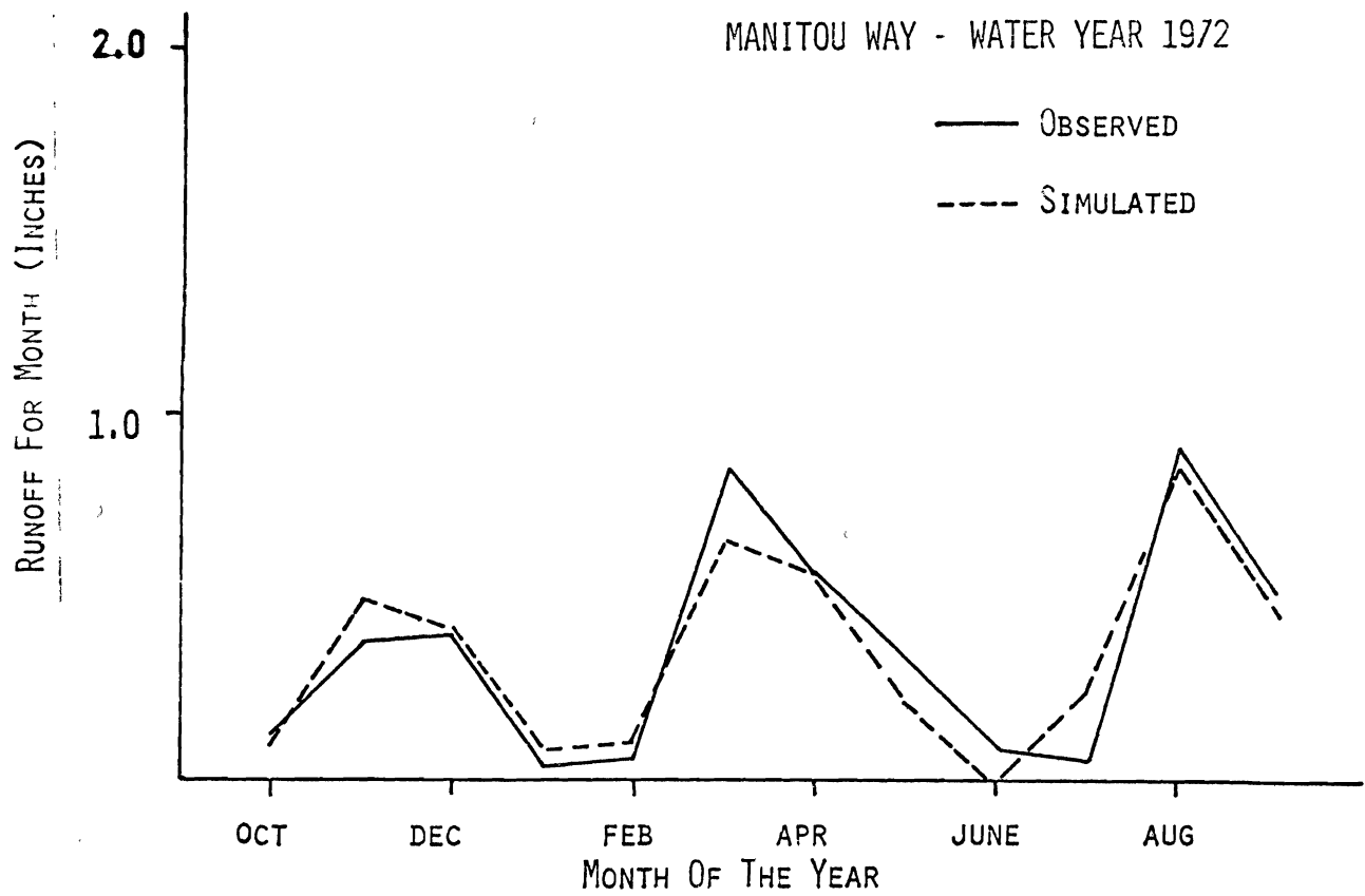
Figure 3. Observed vs. simulated runoff—Manitou Way (1972).
