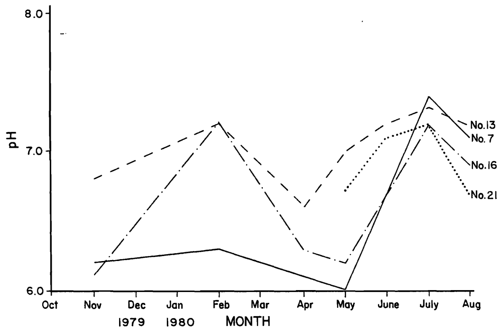
Figure 16. pH of groundwater in wells #7, 13, 16, and 21.
