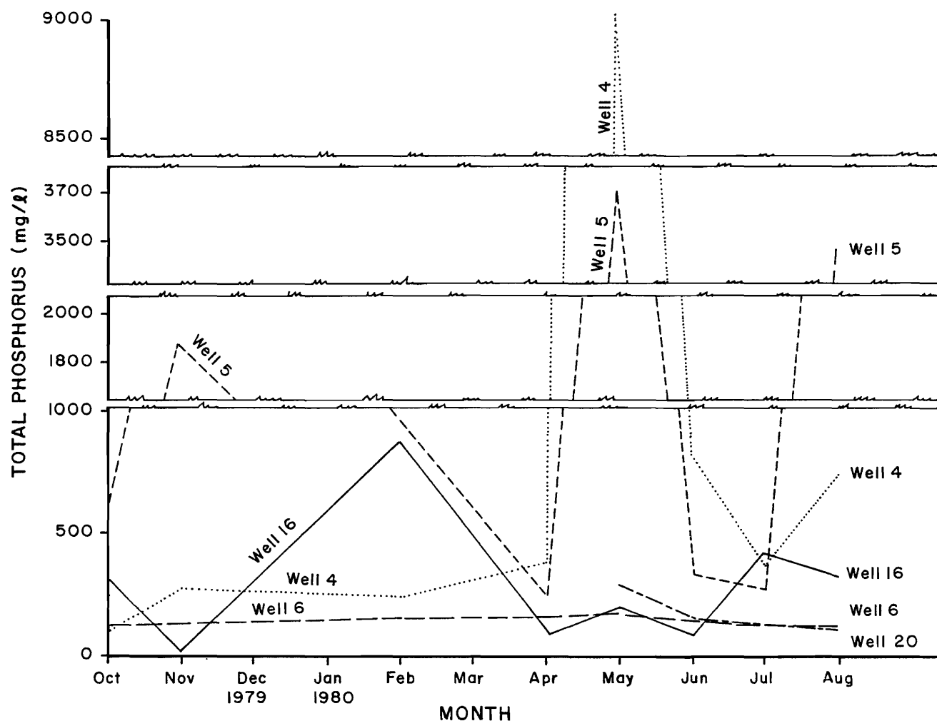
Figure 22. Total phosphorus concentration in wells #4, 5, 6, 16, and 20.
