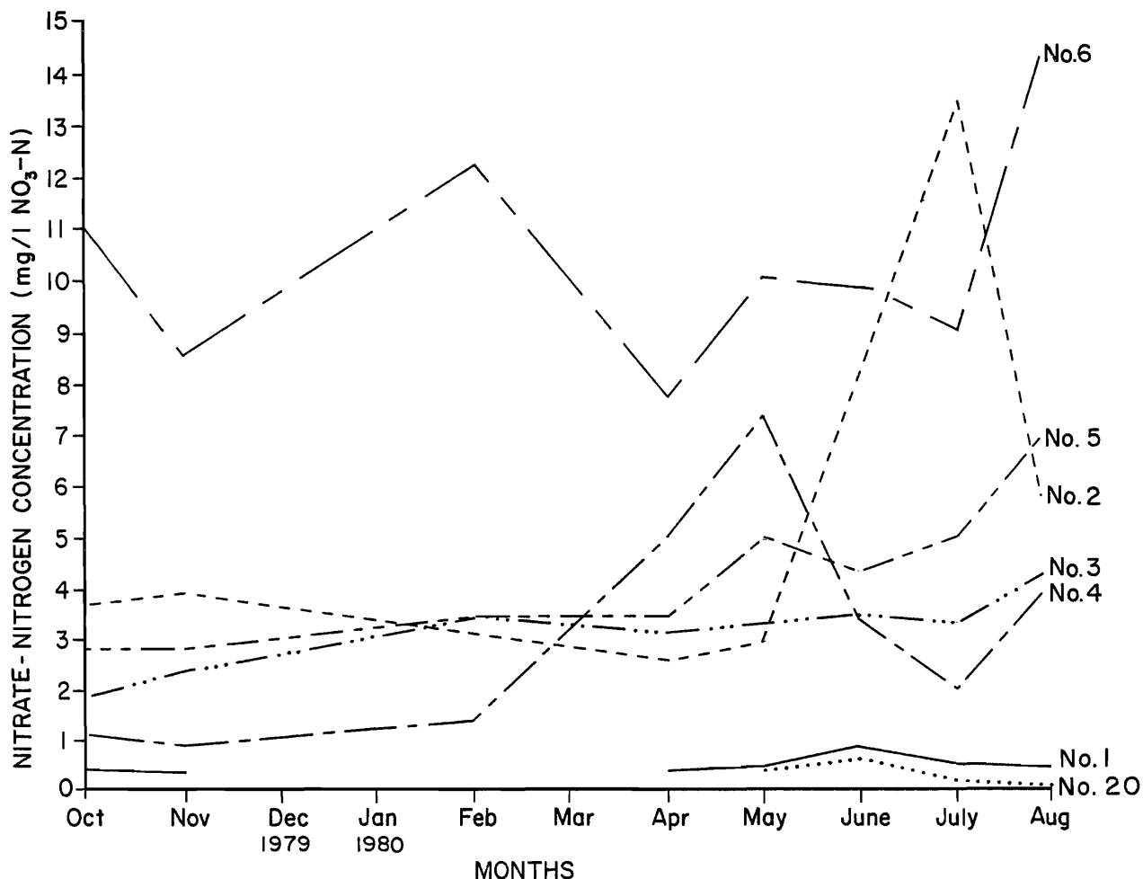
Figure 23. Monthly variation in \text{NO}_3^- concentration.
