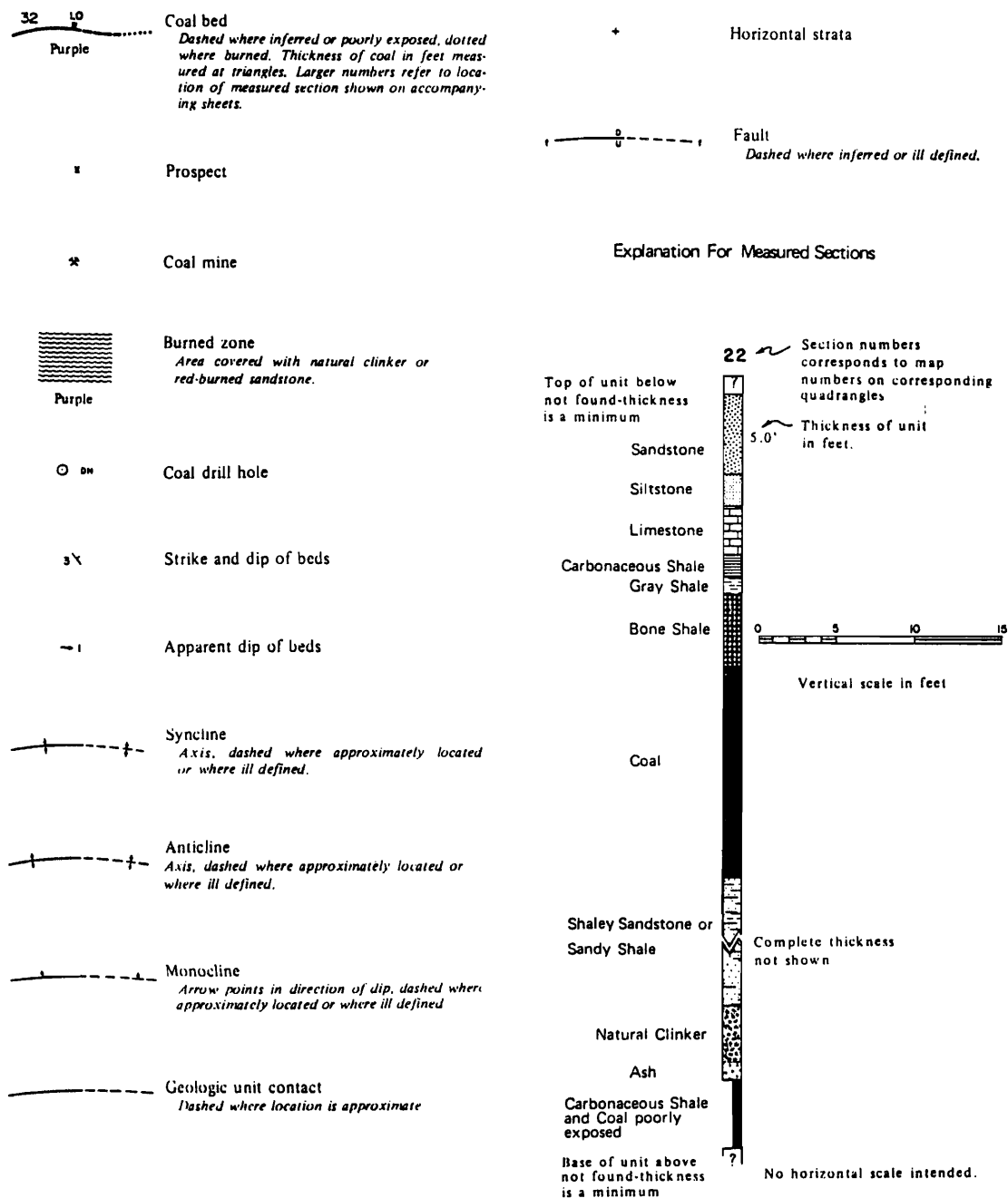
Figure N-4. Key to Figure N-2 (Doelling 1972, p. 137).
