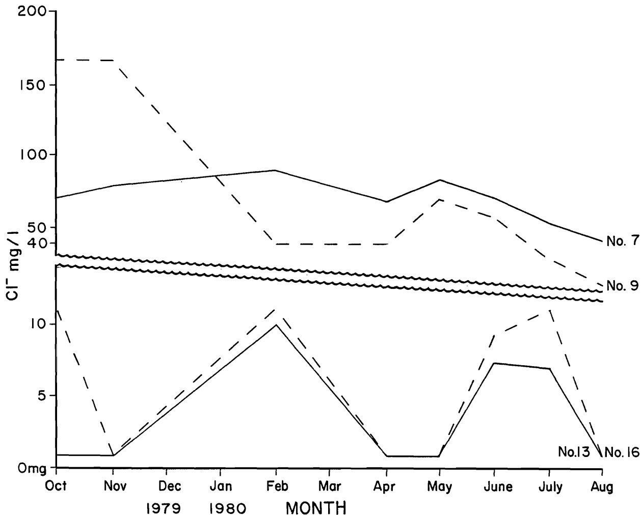
Figure 21. Chloride ion concentrations in wells #7, 9, 13, and 16 (mg/l).
