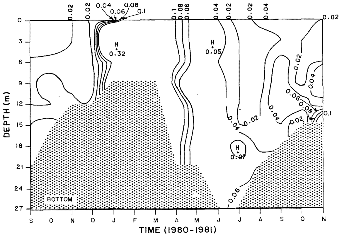
Figure 23. Nitrate plus nitrite concentration ( \text{mg N/l} ) isopleth for site C in Mt. Dell Reservoir.
