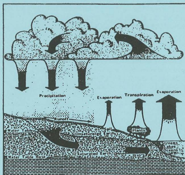
The hydrologic cycle. (Drawing by Rex Heer, Iowa State University)
