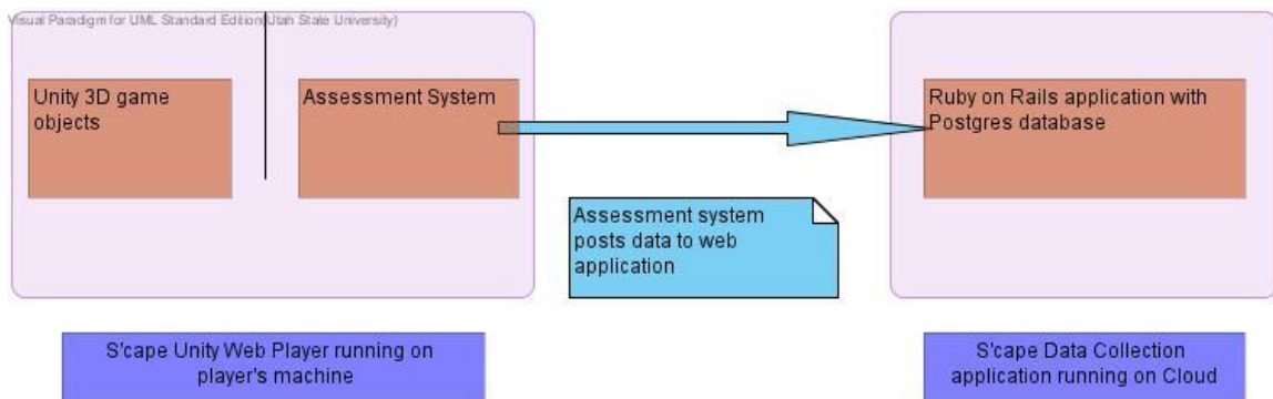
Figure 11 Overall architecture
