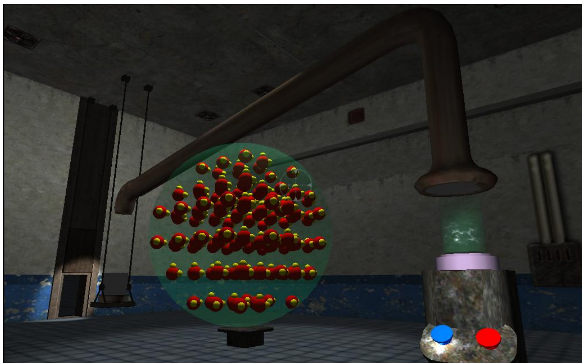
Figure 6. Molecular view of ice
