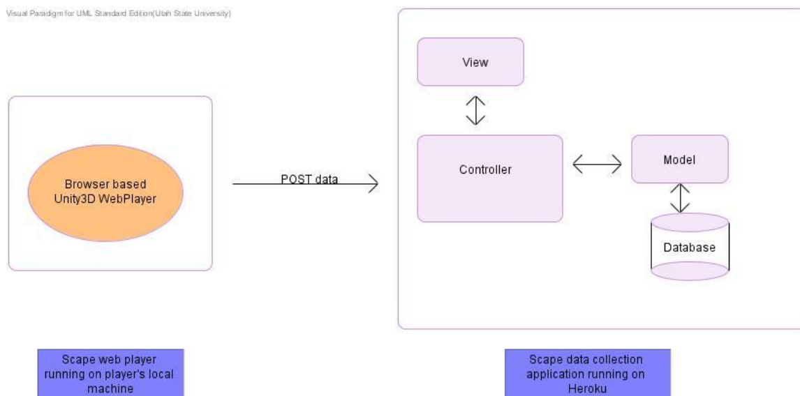
Figure 14. Data collection architecture
