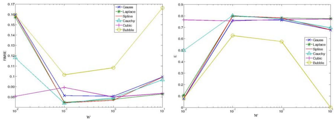
Fig. 2.10 Kernel type selection based on RMSE (left) and E (right)
