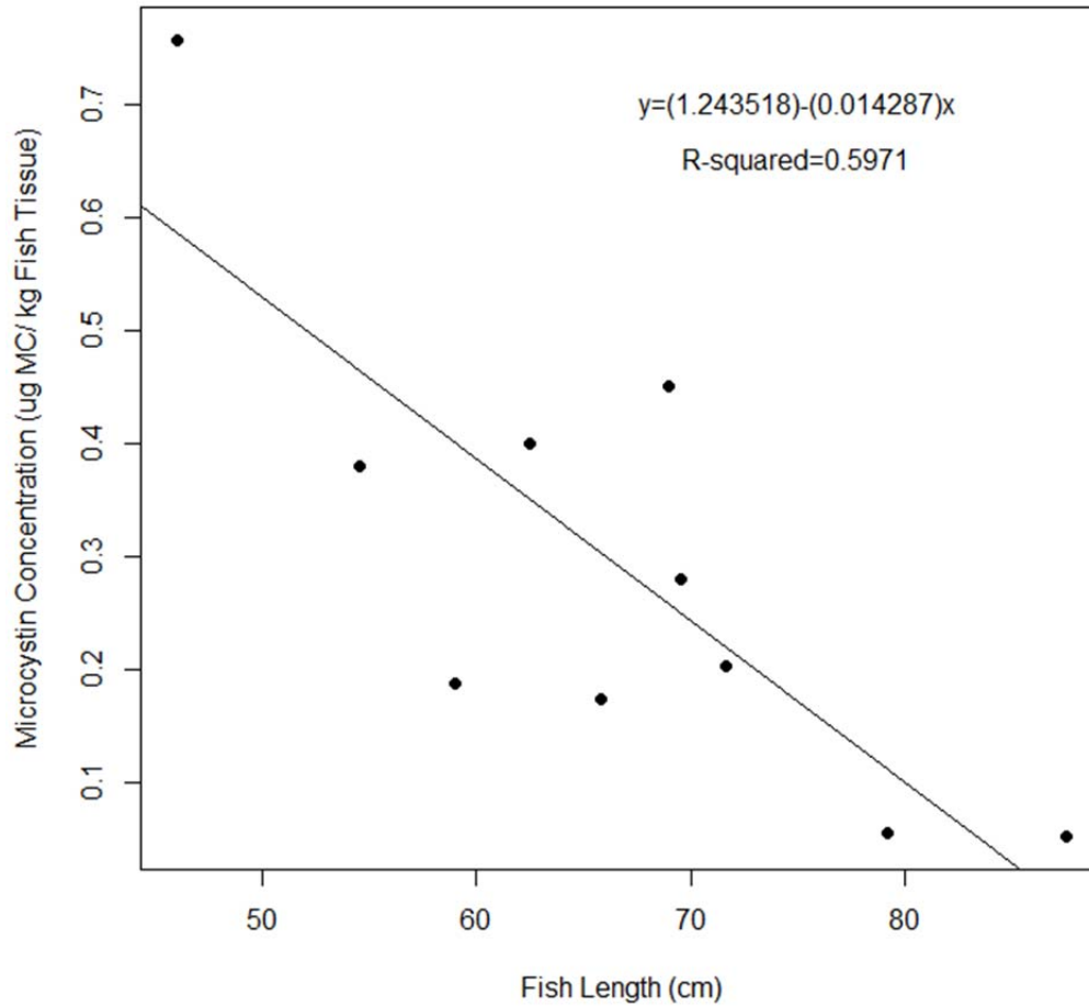
Figure 3: Relationship between fish length and microcystin concentration for northern pike collected from the St. Mary’s River, MI. A significant negative correlation was detected between total microcystin concentration within each northern pike and the total fish length ( S = 276 , p -value = 0.039, \rho = -0.673 ). A significant linear regression model was fit to data in order to characterize the observed trends ( F = 13.51 , p -value = 0.006).
