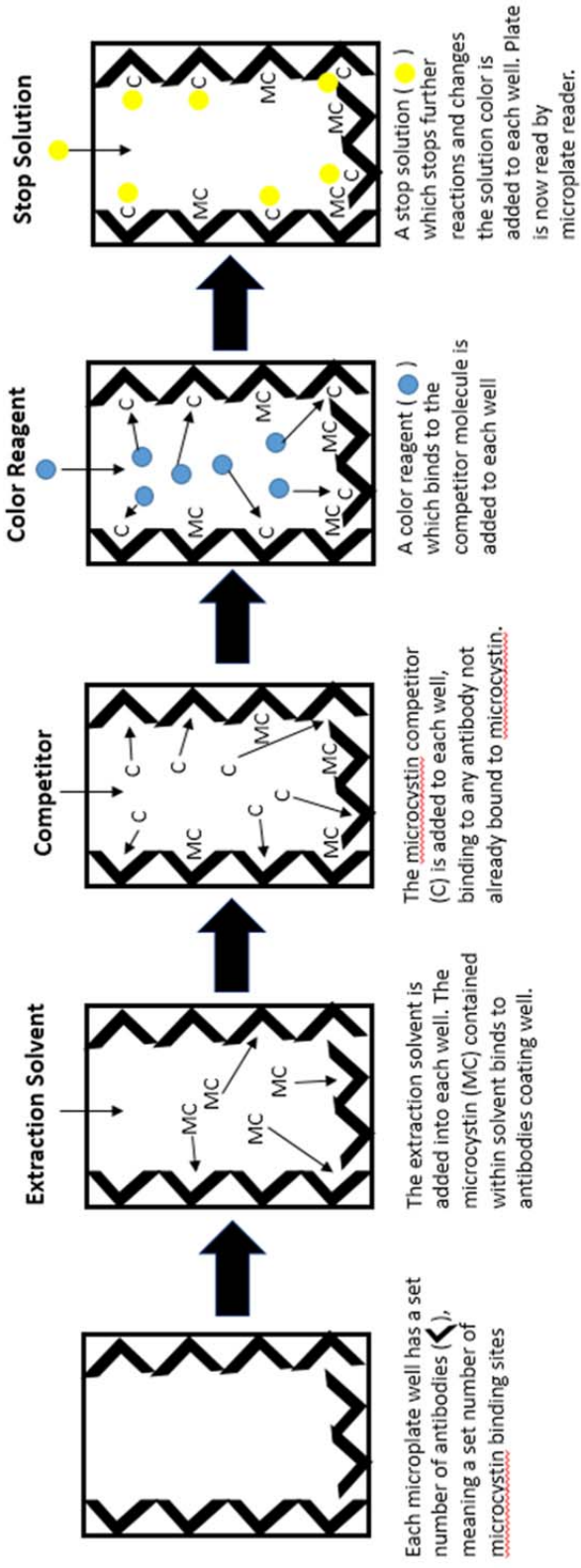
Figure 6: Schematic depiction of enzyme linked immune sorbent assay process for microcystin detection. Enzyme linked immune sorbent assay (ELISA) kits are microplate well kits, containing wells coated with antibodies capable of binding to features of the microcystin molecule. The rectangles pictured above represent a cross section of a single microplate well.
