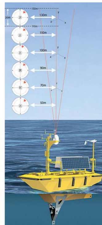
Figure 11 - WindSentinel wind data range gates
