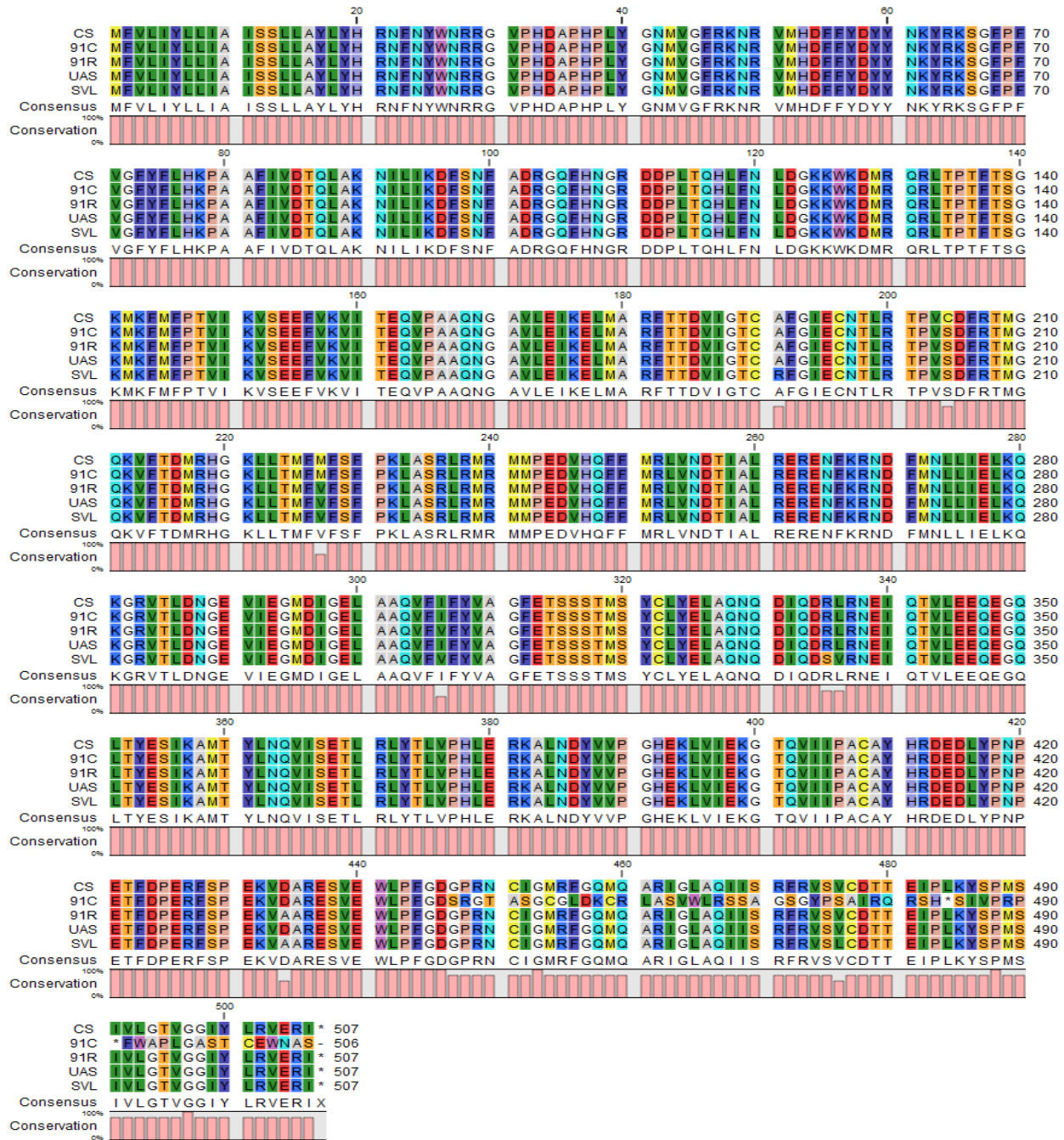
Figure 15. The CLC Protein sequence alignments between the CS , 91-C , 91-R , UAS-Cyp6a2 , and Cyp6a2SVL strains showed 9 amino acid substitution in total. The overall consensus is signified by a pink bar underneath the sequences. The SVL amino acid substitutions (R335S / L336V / V476L) were only present in the Cyp6a2SVL line, however, the DDT-resistant 91-R and the Cyp6a2SVL strains shared two mutations in common (I306C /D434A). At this time it is unclear which of these mutations may enable Cyp6a2 to metabolize DDT. The 91-C sequence is degenerate from 447 onward due to a base pair deletion leading to a frame shift mutation.
