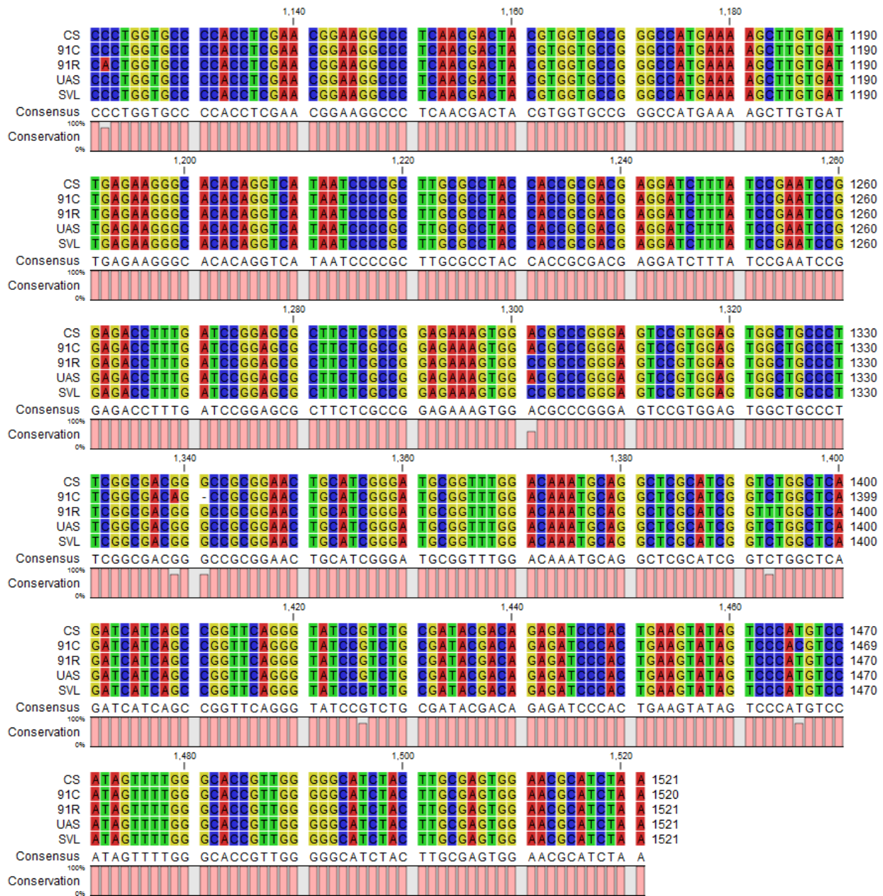
Figure 13. The CLC DNA sequence alignments between the CS , 91-C , 91-R , UAS-Cyp6a2 , and Cyp6a2SVL strains showed 21 SNP's were present in the coding region of Cyp6a2 . The overall consensus is signified by a pink bar underneath the sequences. The highly DDT-resistant 91-R line and the Cyp6a2SVL line have mutations in common at nucleotide positions 408, 916, 933, and 1301. The 91-C strain contained a single basepair deletion at position nucleotide 1341.
