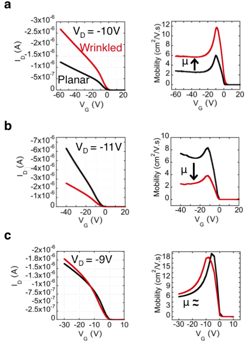
Figure 5.8: Effects of wrinkling single crystal field-effect transistors on mobility. a- c) Drain current I_D vs. gate voltage V_G corresponding to three different devices in their planar configuration and while undergoing wrinkling. Corresponding Mobility \mu = [L/WC_iV_D] (dI_D/dV_G) vs. gate voltage V_G is shown.
