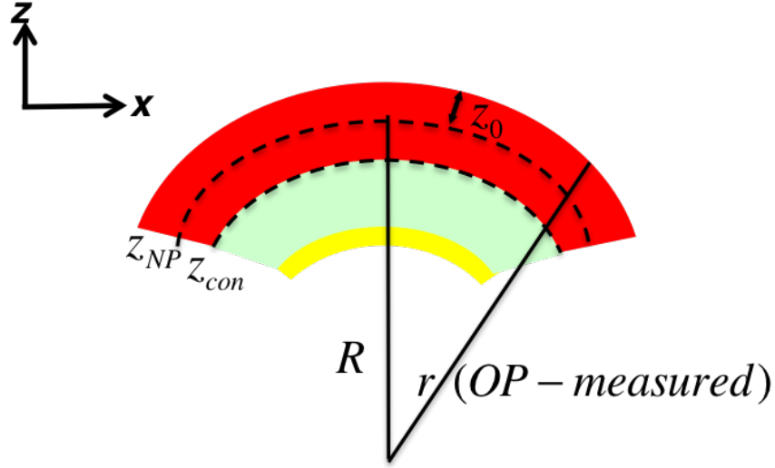
Figure 5.11: Bending of multilayered film.
