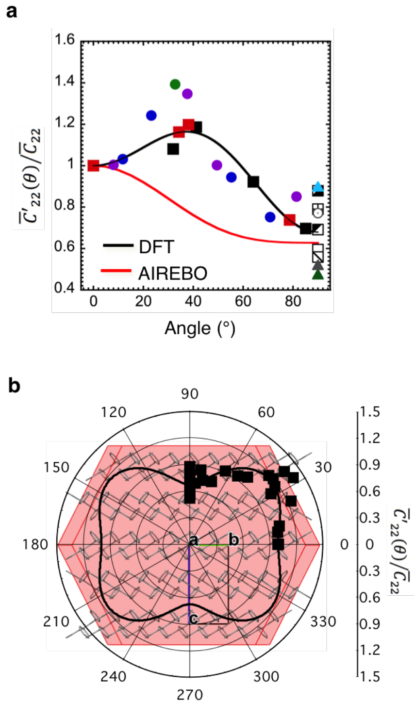
Figure 2.8: In-plane stiffness anisotropy in rubrene single crystals. a) Angular dependence of \bar{C}'_{22} normalized by \bar{C}_{22} . Marker shape indicates different substrate modulus. Marker color indicates different crystal sample. b) Polar plot of experimental data in (a) overlaid on structure of (100) face of rubrene. Black line shows Equation 2.4 with elastic constant values from DFT.
