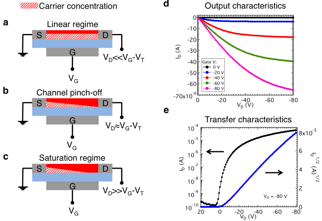
Figure 1.4: Field-effect transistor operation. a-c) Carrier concentration profiles for different operation regimes. d) Output and e) transfer characteristics for representative rubrene single crystal transistor.
