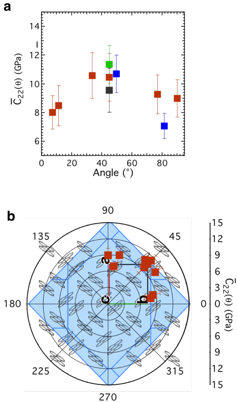
Figure 2.19: In-plane stiffness anisotropy in perylene single crystals. a) Angular dependence of \bar{C}'_{22} . Marker color indicates different crystal sample. b) Polar plot of experimental data in (a) overlaid on structure of (100) face of perylene.
