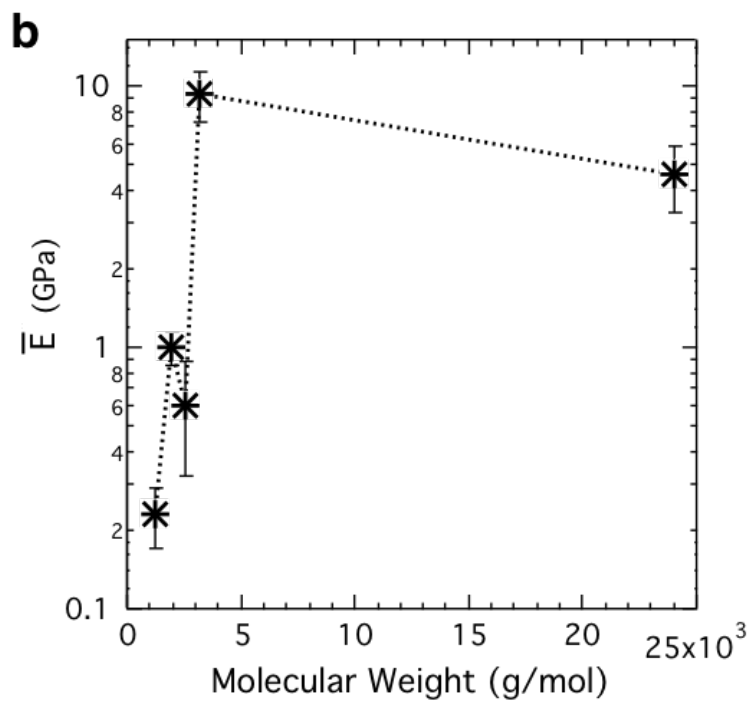
Figure 3.5: In-plane elastic moduli of a) BTTT oligomers and b) BTTT oligomers and polymer as a function of molecular weight.
