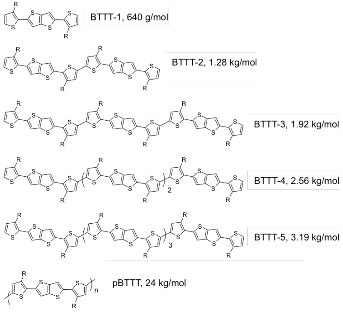
Figure 3.1: Chemical structures of BTTT series. R = C 12 H 25 .
