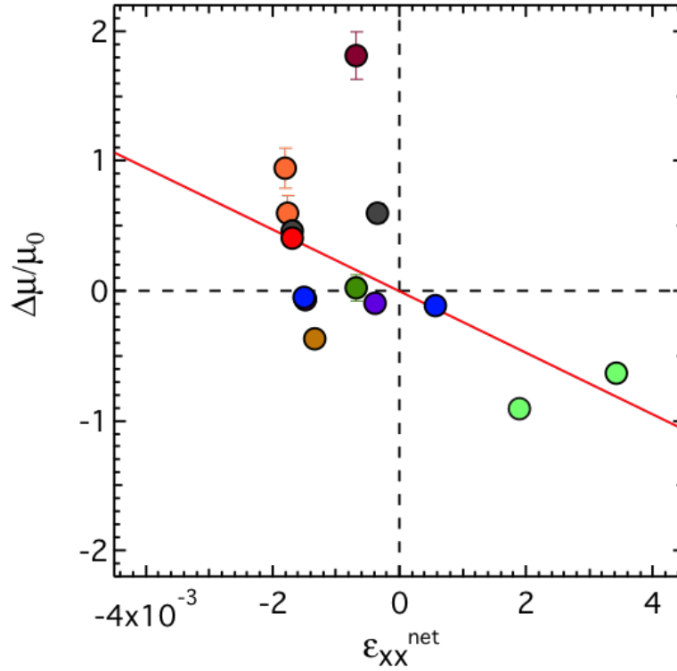
Figure 5.13: Effect of net channel strain in field-effect carrier mobility of rubrene transistors. Net compression (negative values) causes mobility increase and the opposite effect is observed for net channel tension (positive values). Different colors represent different devices. Individual device details are shown in Appendix B.
