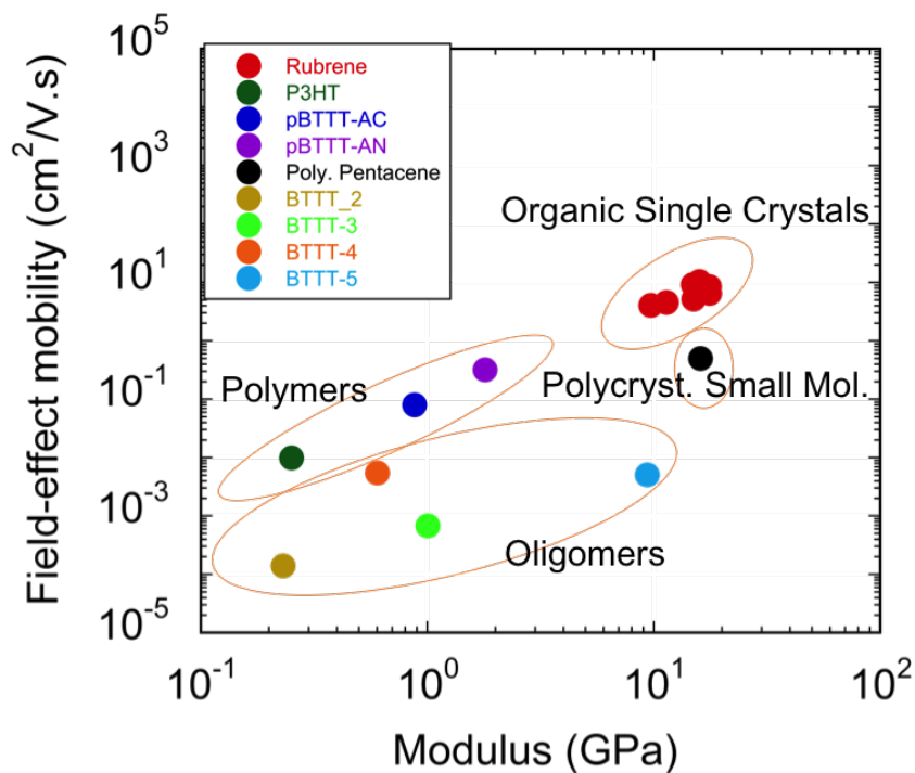
Figure 6.1: Average field effect mobility of organic semiconductor materials as a function of average modulus. Average mobility and modulus values for P3HT, pBTTT as-cast (AC) and annealed (AN) were obtained from O'Connor et al. [32]. Average mobility and modulus values for polycrystalline pentacene were obtained from Tahk et al. [31].
