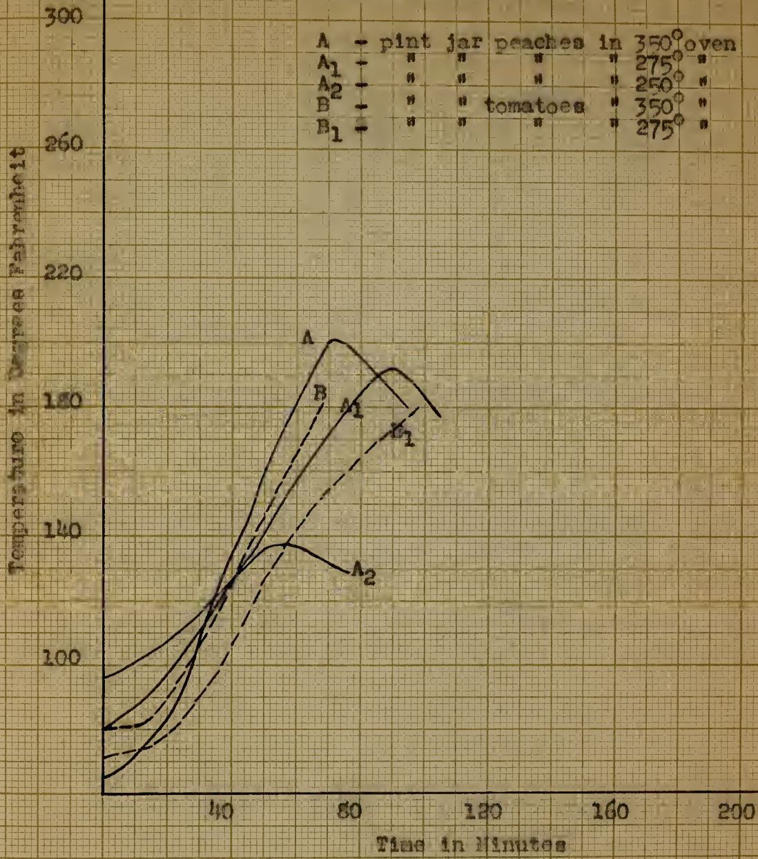
Figure 15. Effect of gas oven temperature upon the rate of heat penetration in pint jars of tomatoes and peaches.
