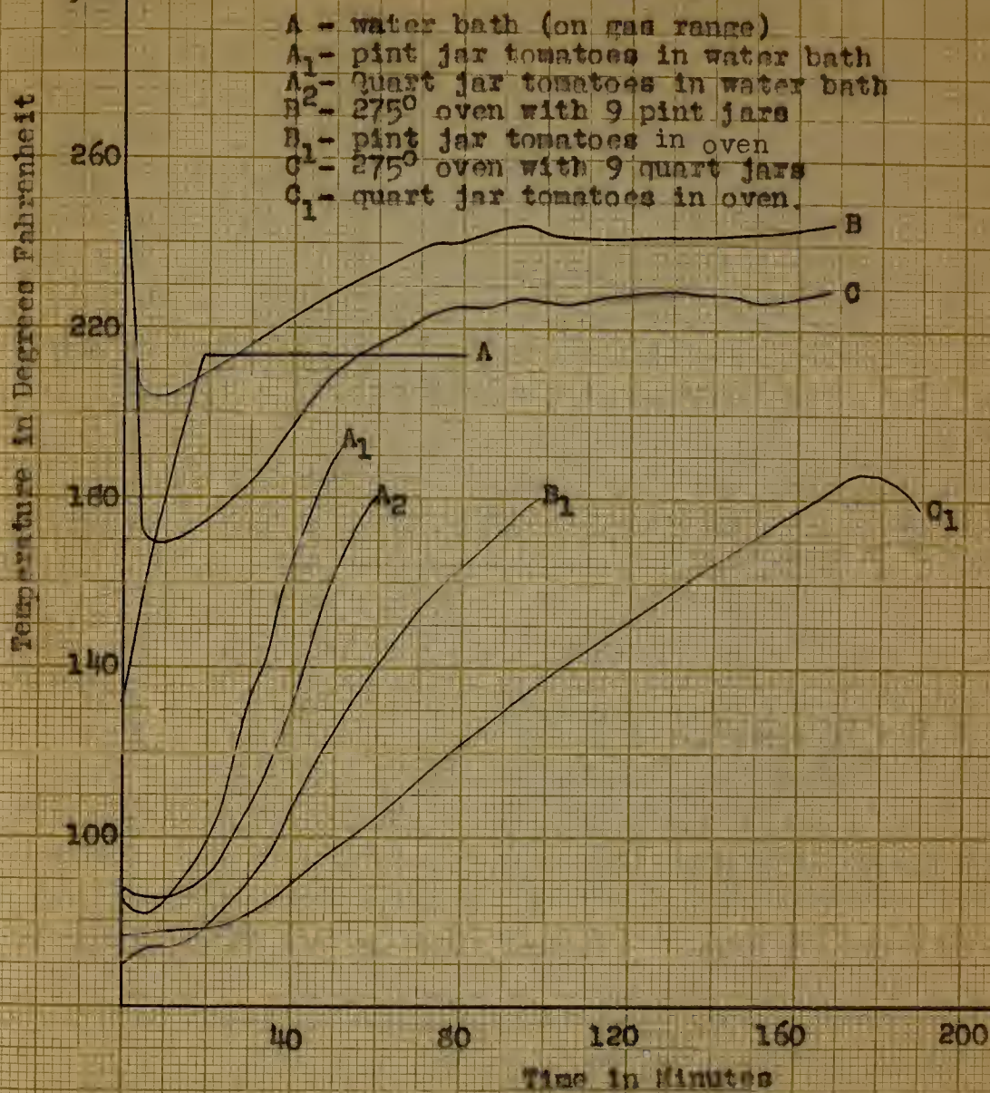
Figure 14. Comparison of the rate of heat penetration in pint and quart jars of tomatoes processed in the water bath and in the gas oven.
