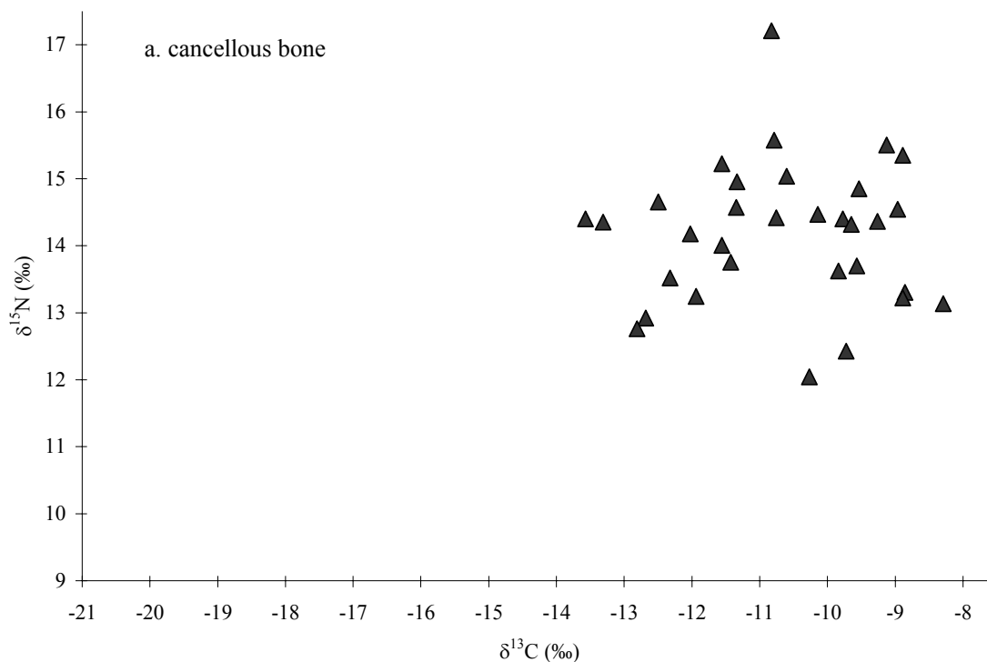
Figures 1a-1c: \delta^{13}\text{C} and \delta^{15}\text{N} values for all skeletons under study, by skeletal element. NB: the tooth dentine and cortical bone values show a greater spread than those derived from cancellous bone collagen, which attests to the diverse origins of the individuals in this group.
