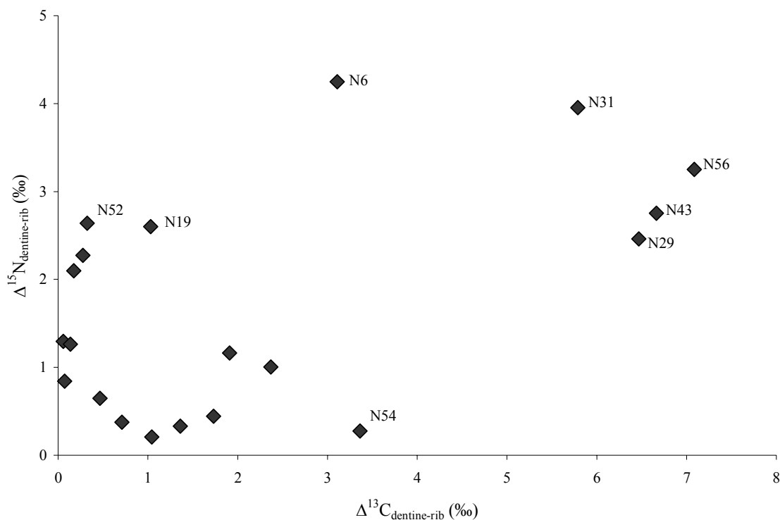
Figure 2: Changing diets: difference between rib and tooth dentine \delta^{13}\text{C} and \delta^{15}\text{N} values for each individual in the study. NB: Labels mark burial numbers.
