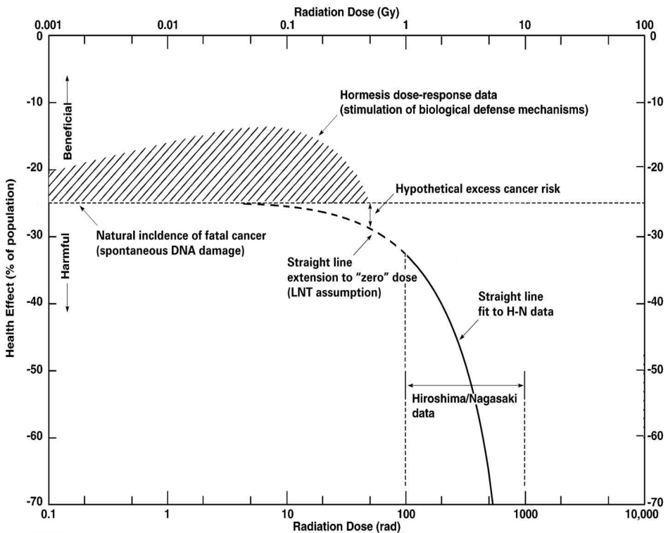
FIGURE 2. Dose-Response for Short-Duration Radiation Exposure (Cutler 1999).
