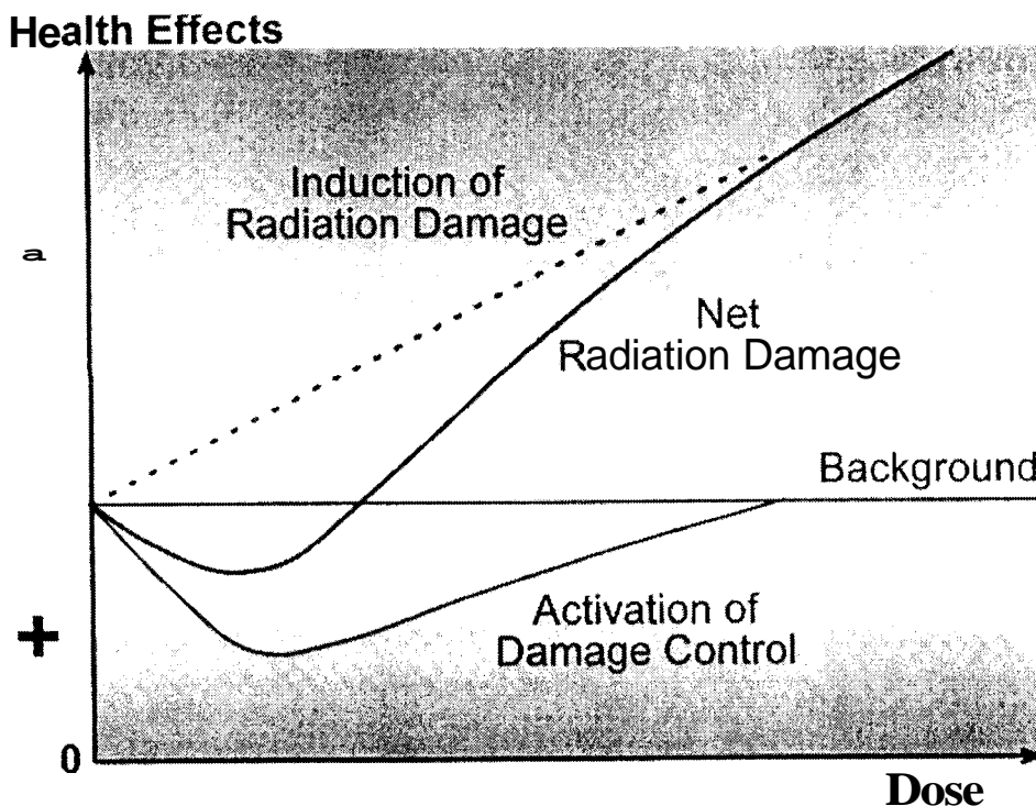
Figure 9. Schematical diagram of the biopositive and bionegative radiation effects as a function of dose, with the damage induction superimposed by the biological defense mechanism, with a de facto threshold generally in the area between 0.2 and 2 Gy (Becker 2002, after Feinendegen).
