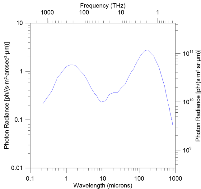
Figure 1. Diffuse CIB background component.
