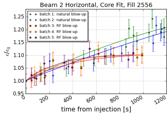
Figure 4: RF batch-by-batch blow-up test with 5 batches of 12 bunches. Batches 1 and 2 are left to natural blow-up. Batches 3, 4 and 5 are longitudinally blown up from a bunch length of 1.1 ns after capture to a target of 1.6 ns. An exponential fit (line) is applied to the relative emittance growth measured with wire scanner (dots). \epsilon_0 is the emittance at injection into the LHC.
