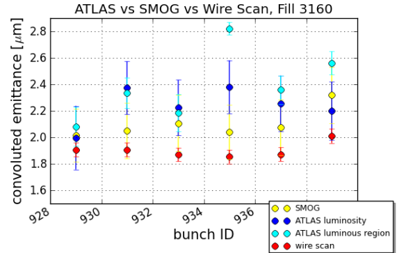
Figure 3: Convoluted emittance per bunch measured with SMOG and wire scanners and calculated from ATLAS luminosity and luminous region for Fill 3160.
