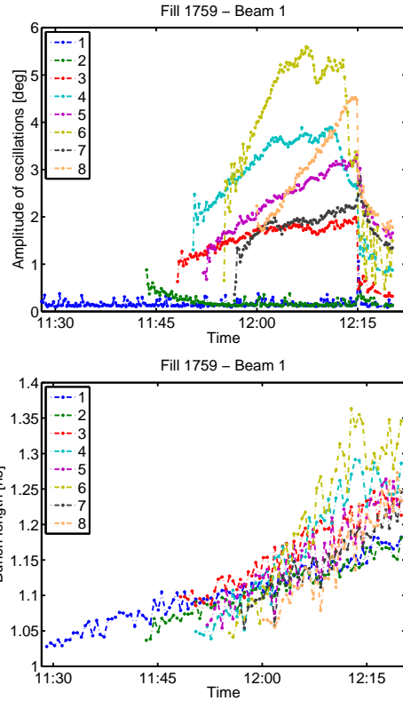
Figure 3: Amplitude of the phase oscillations (top) and bunch length (bottom) with time after injection for 8 bunches of Beam1. Bunch 1 is controlled by the phase loop. Change to the nominal phase loop setting at 12:15.
