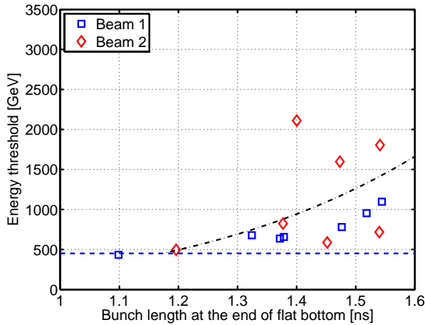
Figure 5: Energy at which the phase oscillations start to grow during the ramp as a function of bunch length at the end of the flat bottom for 8 bunches of Beam1 and Beam2 together with scaling law E_{th} = \tau^4 V^{1/5} (black curve). Each measured point is scaled in energy according to its intensity as N^{4/5} . Average bunch intensity 1.56 \times 10^{11} .
