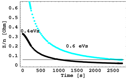
Figure 2: Threshold impedance (1) for loss of Landau damping for bunches with \varepsilon = 0.4 eVs and 0.6 eVs and nominal intensity during the 2010 ramp. The line Z/n = 0.065 Ohm corresponds to the start of instability at 1000 s for \varepsilon = 0.4 eVs and at flat top for \varepsilon = 0.6 eVs.
