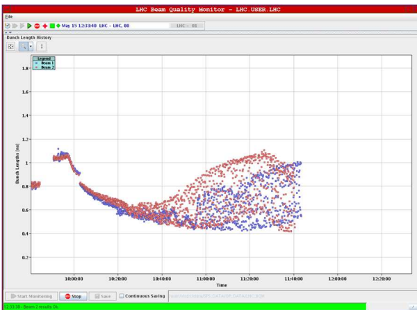
Figure 1: Bunch length of beam 1 (blue) and beam 2 (red) measured by BQM during ramp on 15 May 2010.
