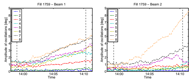
Figure 4: Amplitude of phase oscillations during acceleration cycle for 8 bunches (with different longitudinal emittances) of Beam1 (left) and Beam2 (right). Dashed vertical lines indicate start and end of the ramp.
