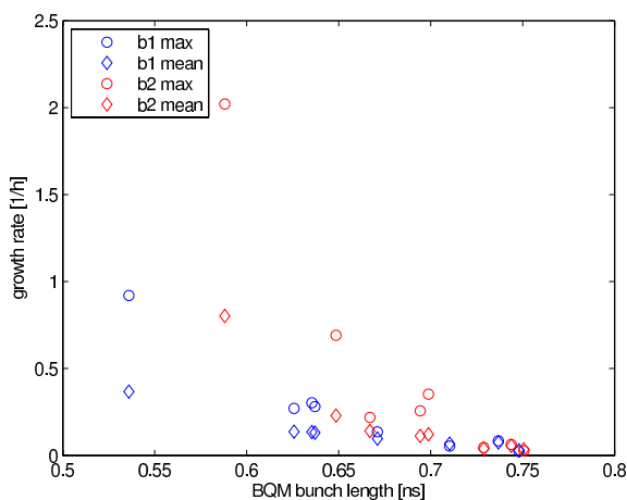
Figure 6: Growth rate of the maximum and mean bunch length during first 25 min of the flat top as a function of initial (flat top) bunch length for 8 bunches of Beam1 and Beam2 (measured by BQM) in 12 MV voltage.
