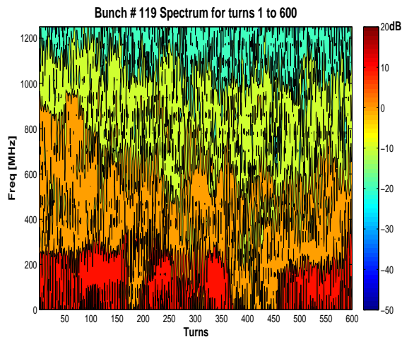
Figure 5: Spectrogram of bunch 119 vertical signal for the transients in Figures 1–3. The unstable bunch shows frequency content up to roughly 1.2 GHz, with most power in the band up to 600 MHz. The complex time structure is related to the 100–200 turn relaxation oscillation.
