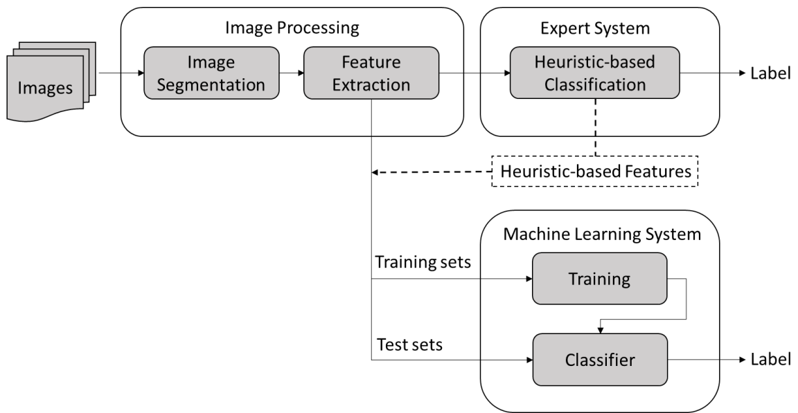
Figure 1. Overview of our element detection pipeline
