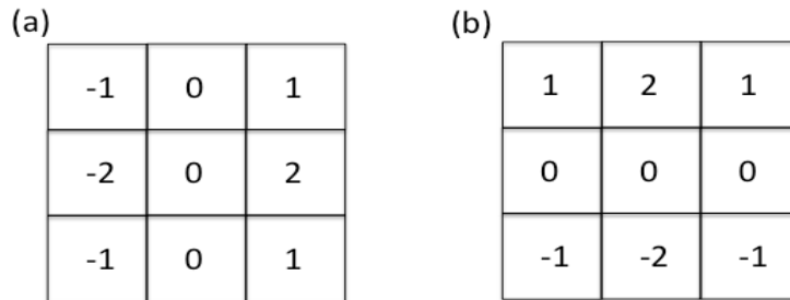
Figure 8. Sobel operators
