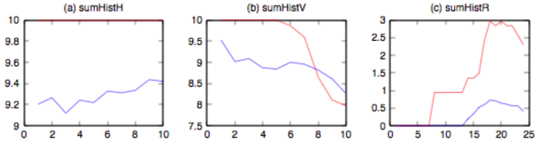
Figure 10. Plot of histograms (H for horizontal, V for vertical and R for radial) averaged over all samples for positives (red) and negatives (blue) - part 1
