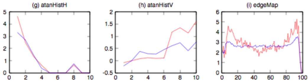
Figure 12. Plot of histograms (H for horizontal, V for vertical and R for radial) averaged over all samples for positives (red) and negatives (blue) - part 3
