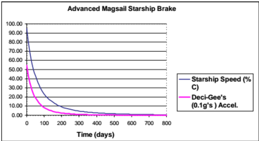
Figure 8. Advanced Magsail deceleration using YBCO Superconductor for a 100km radius magsail. Magnetic Field of B_m = 1.0 \times 10^{-6} T, with a wire density of 7 \times 10^3 kg/m 3 , an engineering current density of 1011 A/m 2 at 77 K, a 1.53 mm thick wire, and a payload ratio of 0.8088.
