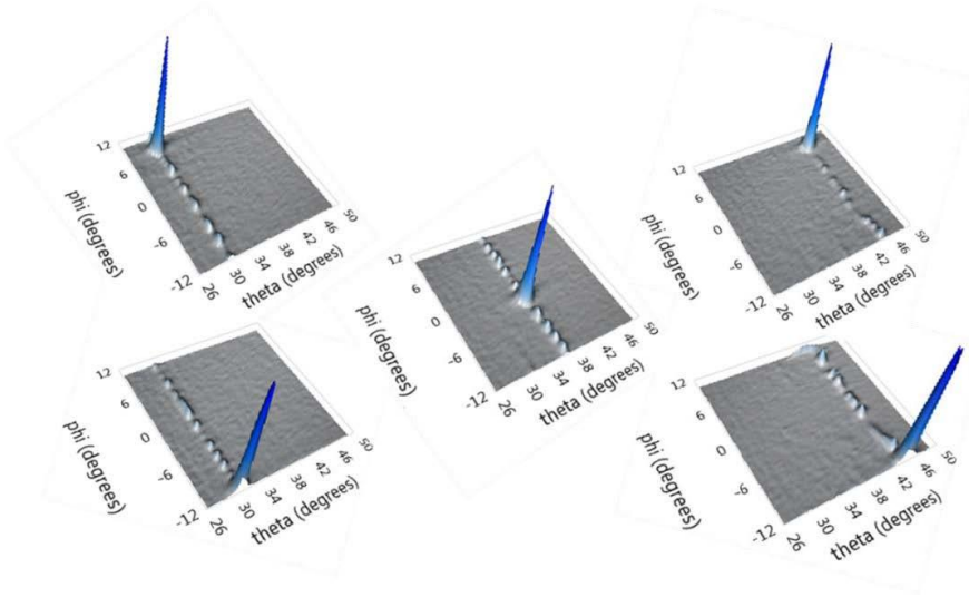
Figure 4. UCSB Phased array for chip level laser communication with no external optics showing electronic beam steering. Hulme et al. , 2014.
