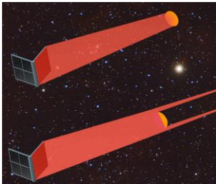
Figure 1. Conceptual drawing showing beam filling sail and then as distance increases eventually overflowing. With Continued illumination speed increases by 2^{1/2} .
