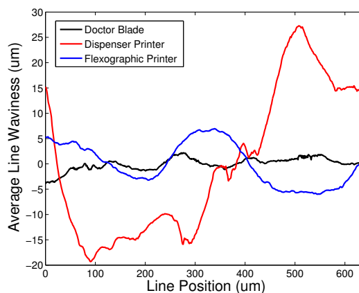
Figure 5. Comparison of resulting cathode average line waviness ( W_a ) with a zero average as produced by doctor blade, dispenser printer, and flexographic printer.
