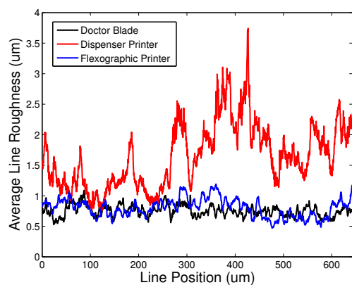
Figure 4. Comparison of resulting cathode average line roughness ( R_a ) as produced by doctor blade, dispenser printer, and flexographic printer.
