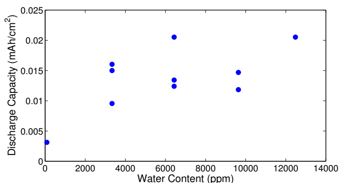
Figure 3. Discharge capacity of coin cells without a gel polymer. Each cell was cycled 100 times.
