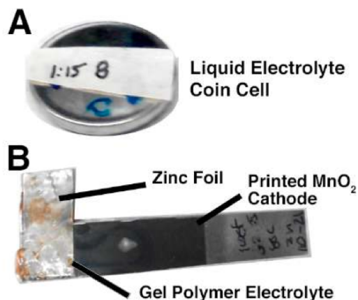
Figure 2. Test cell form factors. A) Coin cell containing liquid electrolyte (no PVDF-HFP gel component); B) Sandwich cell.
