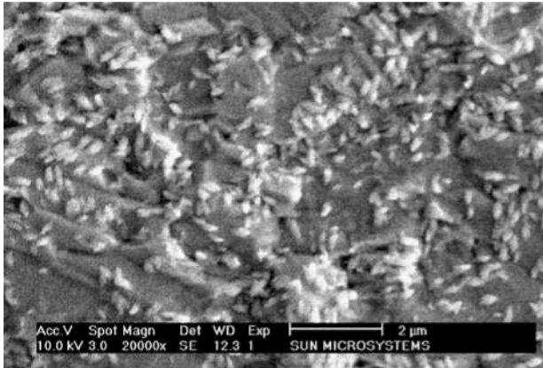
Figure 6 Cross-section of Al 2 O 3 -Cu composite coating produced by EPD-EP sequential deposition.
