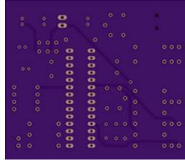
FIGURE 13: EAGLE PCB BACK
