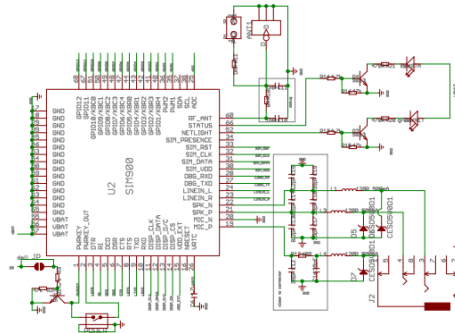
FIGURE 19: SEED STUDIO GPRS SHIELD SCHEMATIC PART 1
