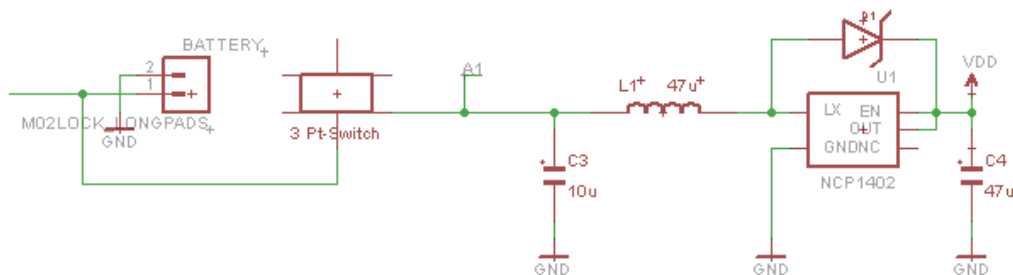
FIGURE 10: EAGLE PCB 5V STEP-UP CONVERTER SCHEMATIC
