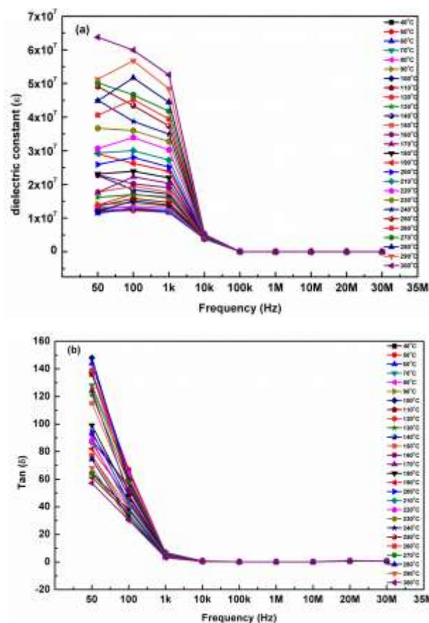
Fig. 4 – Dielectric Constant (a) and Dielectric Loss (b) of G-sheets as function of temperature
