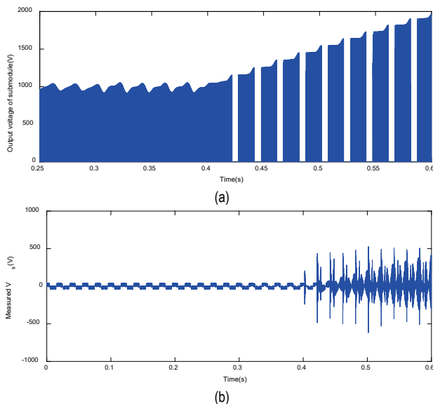
Figure 13 Output voltage of the fault SM: (a) Output Voltage of SM2; (b) Output voltage after bandpass filtering
