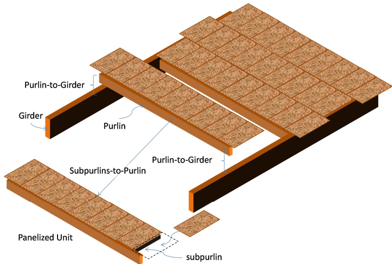
Figure 1: Panelized roof construction.
