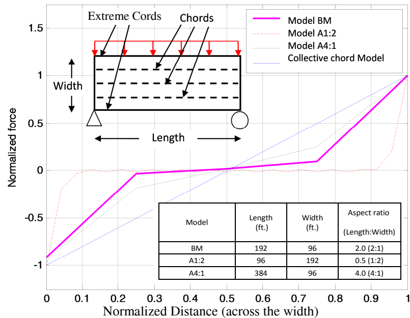
Figure 11. Distribution of chord forces for diaphragms of different aspect ratios.
