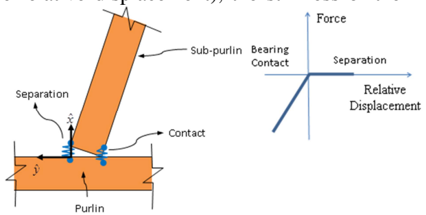
Figure 8. Subpurlin-to-purlin contact model.
