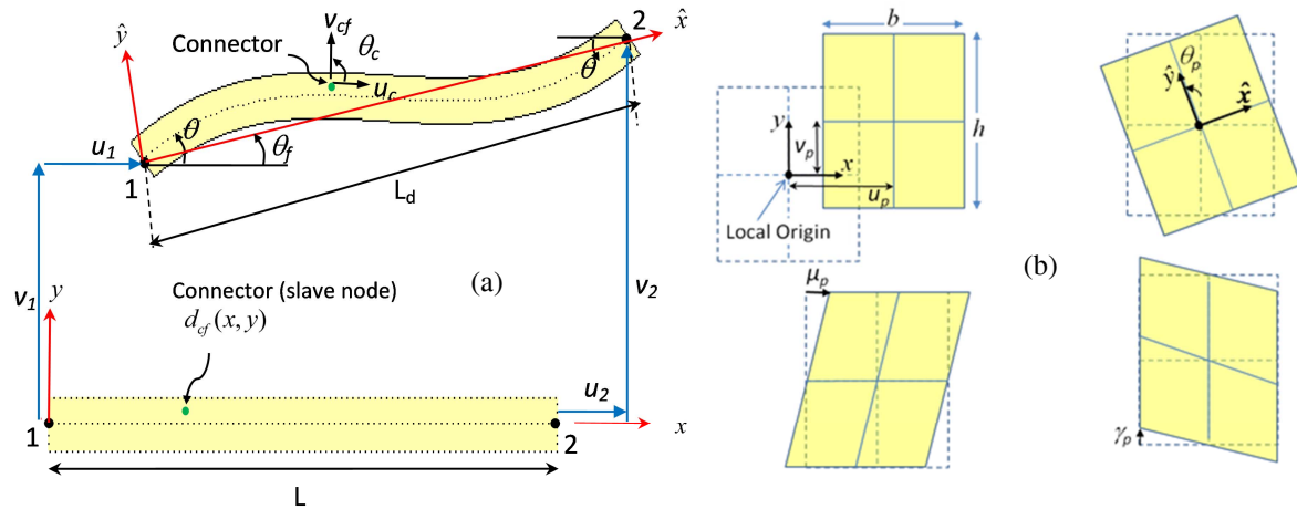
Figure 4. Kinematics of (a) frame element and (b) panel element.
