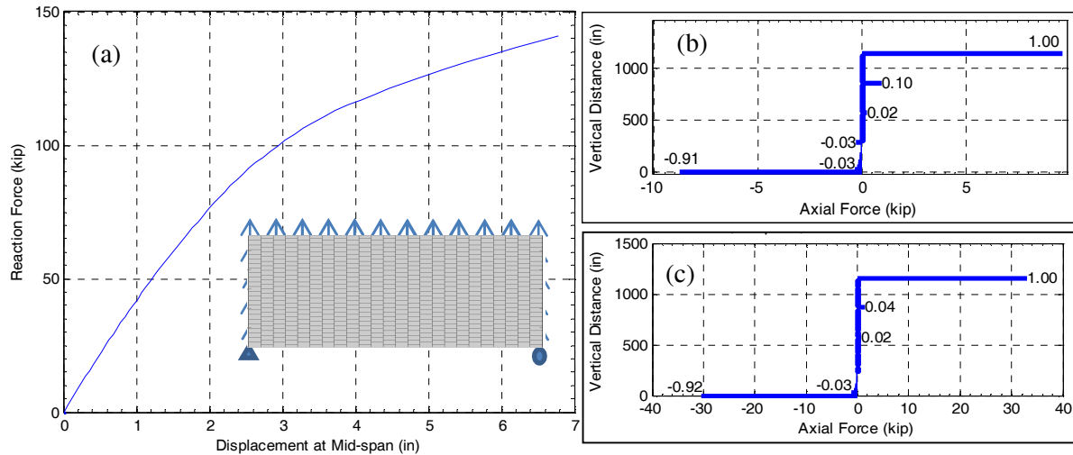
Figure 10. (a) Lateral pushover curve of benchmark diaphragm model (BM); chord force distributions at mid-span when pushover displacement is (b) 1 in. and (c) 6.8 in.
