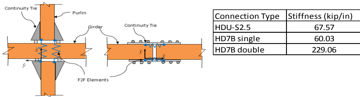
Figure 7. Connection models for purlin-to-purlin ties (left) and girder-to-girder ties (right).
