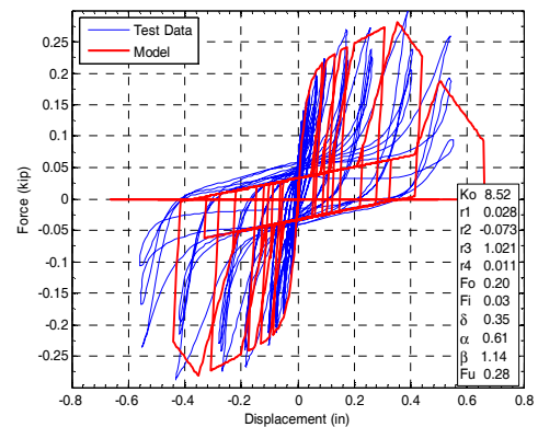
Figure 5. Hysteretic model for sheathing nail.
