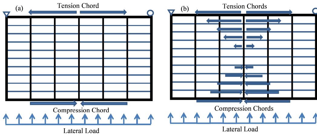
Figure 2. Chord force distribution; (a) traditional diaphragm design method, and (b) collective chord method.
