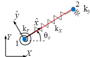
Figure 6. Connector element.
