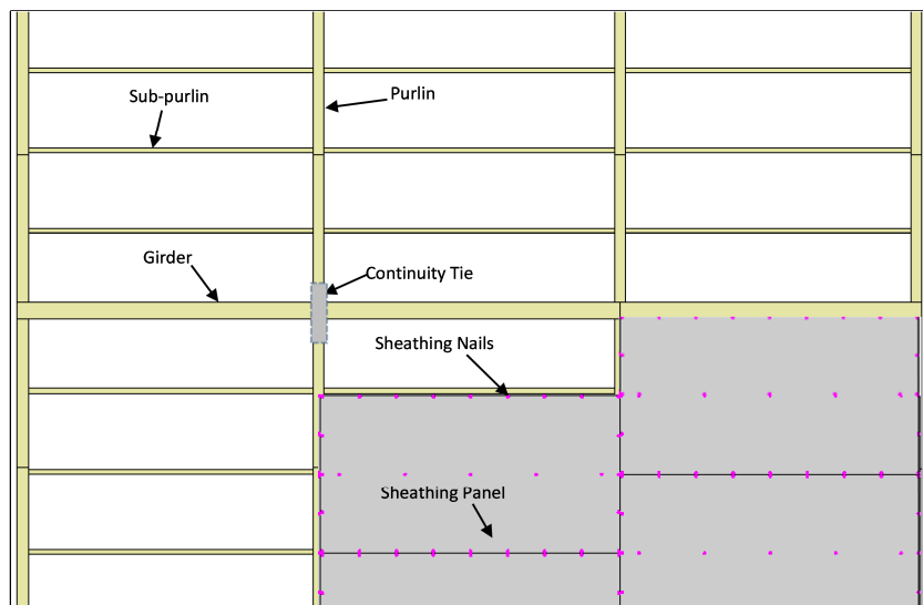
Figure 3. An example assembly of a panelized roof diaphragm.
