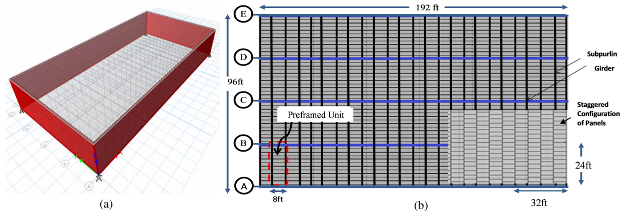
Figure 9. (a) A case study building model, and (b) panelized roof diaphragm model.
