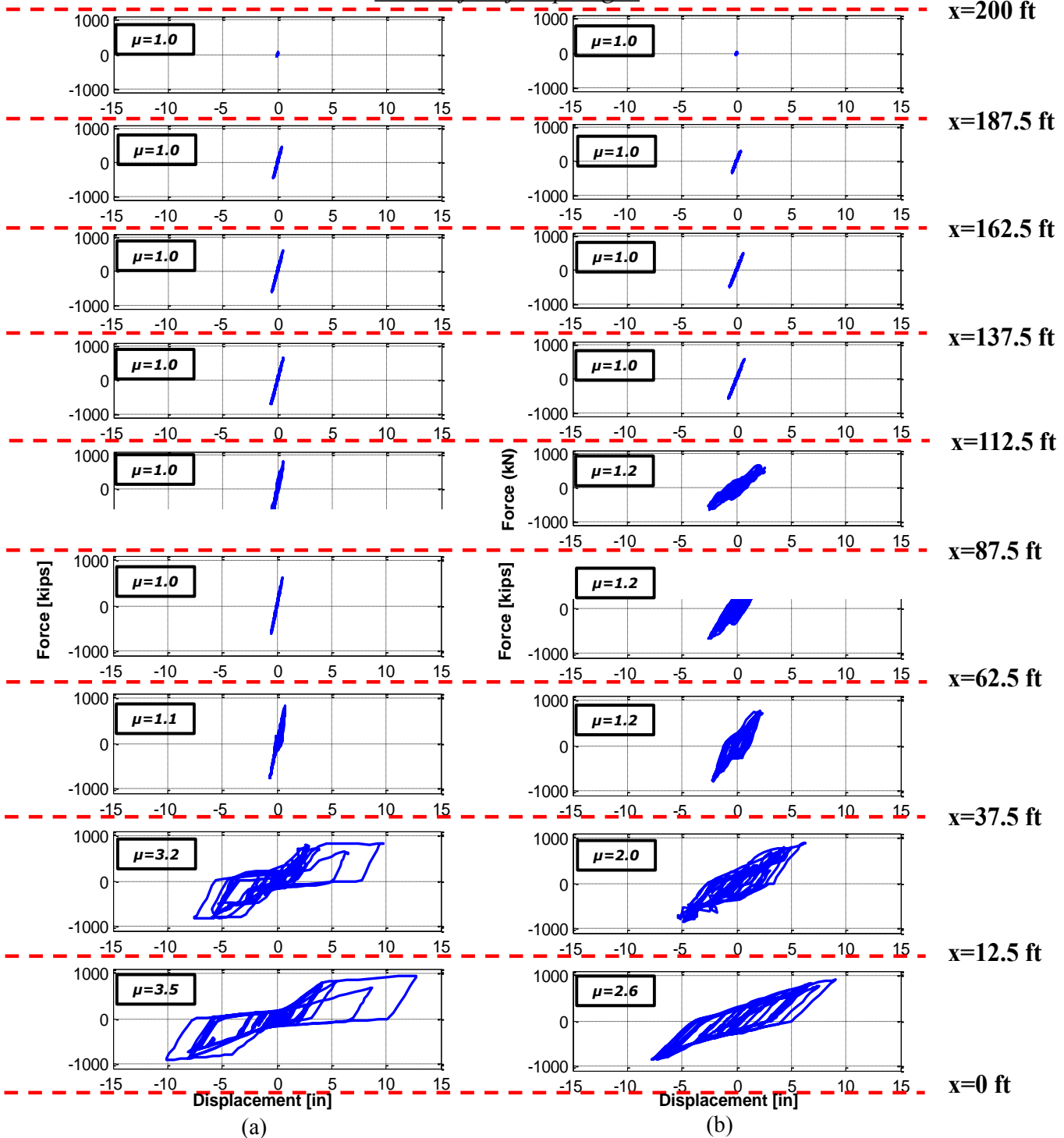
Figure 3. Hysteretic diaphragm response case study for Friuli, Italy (1976) Record at MCE intensity – excitation parallel to diaphragm short direction: (a) conventional (ASCE 7-10) diaphragm design and (b) weakened diaphragm interior design [Koliou, 2014].
