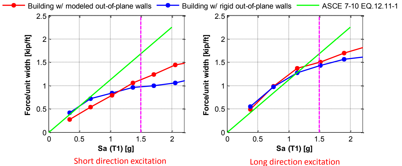
Figure 5. Wall anchorage forces at diaphragm mid-span associated with Performance Group 1 [Table 1]. Walls are 9/4-inch thick concrete, 30-feet high to roof with 3-foot parapet. The building dimensions are 200-ft (short direction) by 400-ft (long direction).
