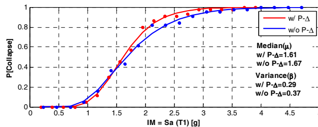
Figure 5. Influence of P- \Delta effects on the collapse capacity of the RWFD building archetype.
