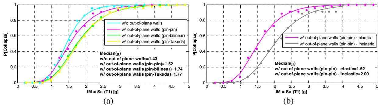
Figure 7. Influence of: (a) out-of-plane wall panels' base fixity conditions and (b) the inelastic response of the out-of-plane wall panels on the collapse capacity of the RWFD building archetype.
