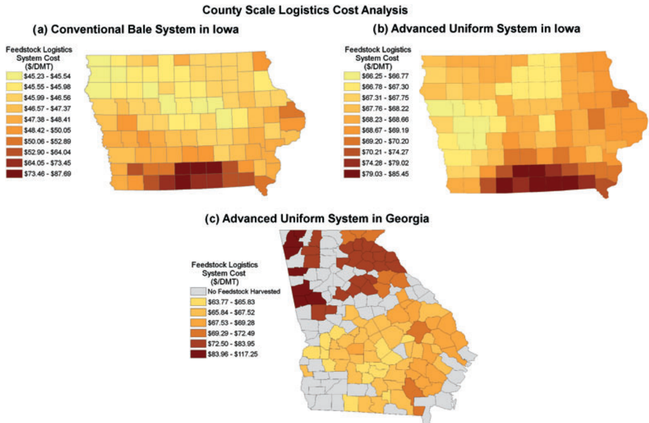
Figure 3. Breakdown of total Case 1 and 2 logistics costs for each county in Iowa based on removable stover limits, and total Case 3 logistics costs for each county in Georgia based on removable switchgrass limits.
