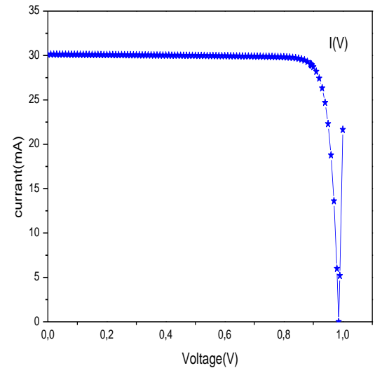
Fig. 6 – Current-voltage characteristics of solar cell optimized
