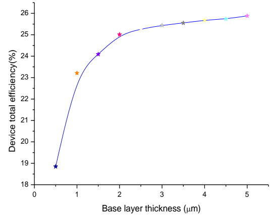
Fig. 5 – Device total efficiency variation depending on the thickness the base layer
