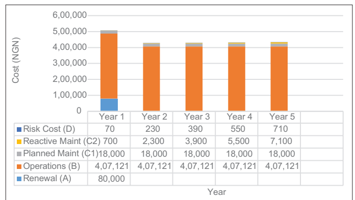
Figure 1: Annual cost model of 3.3 kVA gasoline generator
