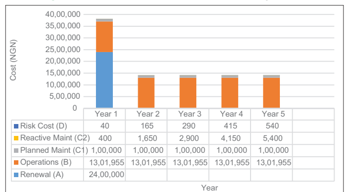
Figure 2: Annual cost model of 20 kVA diesel generator
