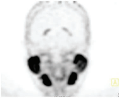
Figure 6. ^{18}\text{F} -choline positron emission tomography (PET) image (coronal view) with ^{18}\text{F} -choline avid parotids and submandibular gland.
