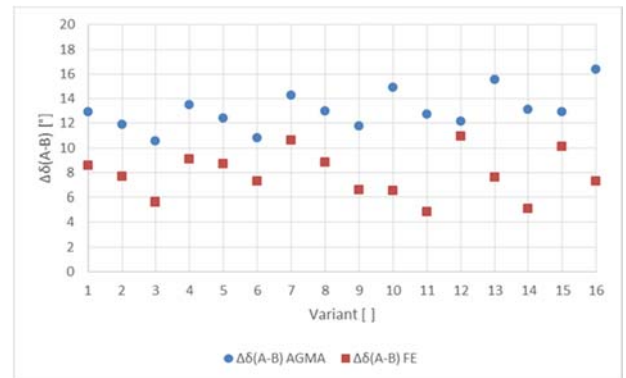
Fig.7 Move of dangerous cross-section of symmetric pairs.
