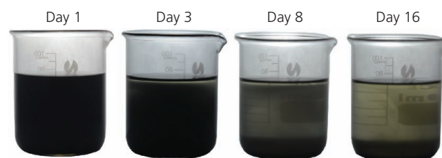
Figure 1. Sedimentation of copper (II) oxide/PKO nanolubricant over a period of time
