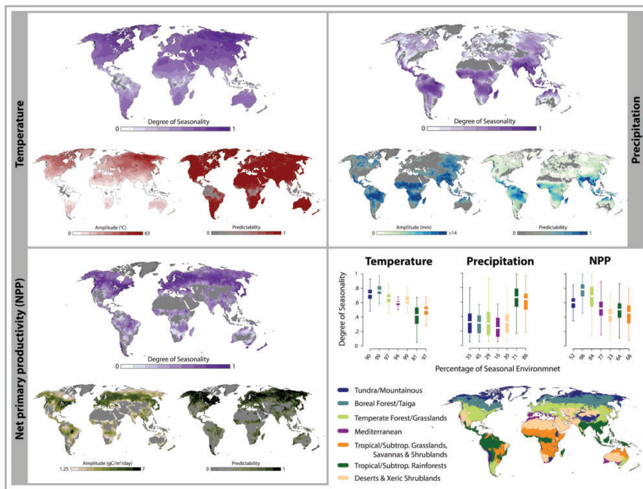
Fig. 2 Degree of seasonality in terrestrial ecosystems (purple) with its two major components, the amplitude and predictability for temperature (top left), precipitation (top right) and NPP (bottom left). All maps have a spatial resolution of 111 \times 111 km. Areas without significant seasonal dynamics are indicated in gray. The bottom right panel shows the median and the 50 percentile (box) and the 95 percentiles (outer bars) of the degree of seasonality for all factors (e.g., temperature, precipitation, and primary productivity) across major terrestrial ecoregions. The x-axes indicate the relative amount (in percentage) of area that exhibits seasonal variation within each ecoregion
